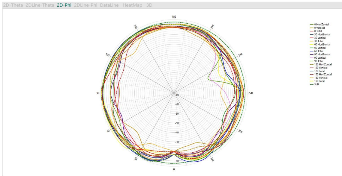
2440MHz 3D-Horizontal Pattern
