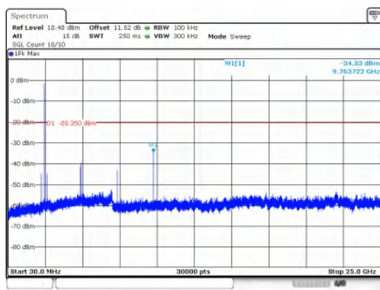
GFSK_DH5_Channel 39
