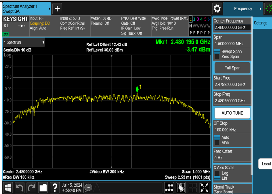
2DH5-Ant1-2480-0~Reference-PASS
