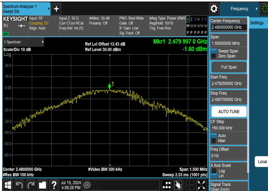
DH5-Ant1-2480-0~Reference-PASS
