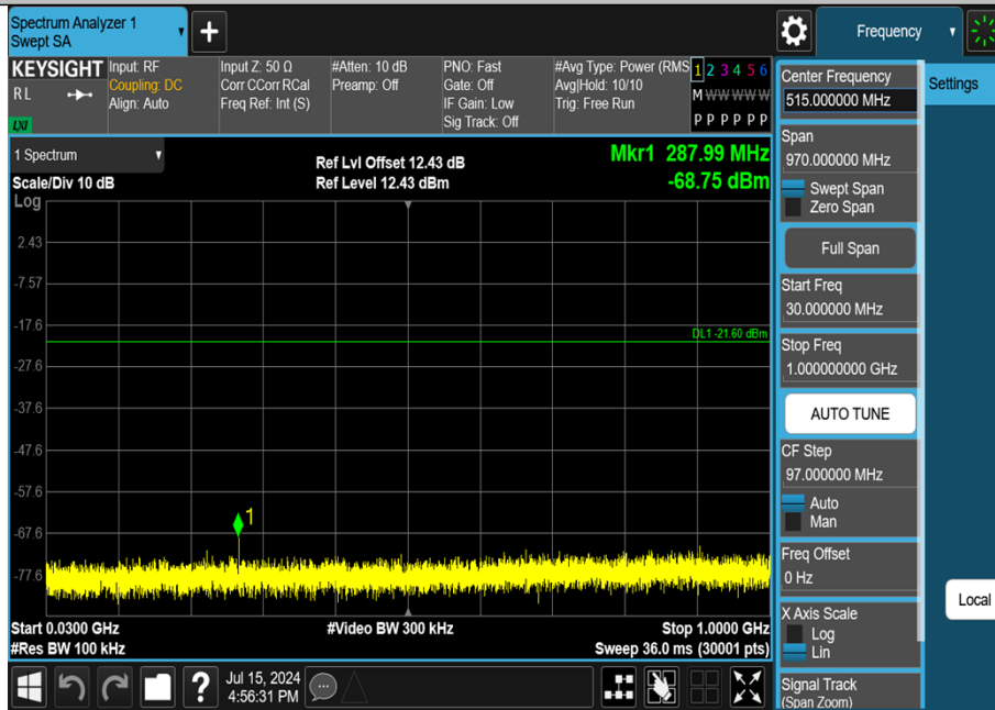
DH5-Ant1-2480-30~1000-PASS
