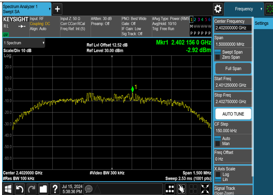
3DH5-Ant1-2402-0~Reference-PASS
