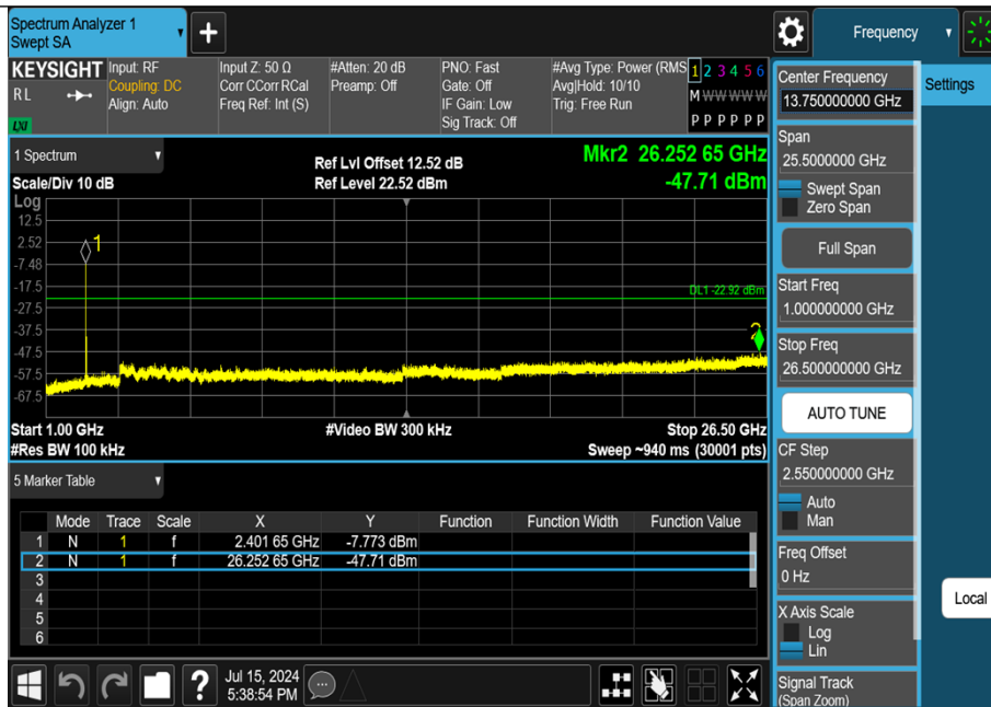
3DH5-Ant1-2402-1000~26500-PASS
