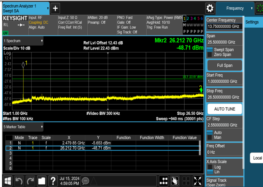
2DH5-Ant1-2480-1000~26500-PASS
