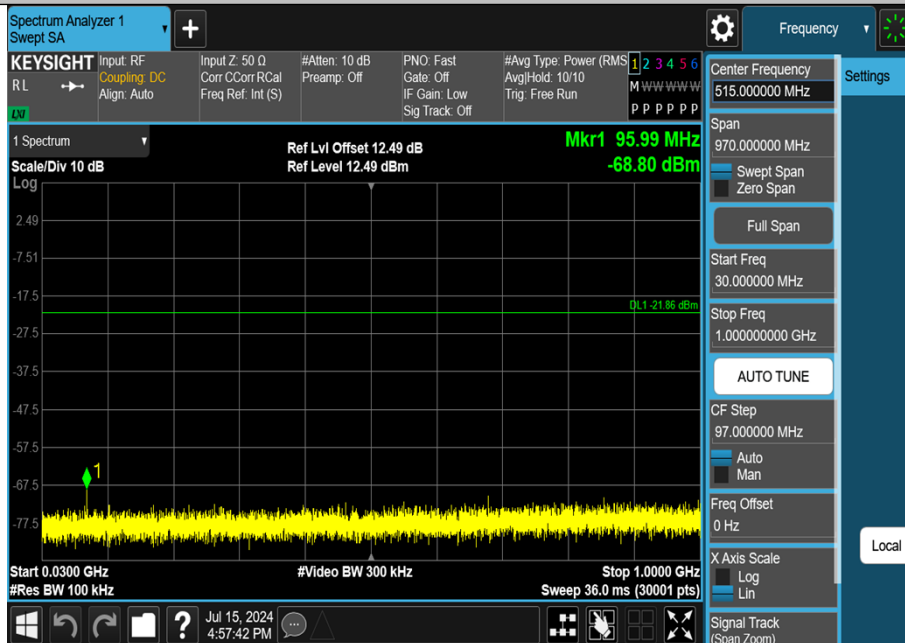
2DH5-Ant1-2441-30~1000-PASS
