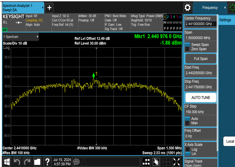
2DH5-Ant1-2441-0~Reference-PASS
