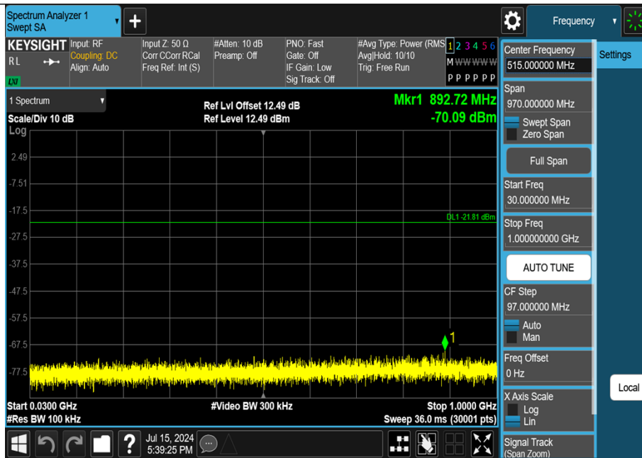
3DH5-Ant1-2441-30~1000-PASS
