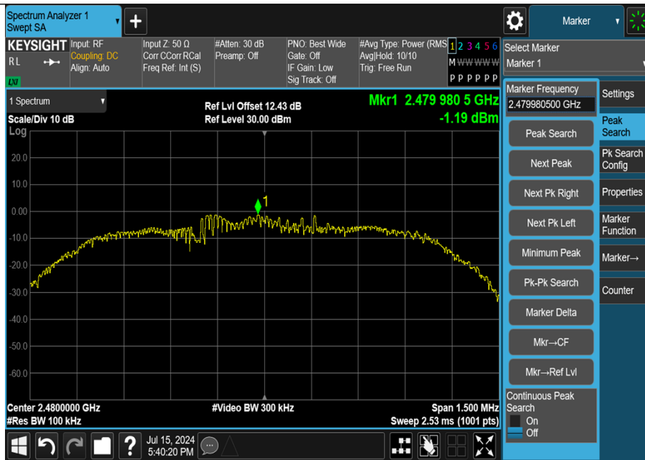
3DH5-Ant1-2480-0~Reference-PASS
