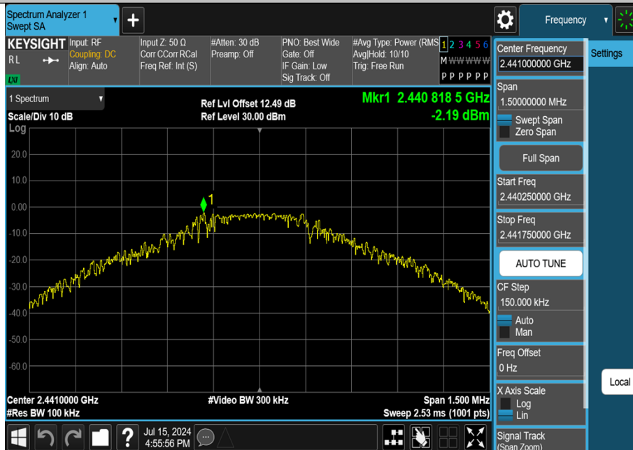
DH5-Ant1-2441-0~Reference-PASS
