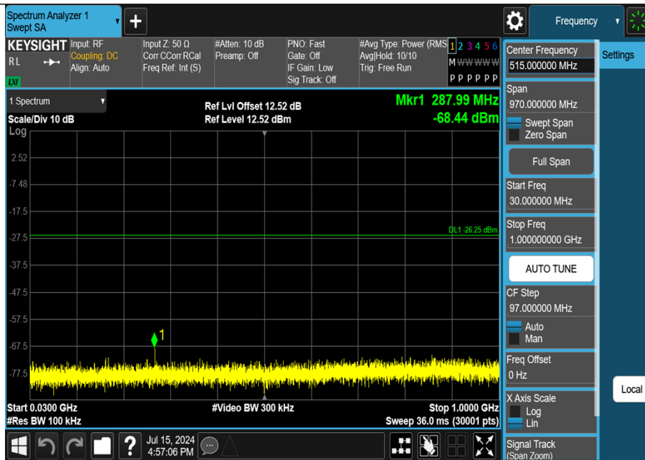
2DH5-Ant1-2402-30~1000-PASS
