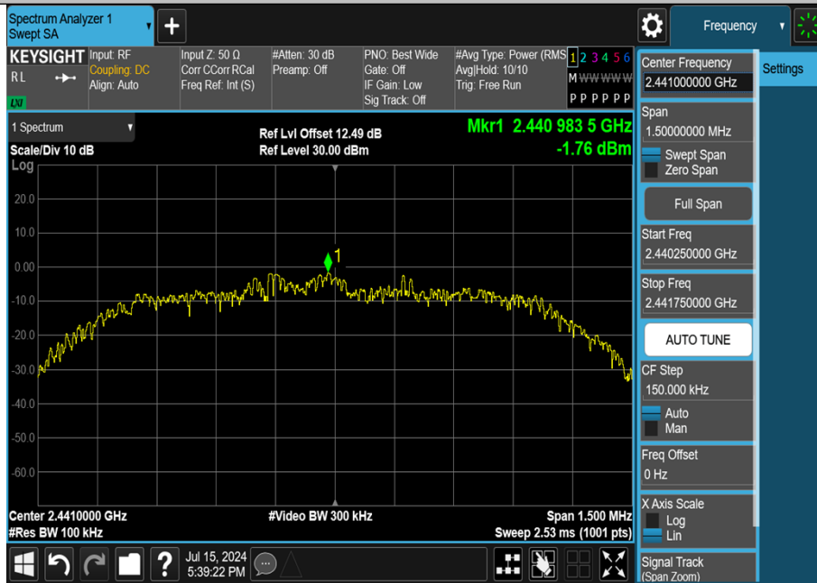
3DH5-Ant1-2441-0~Reference-PASS
