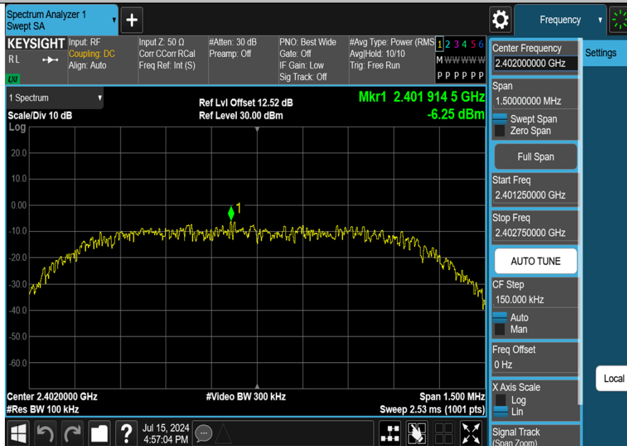
2DH5-Ant1-2402-0~Reference-PASS
