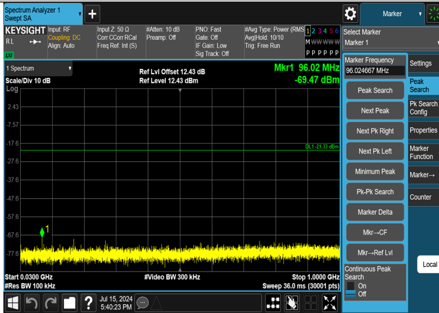
3DH5-Ant1-2480-30~1000-PASS
