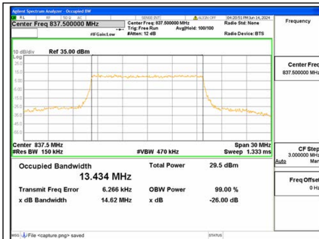
B19 / 15MHz / QPSK/ High CH
