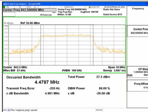
B19 / 5MHz / 64QAM/ High CH
