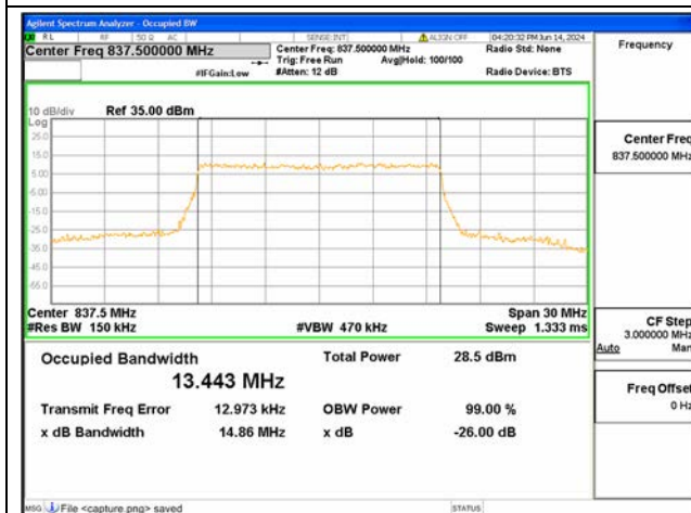
B19 / 15MHz / 16QAM/ Mid CH
