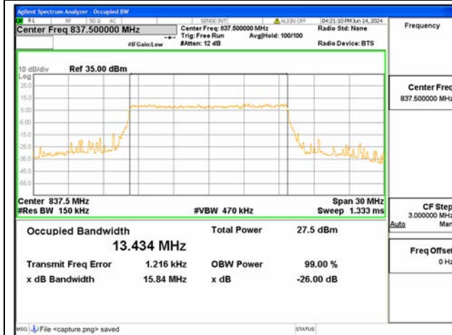
B19 / 15MHz / 64QAM/ High CH
