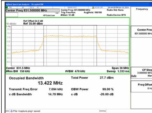
B26 Part22 / 15MHz / 64QAM/ Low CH
