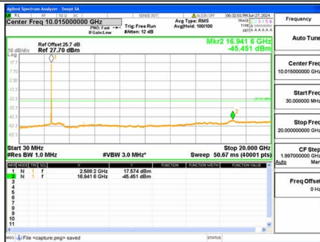
B41(2535-2655)-30M-20G / 15MHz / Mid CH / QPSK
