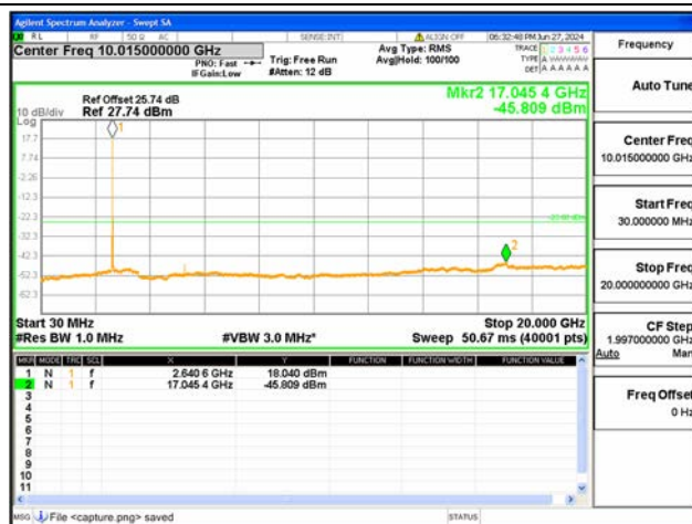
B41(2535-2655)-30M-20G / 15MHz / High CH / QPSK
