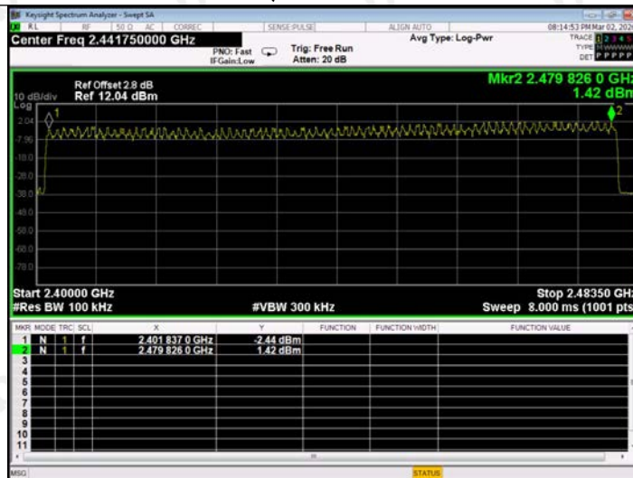
8-DPSK Modulation
