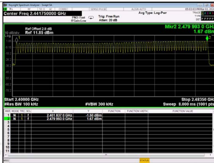
GFSK Modulation
