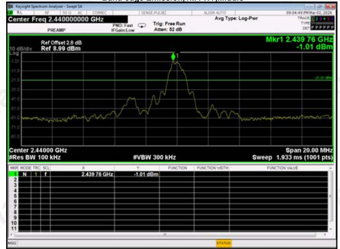
Band edge Emission,1M PHY,Middle
