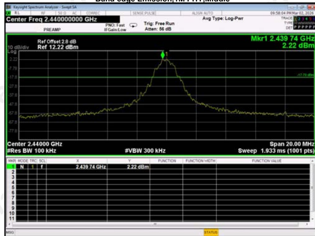
Band edge Emission,1M_PHY,Middle
