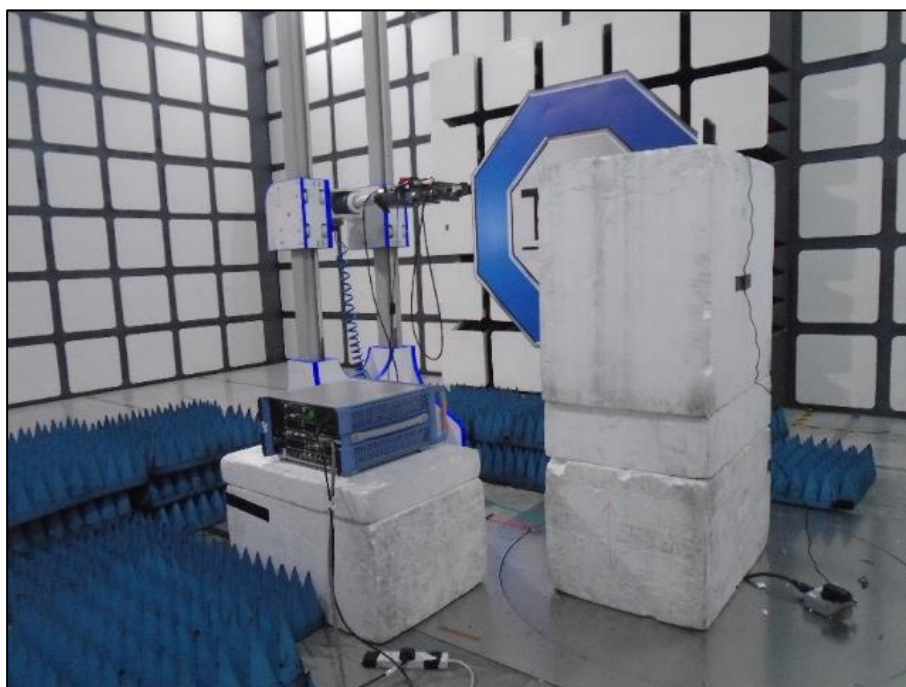
Figure 9 - Test Setup - 18 GHz to 20 GHz
