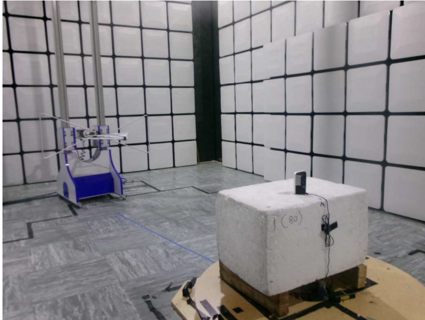
Figure 20 - 30 MHz to 1 GHz
