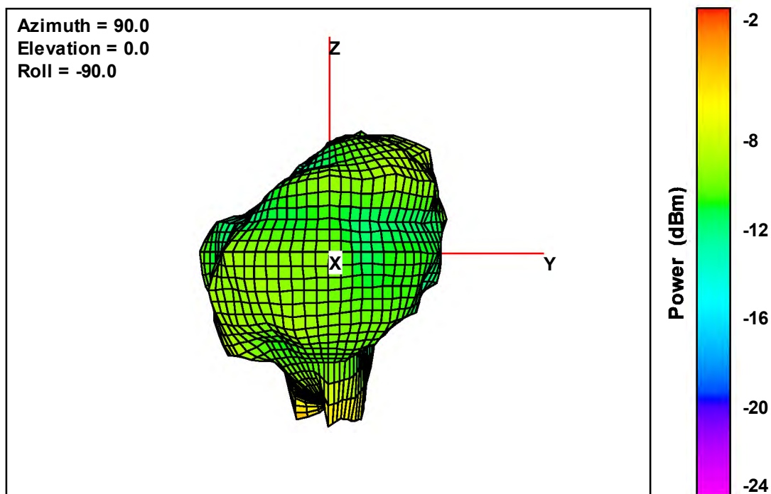
Free-Space Total EIRP, Front Face View, 928 MHz
