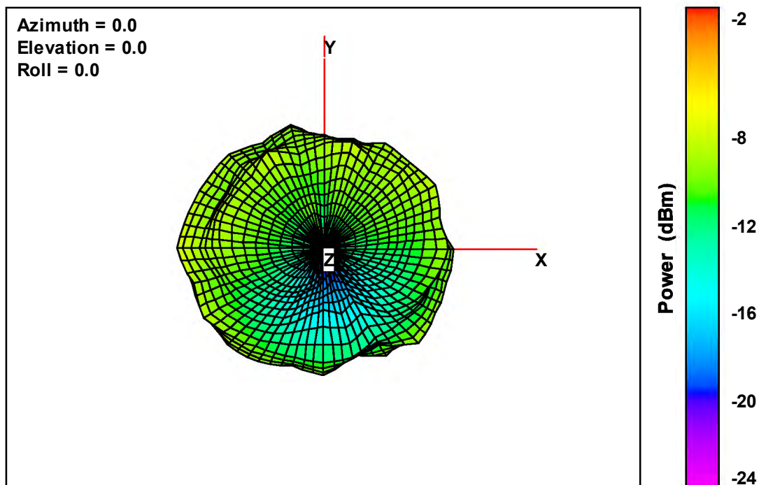
Free-Space Total EIRP, Top View, 928 MHz
