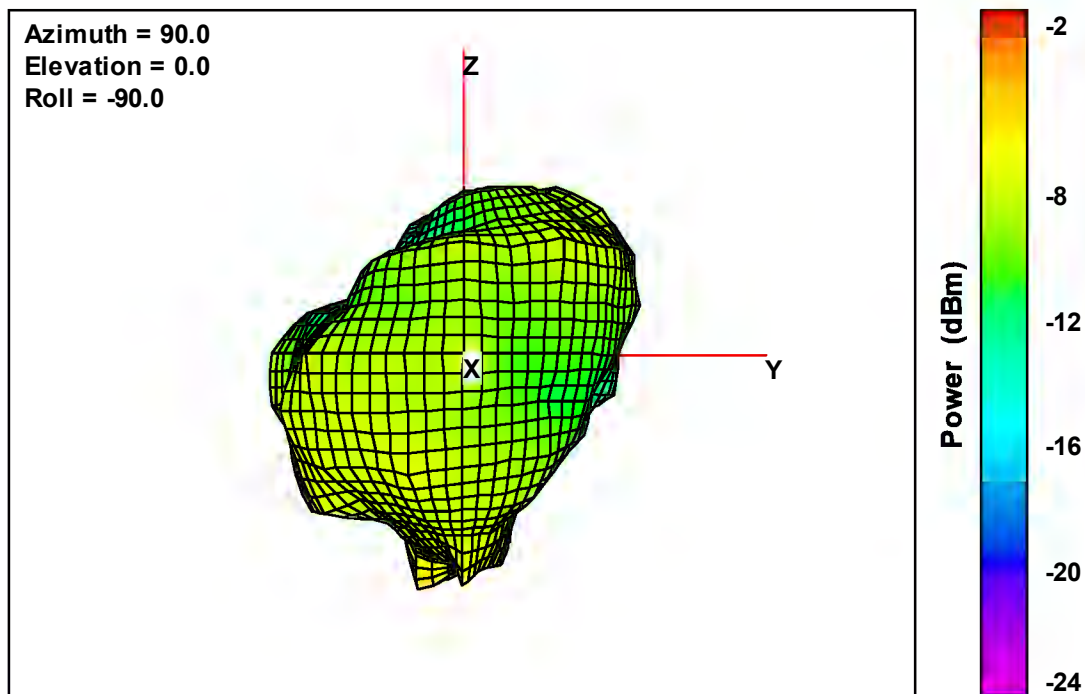
Free-Space Total EIRP, Front Face View, 915 MHz
