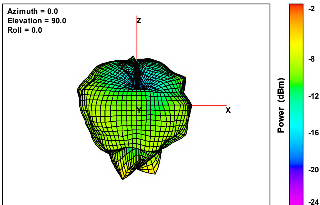
Free-Space Total EIRP, Left Side View, 928 MHz
