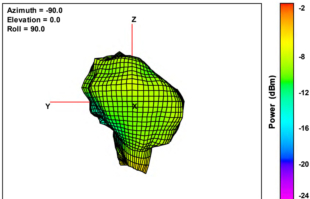
Free-Space Total EIRP, Back Face View, 928 MHz
