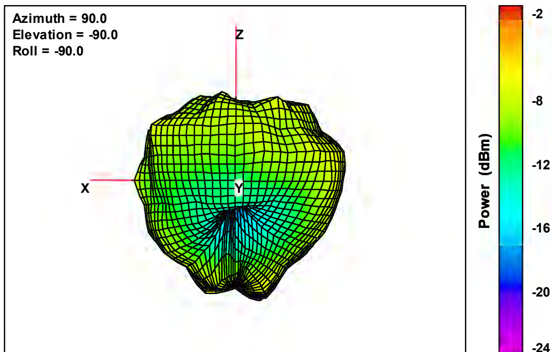
Free-Space Total EIRP, Right Side View, 915 MHz
