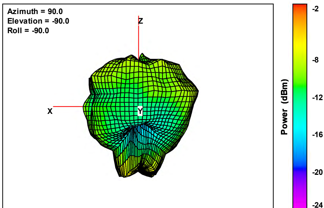
Free-Space Total EIRP, Right Side View, 928 MHz
