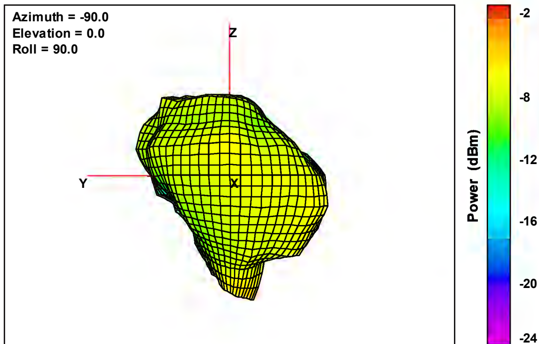
Free-Space Total EIRP, Back Face View, 915 MHz
