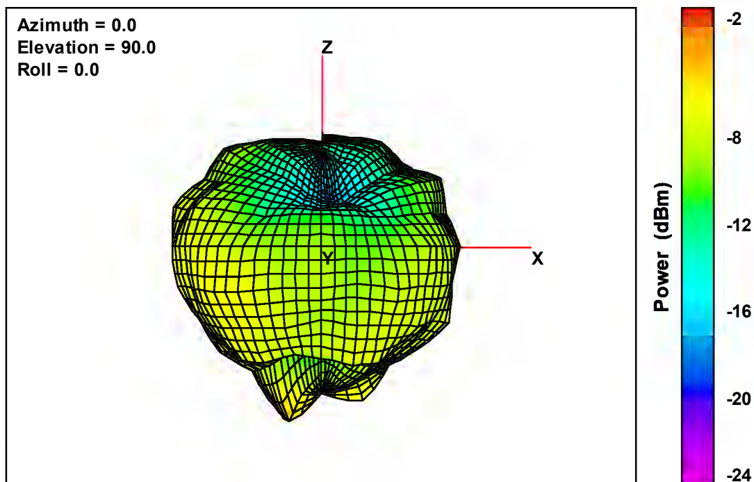
Free-Space Total EIRP, Left Side View, 915 MHz
