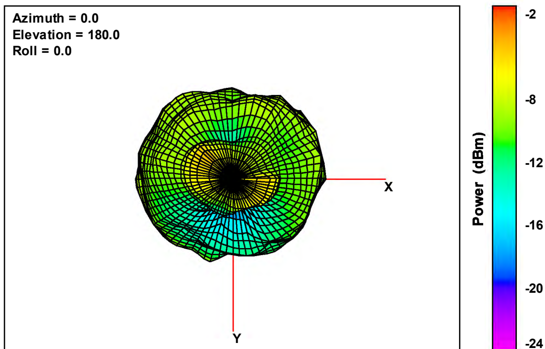
Free-Space Total EIRP, Bottom View, 928 MHz
