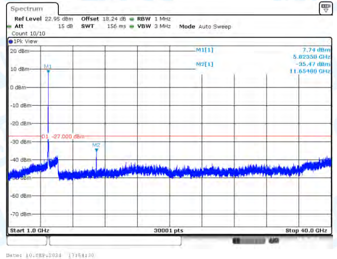
11N20SISO-Ant1-5825-1000~40000-PASS
