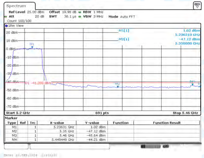
11AX40SISO-Ant1-5230-PASS
