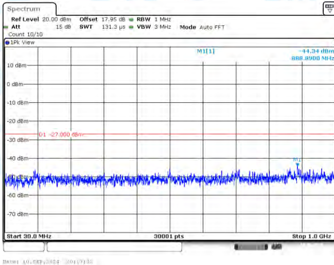
11AC20SISO-Ant1-5180-30~1000-PASS
