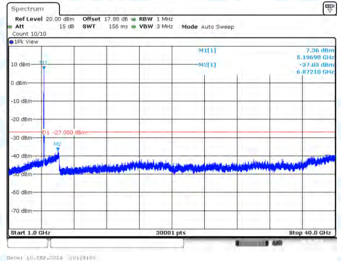
11AC40SISO-Ant1-5190-1000~40000-PASS
