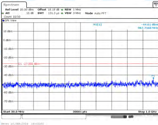
11AC20SISO-Ant1-5785-30~1000-PASS
