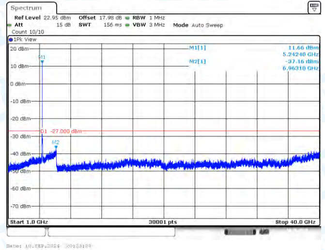
11AC20SISO-Ant1-5240-1000~40000-PASS
