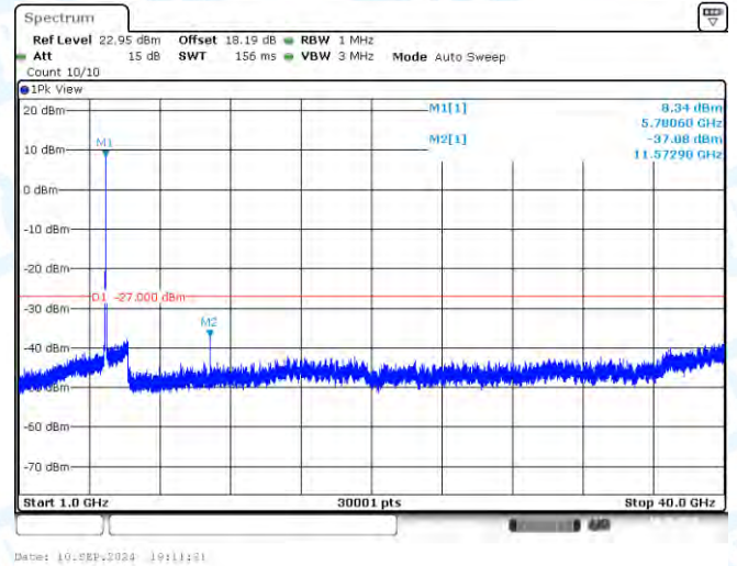
11AX20SISO-Ant1-5785-1000~40000-PASS
