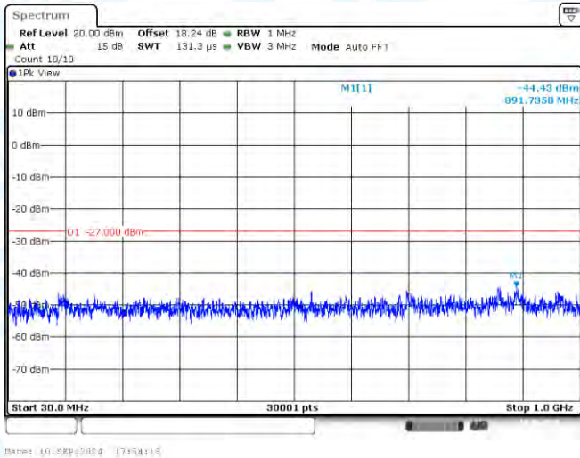
11N20SISO-Ant1-5825-30~1000-PASS
