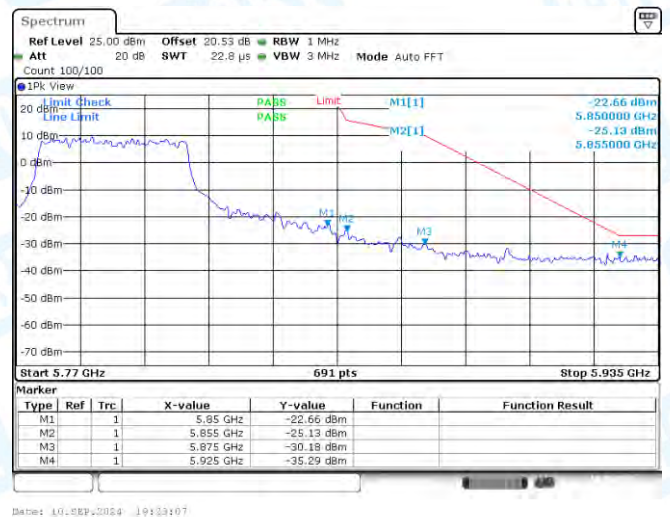
11AX40SISO-Ant1-5795-PASS
