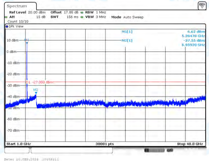
11AX40SISO-Ant1-5190-1000~40000-PASS
