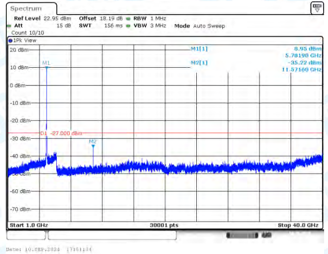
11N20SISO-Ant1-5785-1000~40000-PASS
