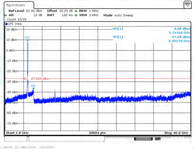
11AX40SISO-Ant1-5755-1000~40000-PASS
