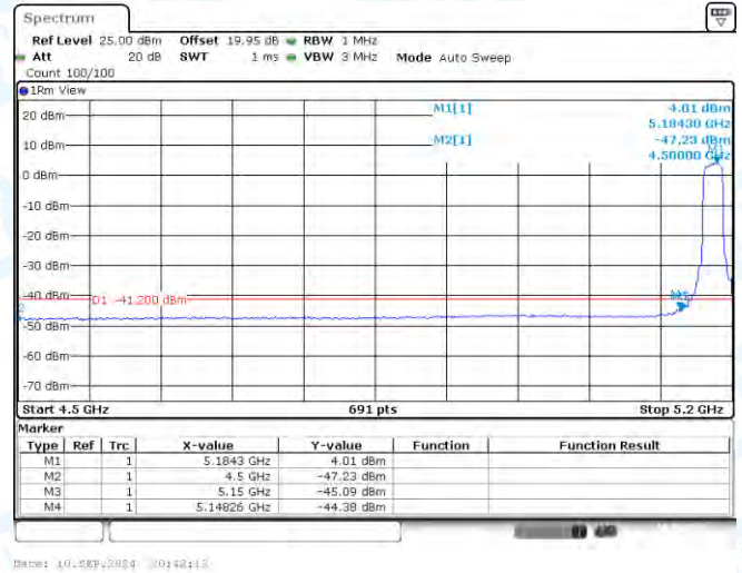
11AX20SISO-Ant1-5180-PASS
