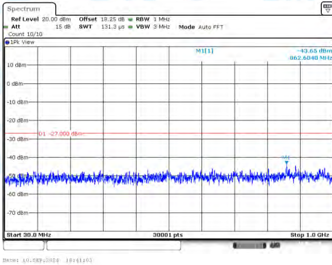
11AC20SISO-Ant1-5745-30~1000-PASS
