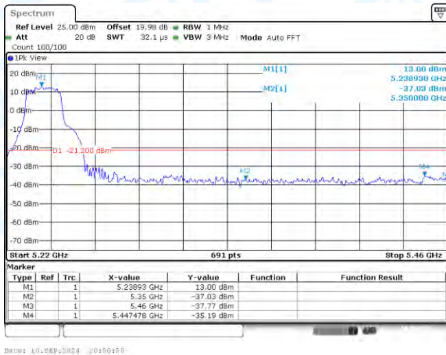
11AX20SISO-Ant1-5240-PASS
