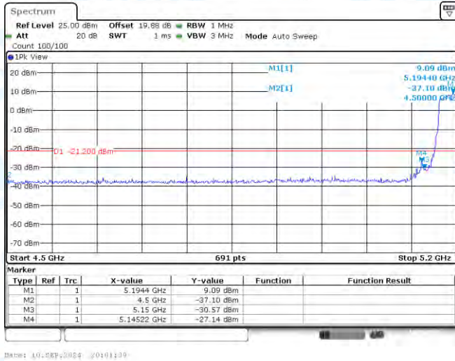
11N40SISO-Ant1-5190-PASS
