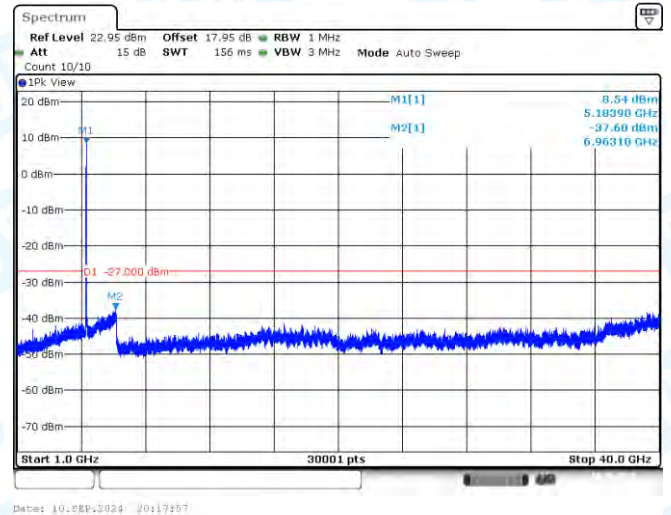
11AC20SISO-Ant1-5180-1000~40000-PASS
