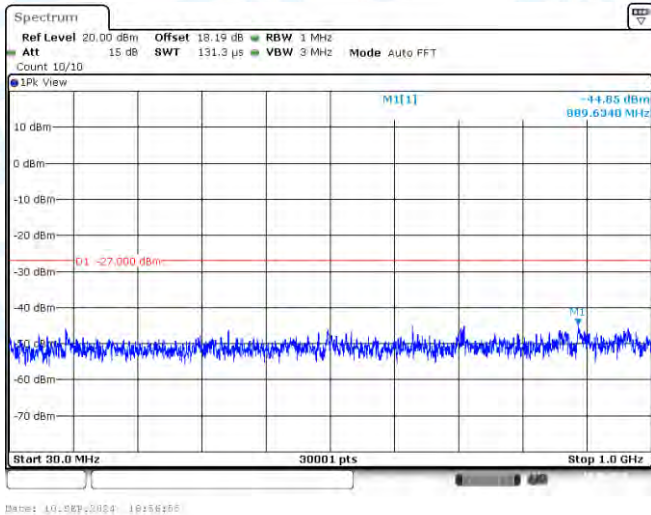
11AC40SISO-Ant1-5795-30~1000-PASS
