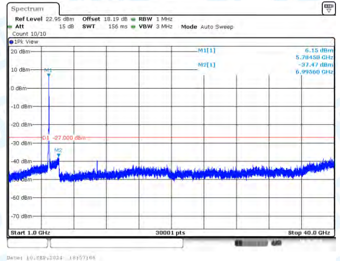
11AC40SISO-Ant1-5795-1000~40000-PASS
