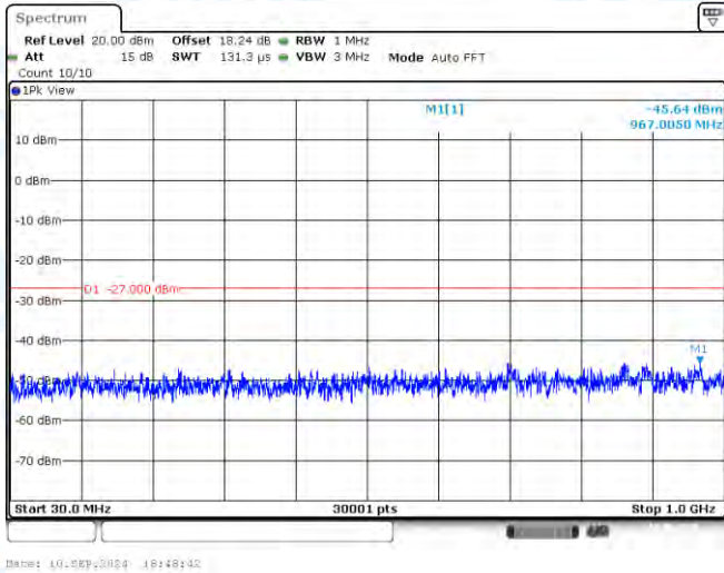
11AC20SISO-Ant1-5825-30~1000-PASS
