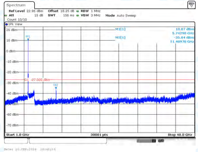
11AC20SISO-Ant1-5745-1000~40000-PASS
