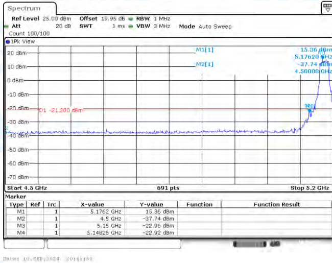
11AX20SISO-Ant1-5180-PASS
