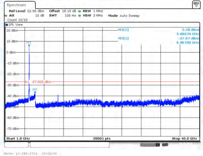
11N40SISO-Ant1-5795-1000~40000-PASS
