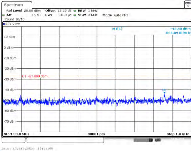
11AX20SISO-Ant1-5785-30~1000-PASS
