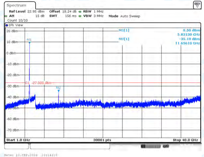
11AX20SISO-Ant1-5825-1000~40000-PASS
