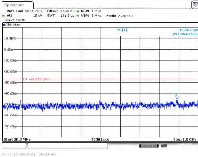
11AC20SISO-Ant1-5240-30~1000-PASS
