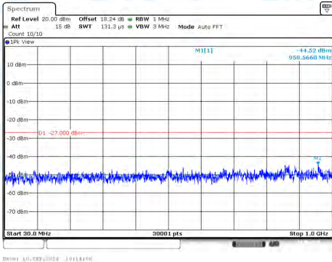
11AX20SISO-Ant1-5825-30~1000-PASS
