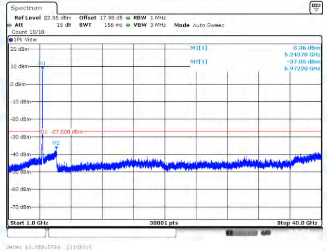
11AX40SISO-Ant1-5230-1000~40000-PASS
