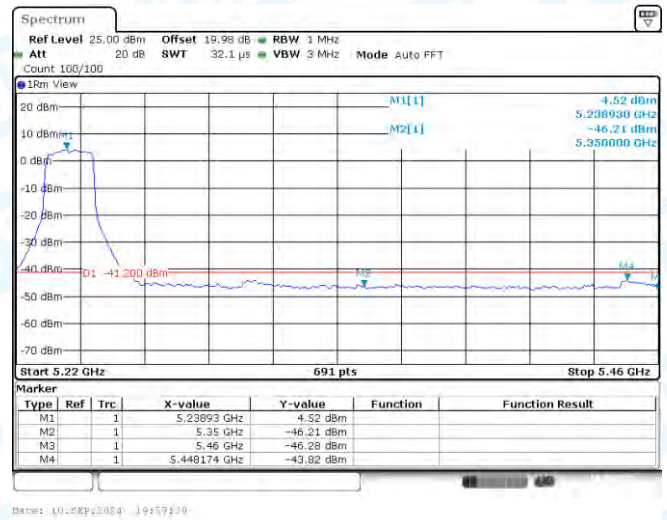
11N20SISO-Ant1-5240-PASS
