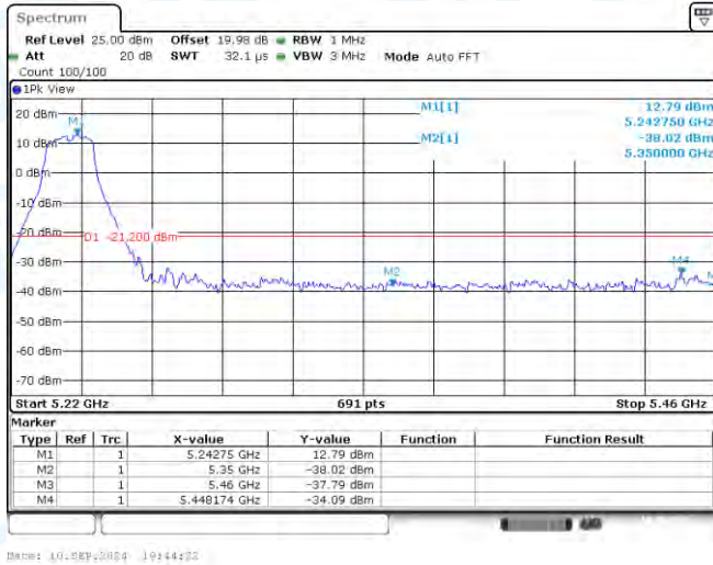
11A-Ant1-5240-PASS
