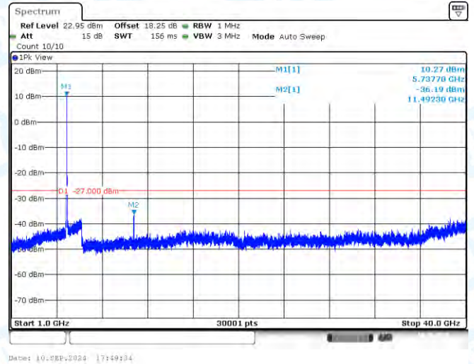
11N20SISO-Ant1-5745-1000~40000-PASS
