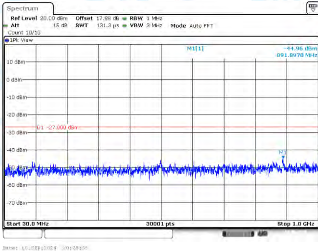
11AC40SISO-Ant1-5190-30~1000-PASS
