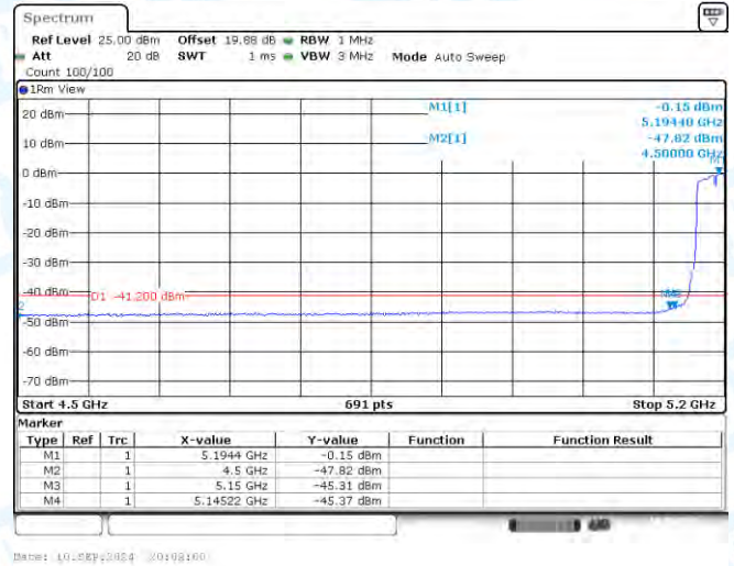
11N40SISO-Ant1-5190-PASS
