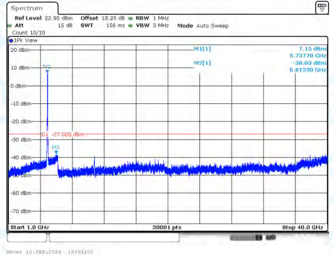
11AC40SISO-Ant1-5755-1000~40000-PASS
