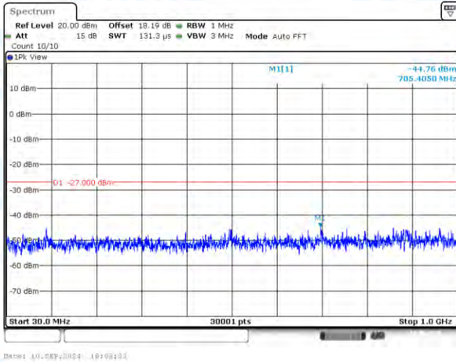
11N40SISO-Ant1-5795-30~1000-PASS
