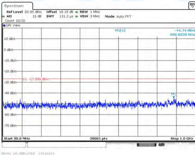
11AX40SISO-Ant1-5795-30~1000-PASS
