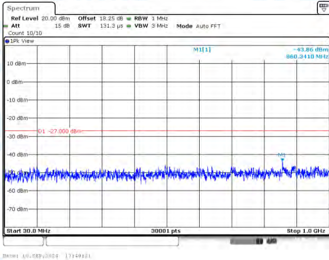
11N20SISO-Ant1-5745-30~1000-PASS
