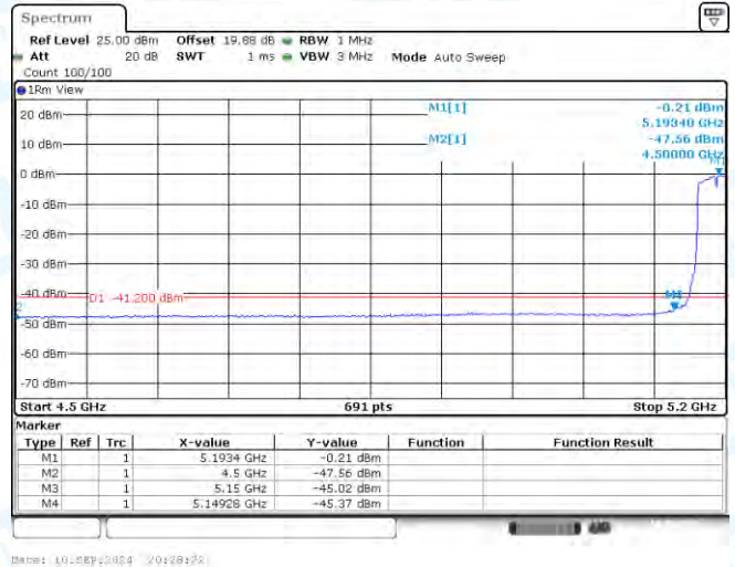
11AC40SISO-Ant1-5190-PASS
