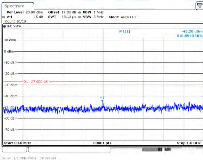
11AX40SISO-Ant1-5190-30~1000-PASS
