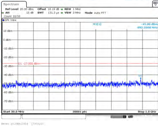
11N20SISO-Ant1-5785-30~1000-PASS
