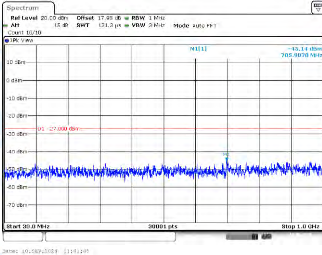
11AX40SISO-Ant1-5230-30~1000-PASS
