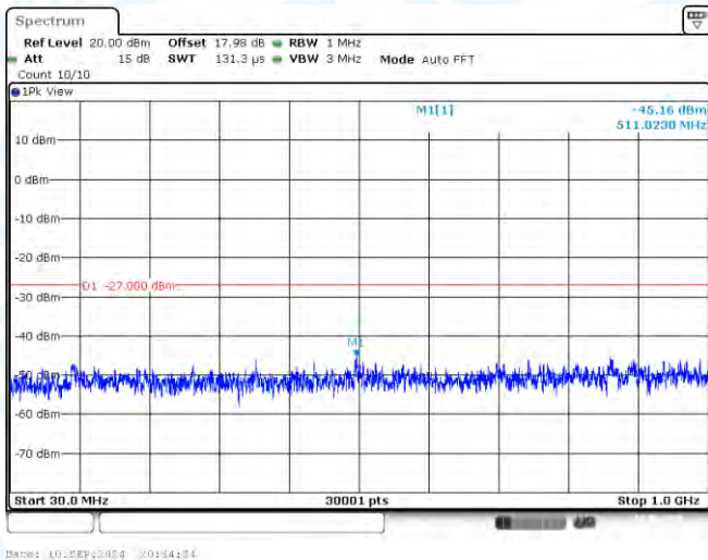
11AC40SISO-Ant1-5230-30~1000-PASS
