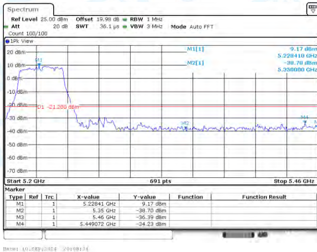
11N40SISO-Ant1-5230-PASS
