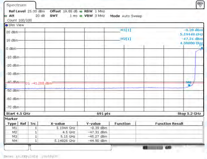
11AX40SISO-Ant1-5190-PASS
