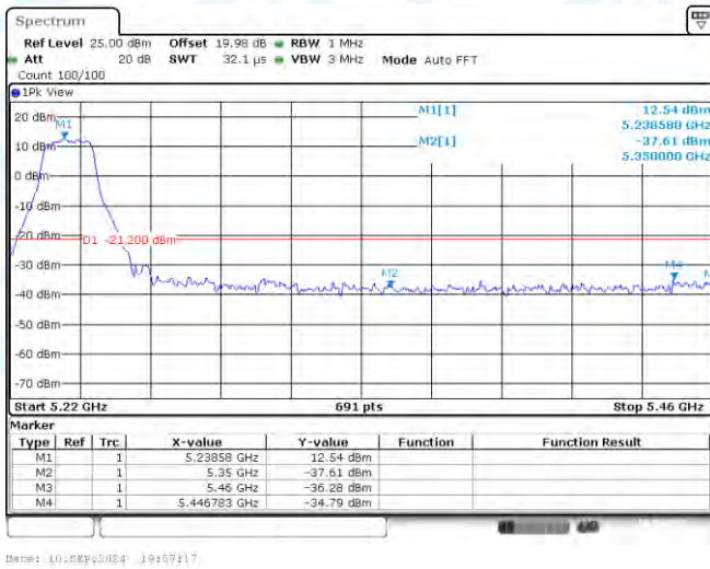
11N20SISO-Ant1-5240-PASS
