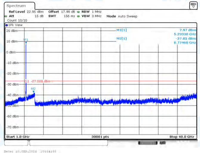
11AC40SISO-Ant1-5230-1000~40000-PASS
