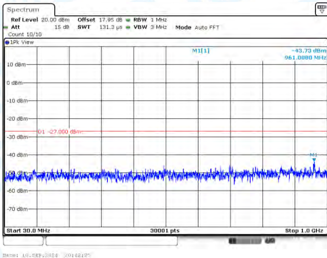
11AX20SISO-Ant1-5180-30~1000-PASS
