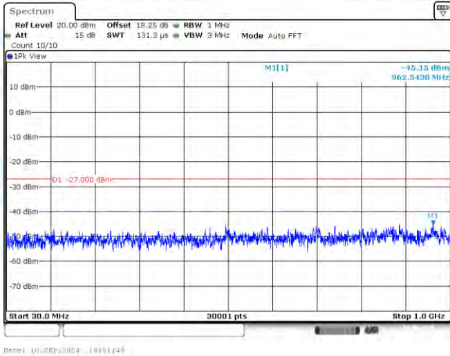
11AC40SISO-Ant1-5755-30~1000-PASS
