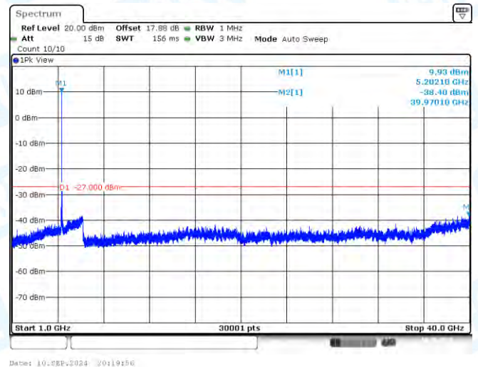
11AC20SISO-Ant1-5200-1000~40000-PASS
