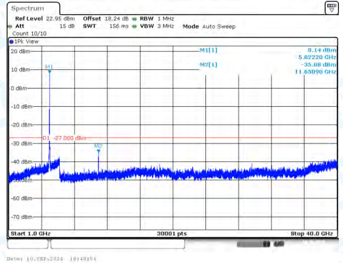
11AC20SISO-Ant1-5825-1000~40000-PASS
