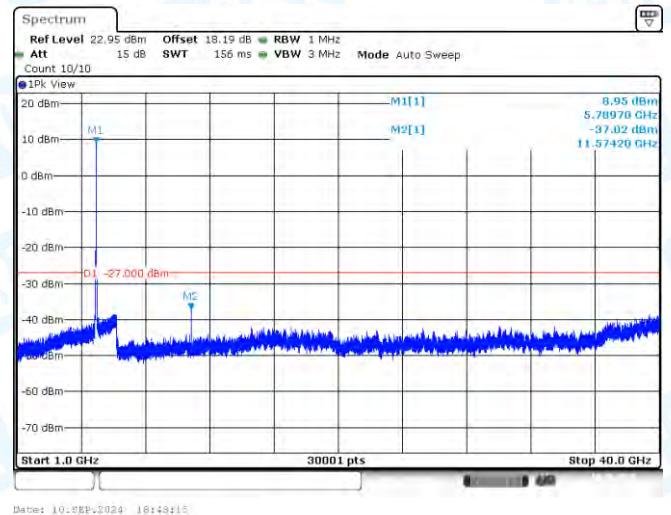
11AC20SISO-Ant1-5785-1000~40000-PASS
