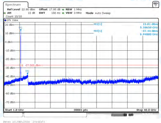
11AX20SISO-Ant1-5180-1000~40000-PASS
