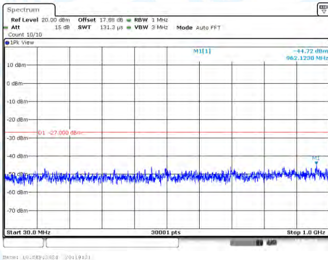
11AC20SISO-Ant1-5200-30~1000-PASS
