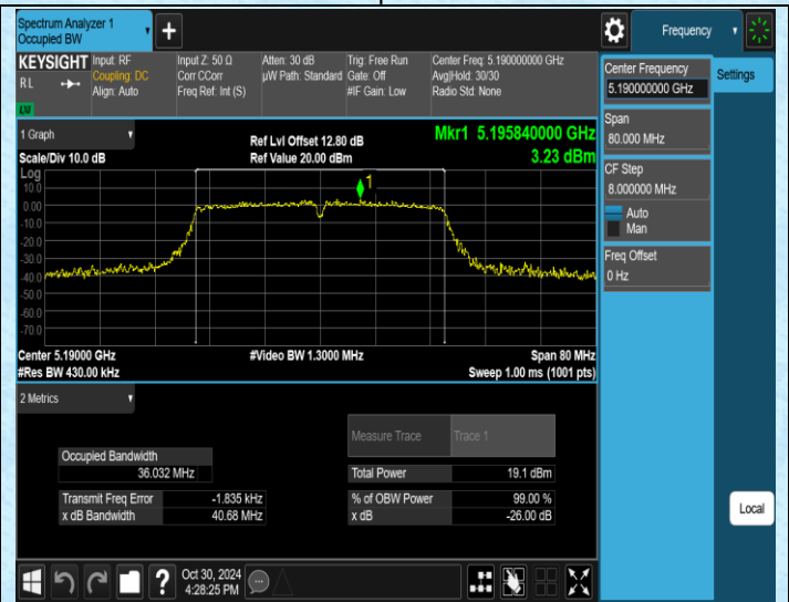
11N40SISO-Ant2-5190
