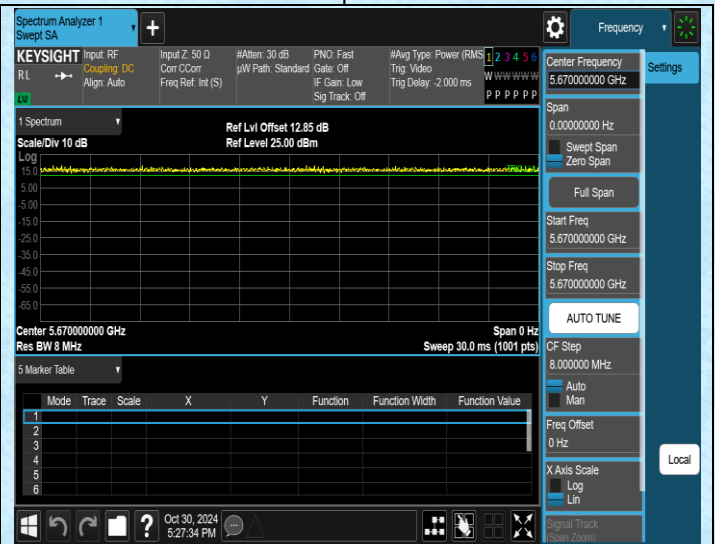
NTNV-11AC40SISO-Ant2-5670
