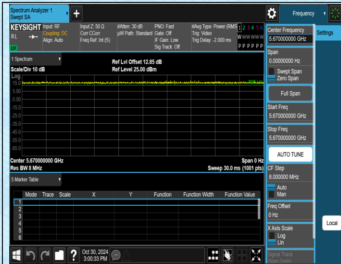
NTNV-11AC40SISO-Ant1-5670
