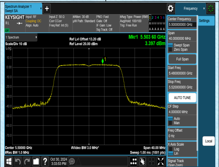
11A-Ant2-5500-PASS
