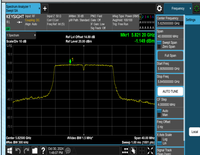
11A-Ant1-5825-PASS
