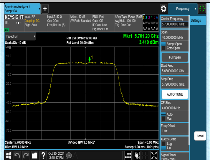
11A-Ant2-5700-PASS
