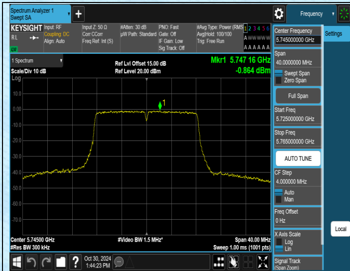
11A-Ant1-5745-PASS
