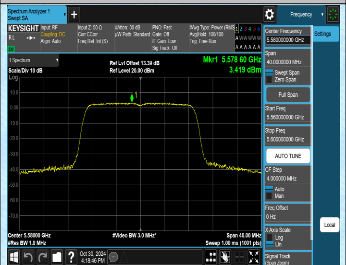
11N20SISO-Ant2-5580-PASS
