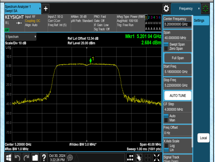
11A-Ant2-5200-PASS
