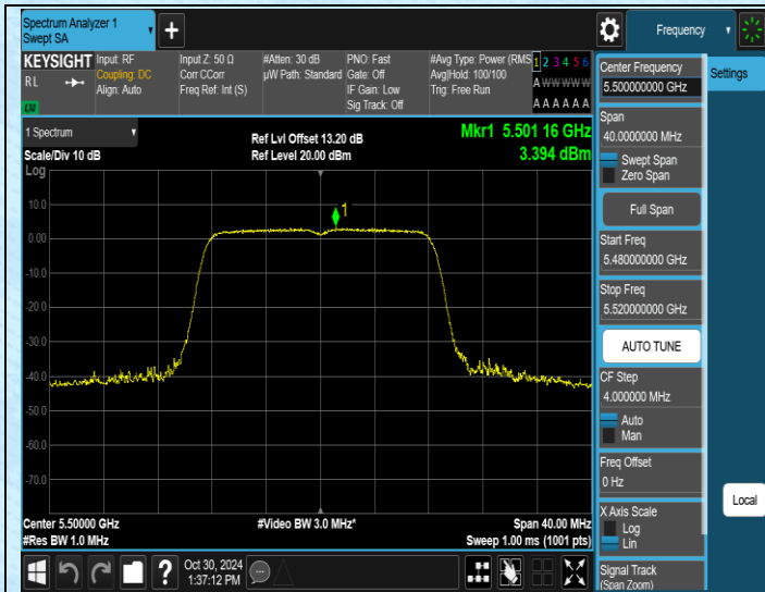
11A-Ant1-5500-PASS
