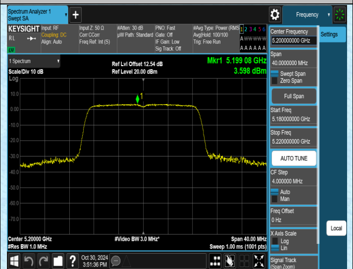
11N20SISO-Ant2-5200-PASS
