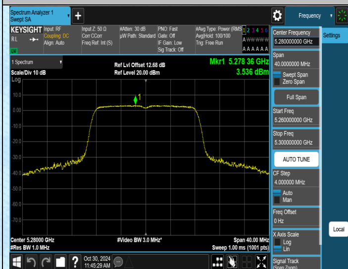
11A-Ant1-5280-PASS
