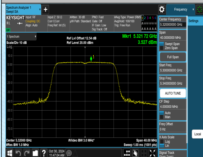
11A-Ant1-5320-PASS
