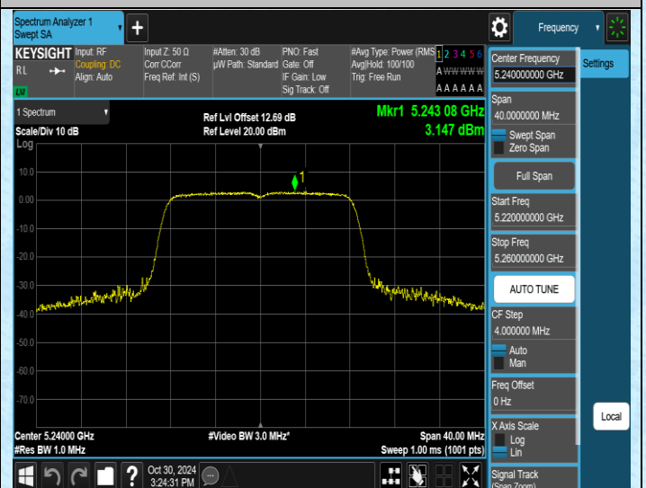
11A-Ant2-5240-PASS
