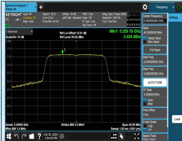
11N20SISO-Ant1-5260-PASS
