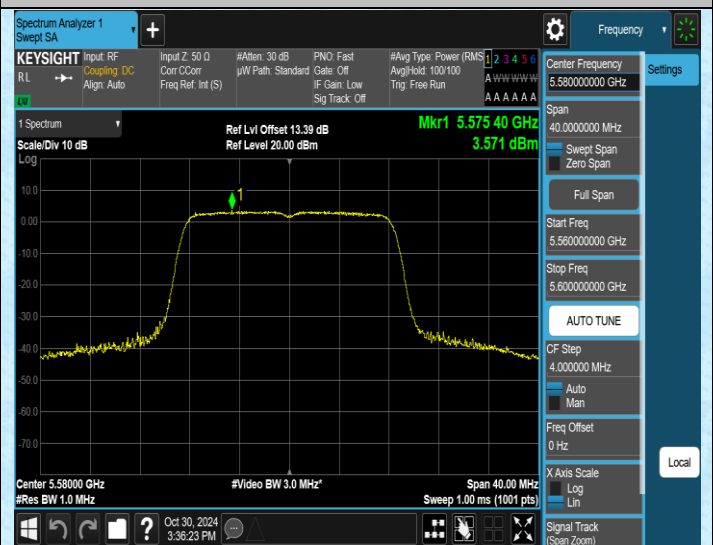
11A-Ant2-5580-PASS
