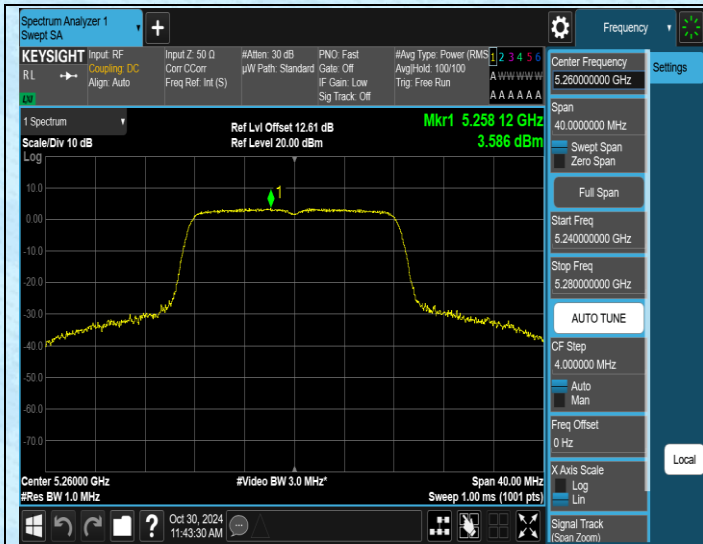
11A-Ant1-5260-PASS
