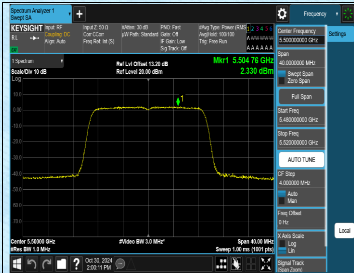
11N20SISO-Ant1-5500-PASS
