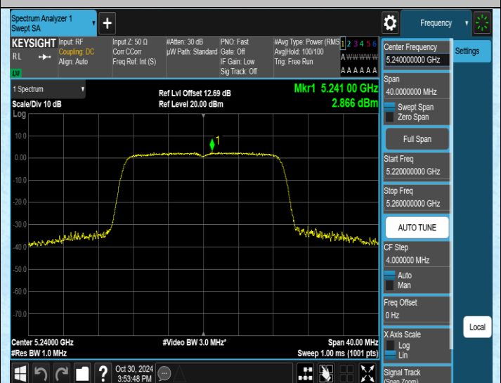
11N20SISO-Ant2-5240-PASS
