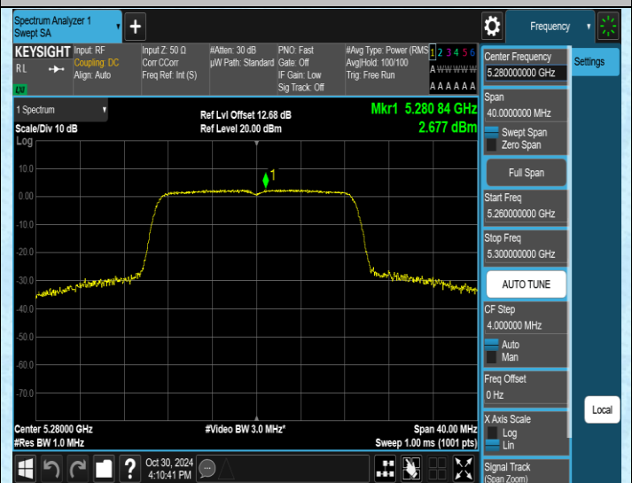
11N20SISO-Ant2-5280-PASS
