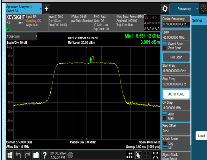
11A-Ant1-5580-PASS
