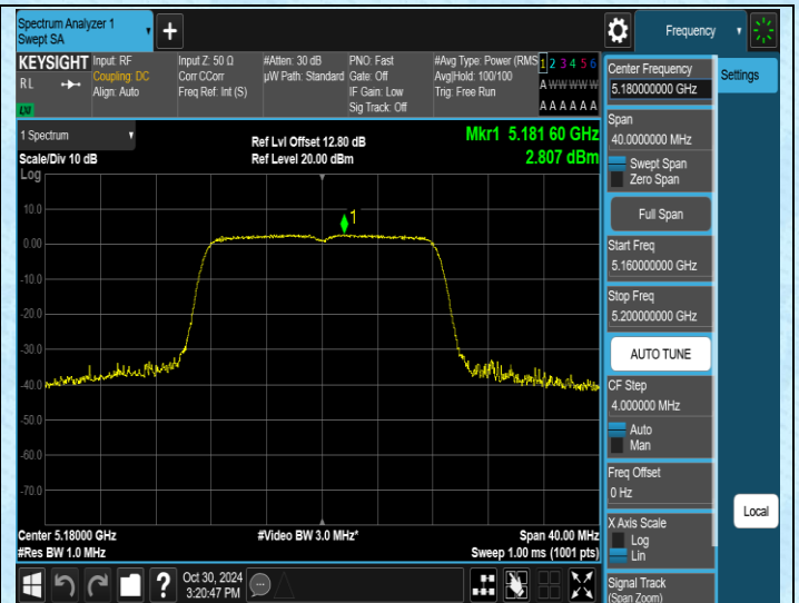
11A-Ant2-5180-PASS
