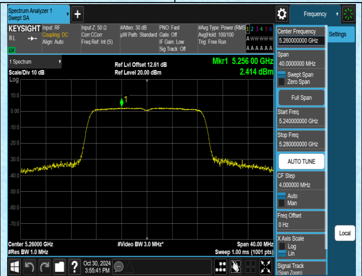
11N20SISO-Ant2-5260-PASS
