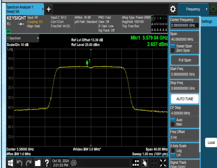
11N20SISO-Ant1-5580-PASS
