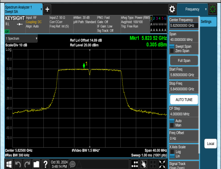
11A-Ant2-5825-PASS
