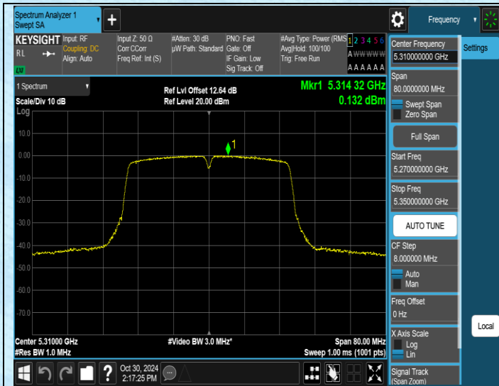
11N40SISO-Ant1-5310-PASS
