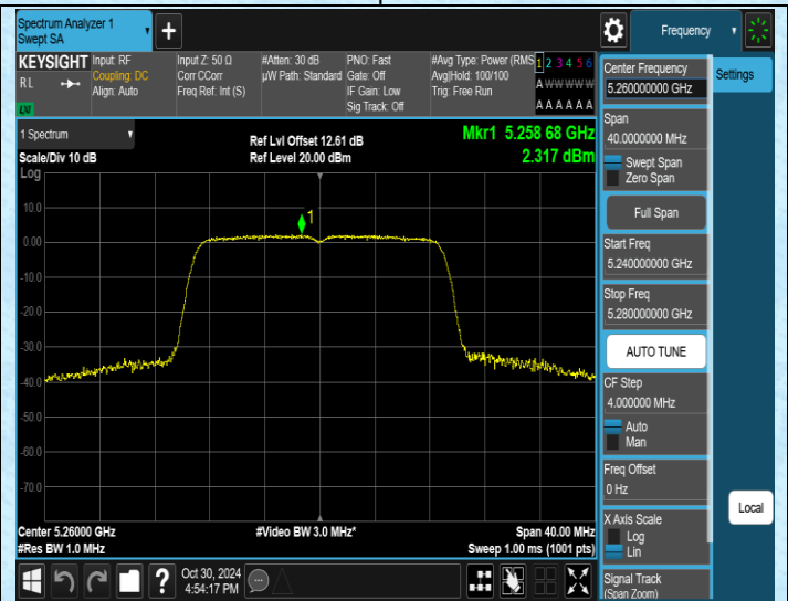
11AC20SISO-Ant2-5260-PASS
