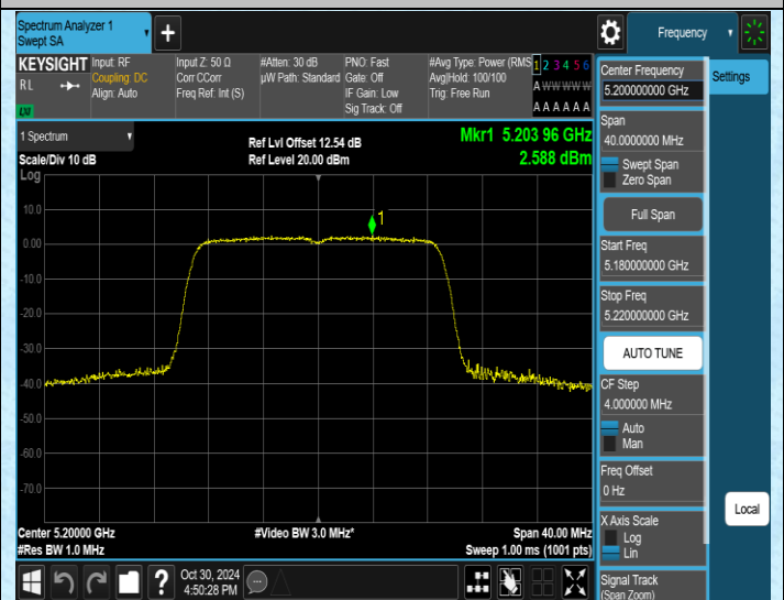
11AC20SISO-Ant2-5200-PASS
