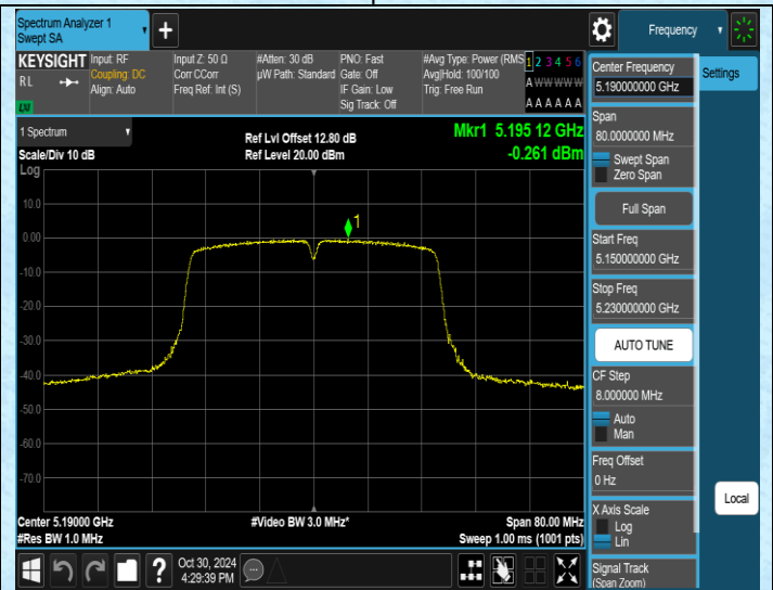
11N40SISO-Ant2-5190-PASS
