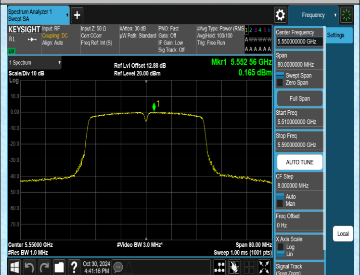
11N40SISO-Ant2-5550-PASS
