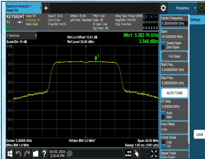
11AC20SISO-Ant1-5260-PASS
