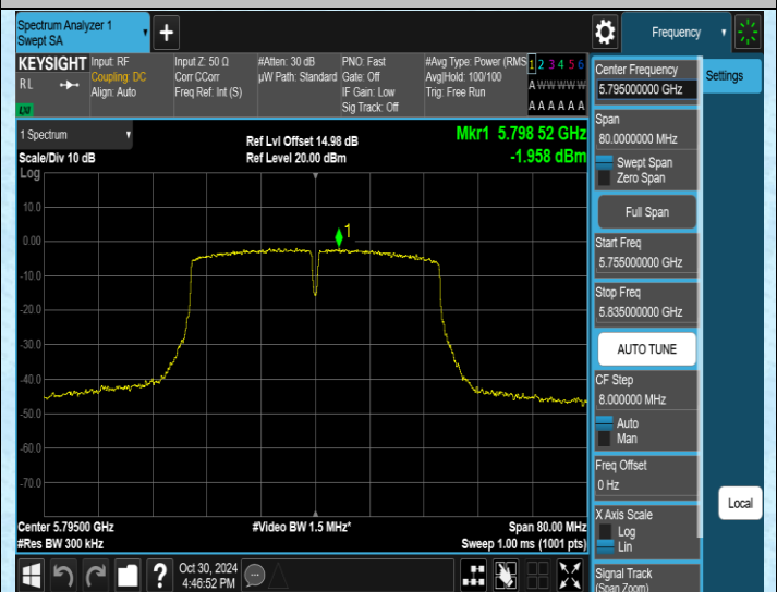
11N40SISO-Ant2-5795-PASS
