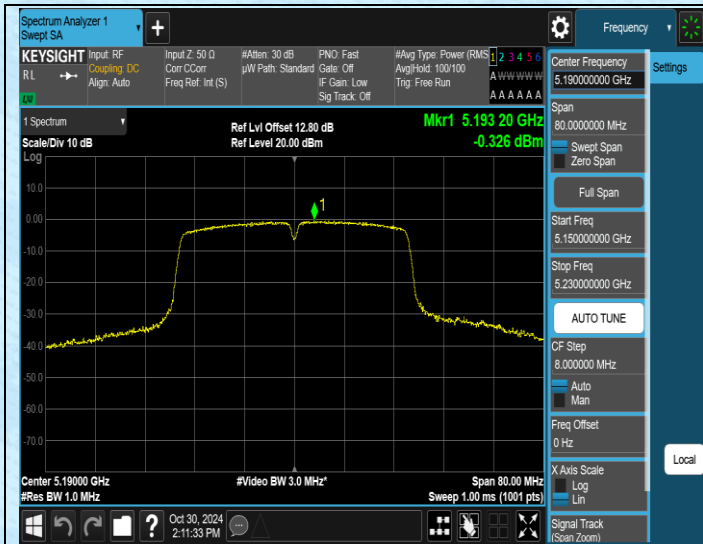
11N40SISO-Ant1-5190-PASS
