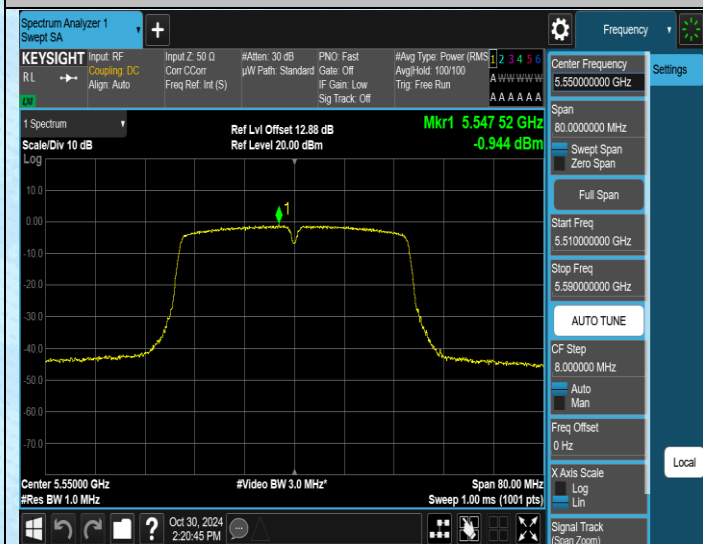
11N40SISO-Ant1-5550-PASS
