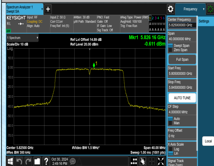
11AC20SISO-Ant1-5825-PASS
