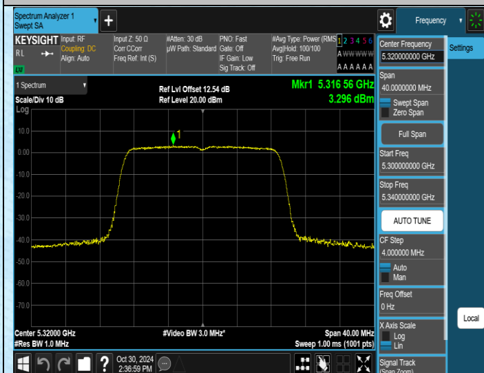
11AC20SISO-Ant1-5320-PASS
