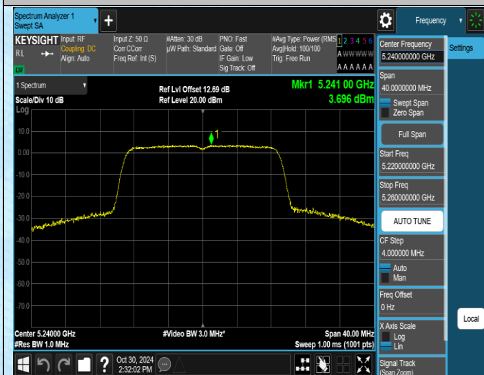
11AC20SISO-Ant1-5240-PASS
