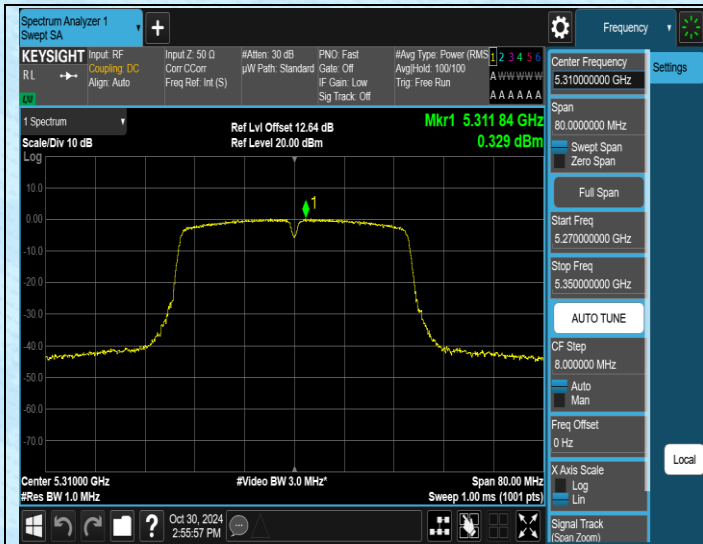
11AC40SISO-Ant1-5310-PASS
