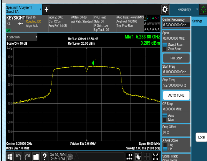
11N40SISO-Ant1-5230-PASS
