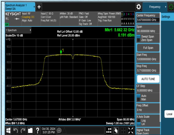
11AC40SISO-Ant1-5670-PASS
