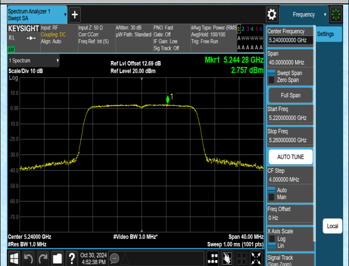
11AC20SISO-Ant2-5240-PASS
