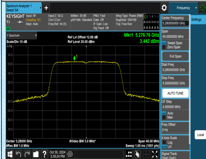
11AC20SISO-Ant1-5280-PASS
