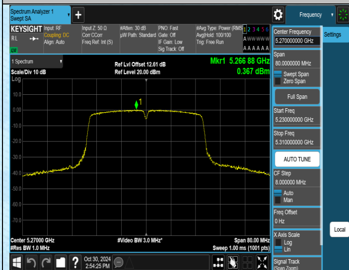
11AC40SISO-Ant1-5270-PASS
