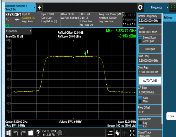
11N20MIMO-Ant1-5320-PASS
