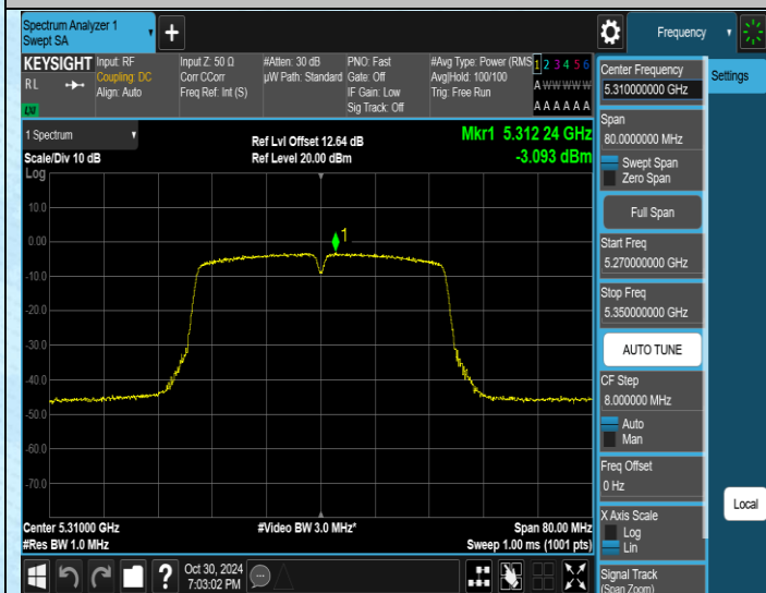
11N40MIMO-Ant1-5310-PASS
