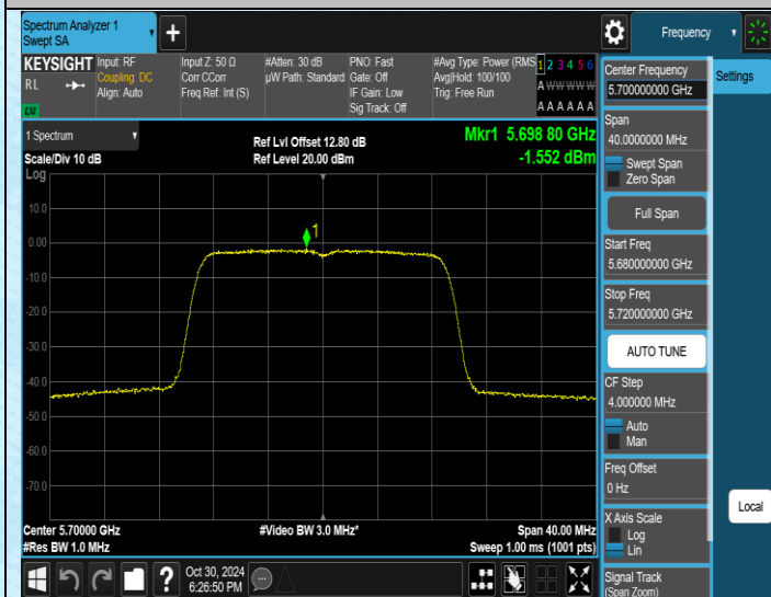
11N20MIMO-Ant1-5700-PASS
