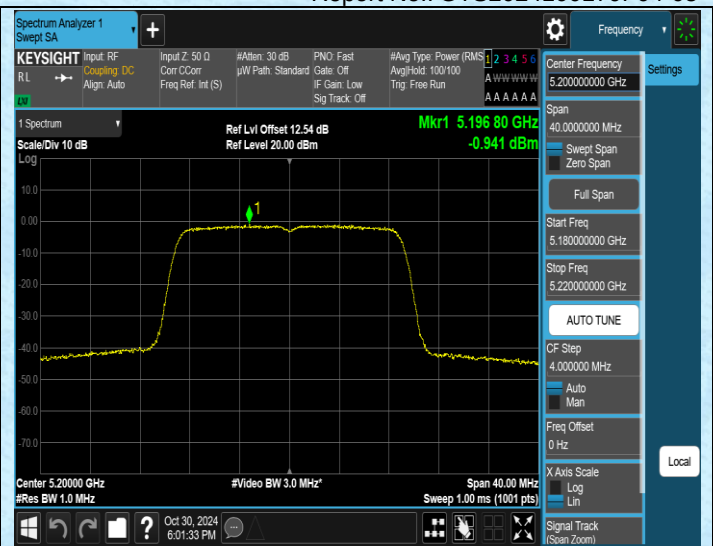
11N20MIMO-Ant2-5200-PASS
