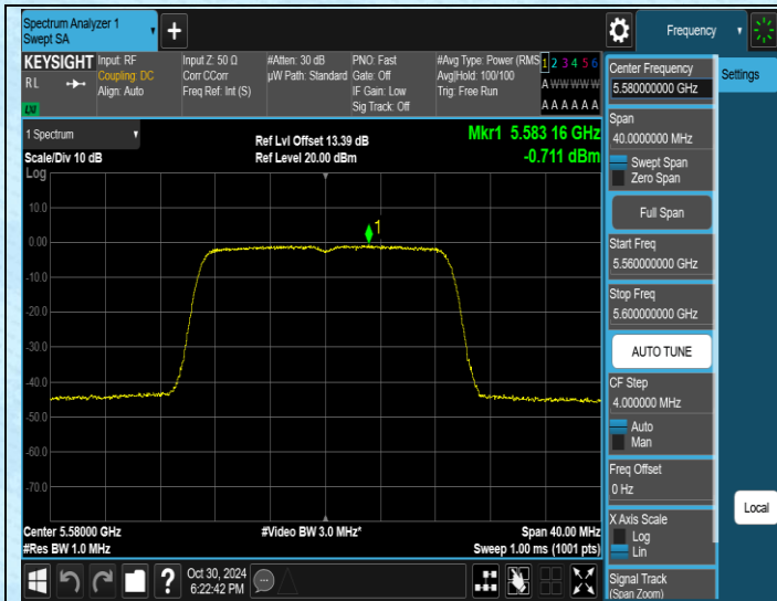
11N20MIMO-Ant1-5580-PASS
