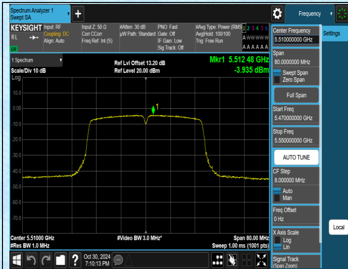
11N40MIMO-Ant1-5510-PASS
