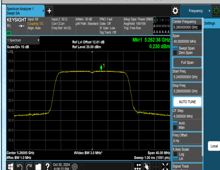
11N20MIMO-Ant1-5260-PASS
