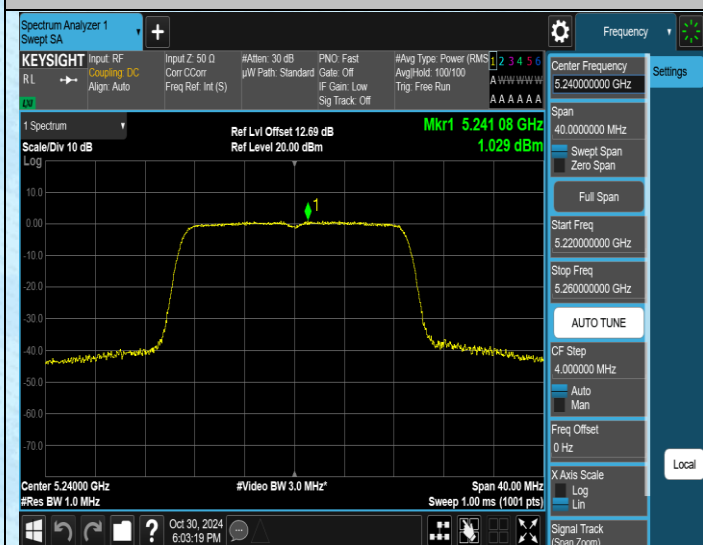
11N20MIMO-Ant1-5240-PASS
