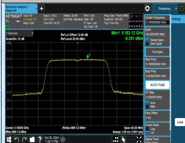
11AC20MIMO-Ant1-5180-PASS
