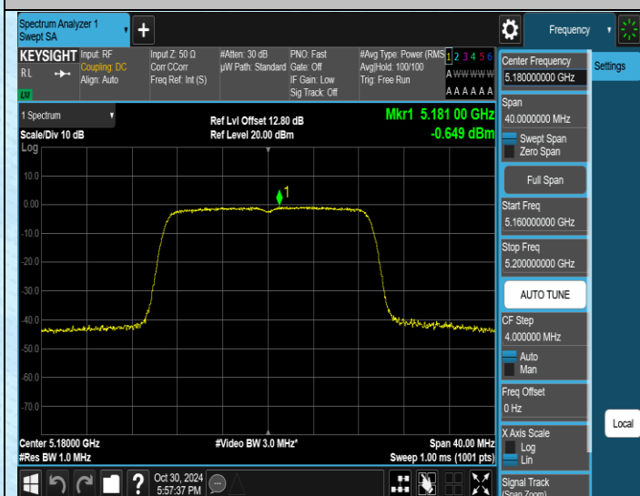
11N20MIMO-Ant1-5180-PASS
