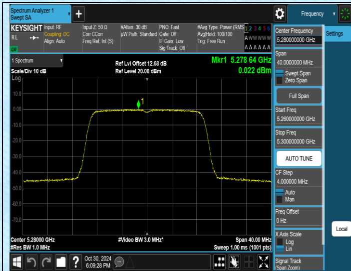
11N20MIMO-Ant1-5280-PASS
