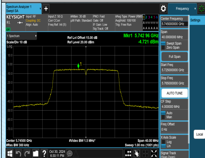
11N20MIMO-Ant1-5745-PASS
