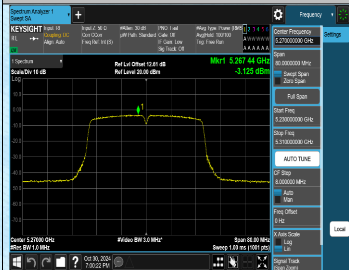
11N40MIMO-Ant1-5270-PASS
