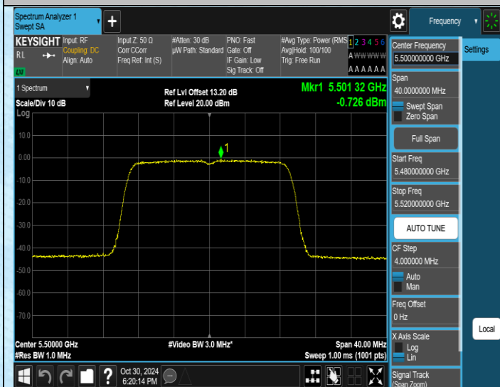
11N20MIMO-Ant1-5500-PASS
