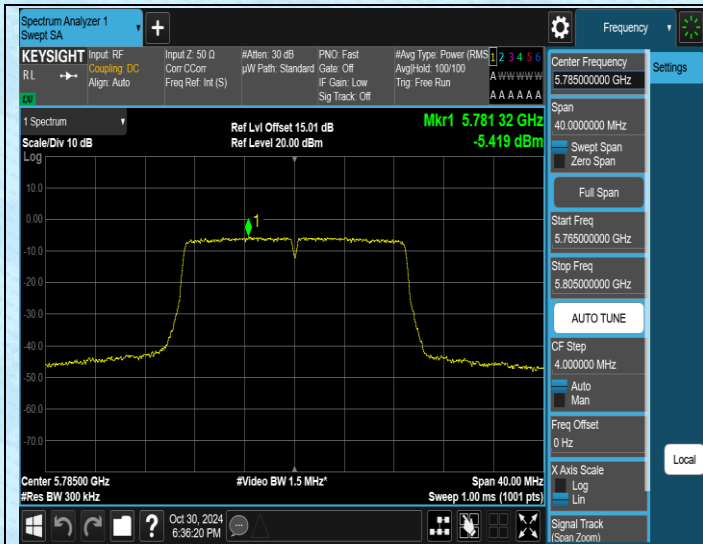
11N20MIMO-Ant1-5785-PASS
