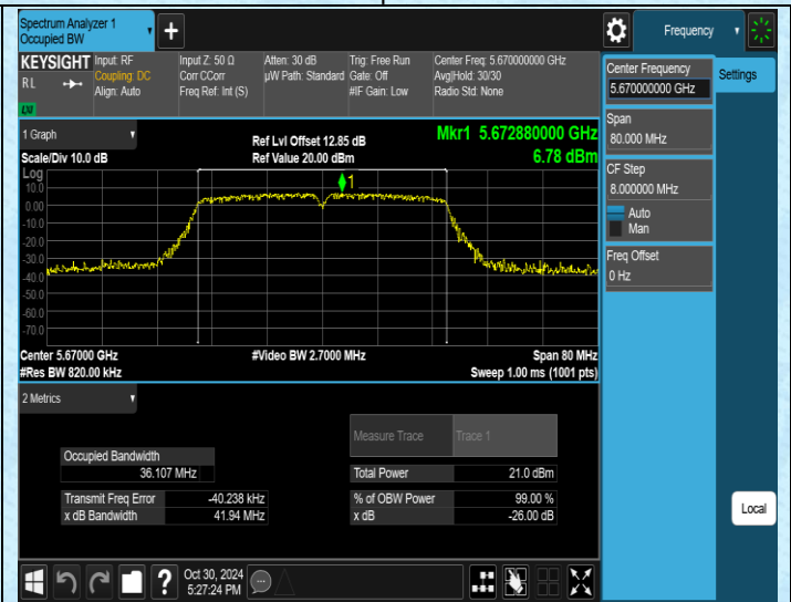
11AC40SISO-Ant2-5670
