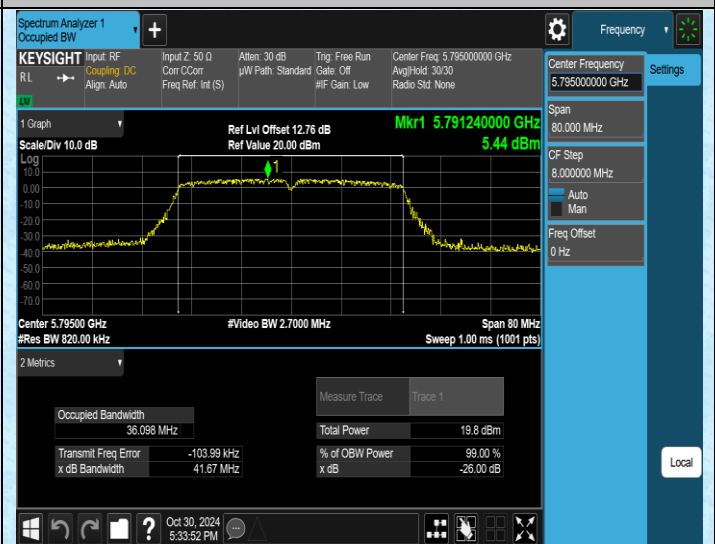
11AC40SISO-Ant2-5795
