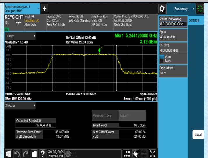
11N20MIMO-Ant2-5240
