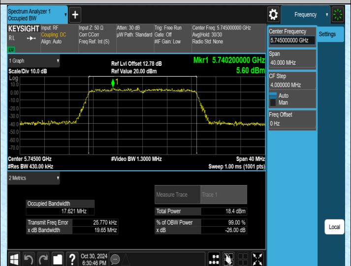
11N20MIMO-Ant2-5745
