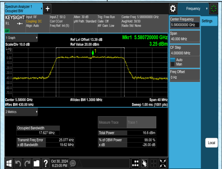
11N20MIMO-Ant2-5580
