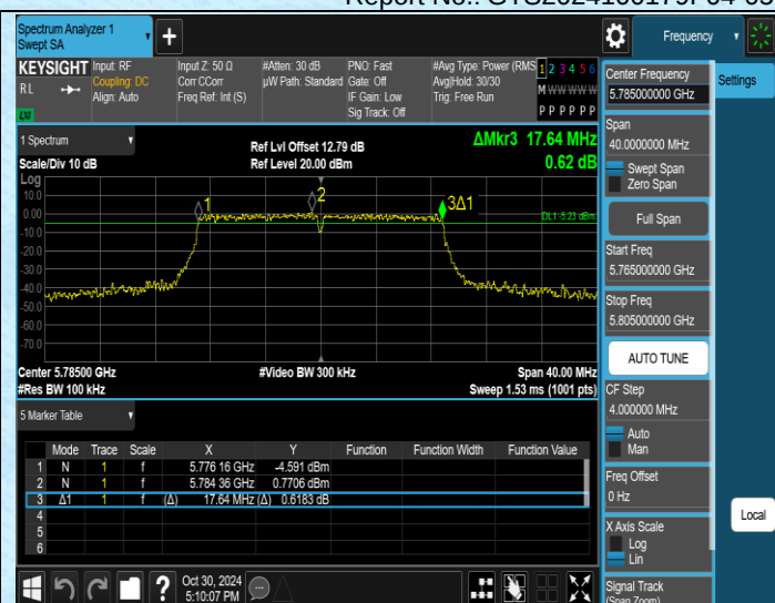
11AC20SISO-Ant2-5785-PASS
