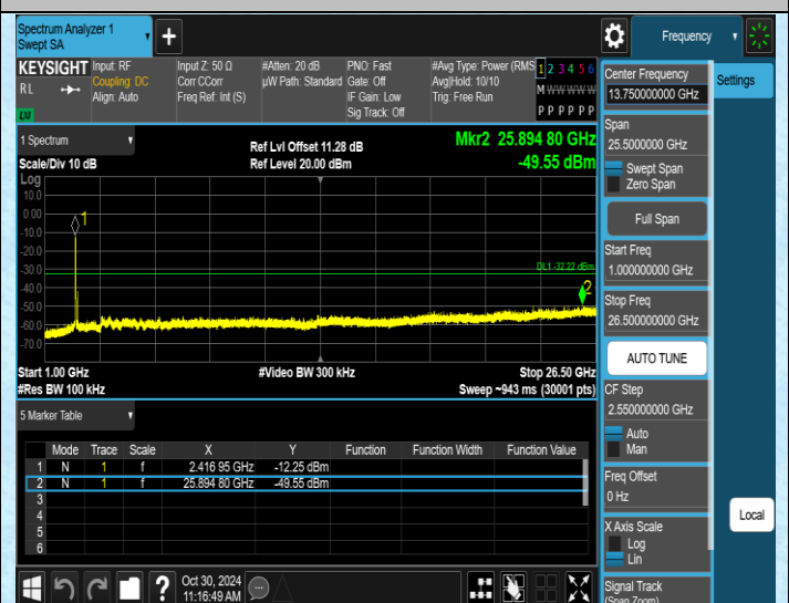
11N40MIMO-Ant2-2422-1000~26500-PASS
