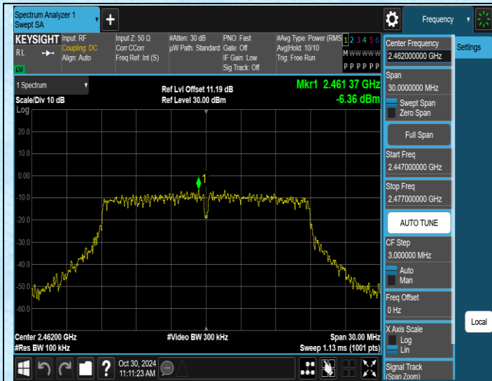
11N20MIMO-Ant1-2462-0~Reference-PASS
