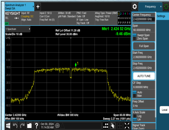
11N40MIMO-Ant1-2422-0~Reference-PASS
