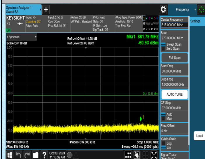
11N40MIMO-Ant2-2422-30~1000-PASS
