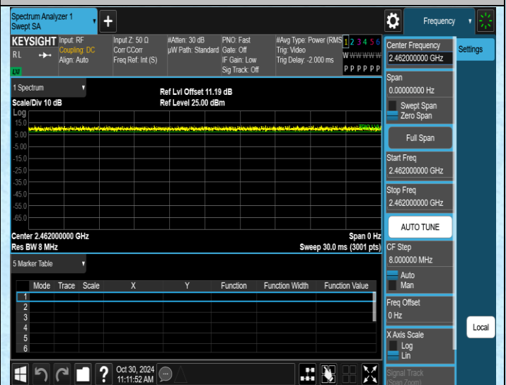
NTNV-11N20MIMO-Ant2-2462
