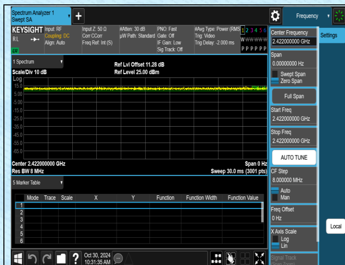
NTNV-11N40SISO-Ant1-2422
