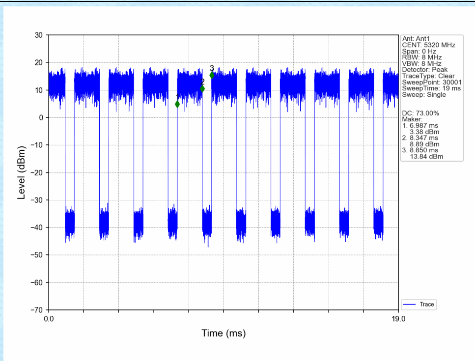
802.11a_HCH_5320MHz_Ant1_NTNV
