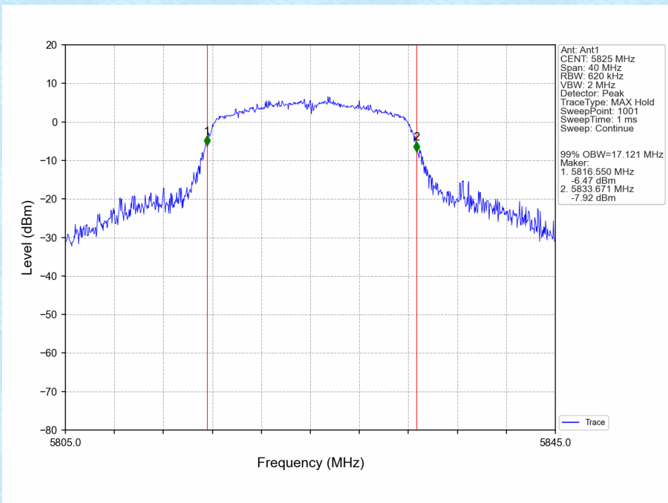
802.11a_HCH_5825MHz_Ant1_NTNV
