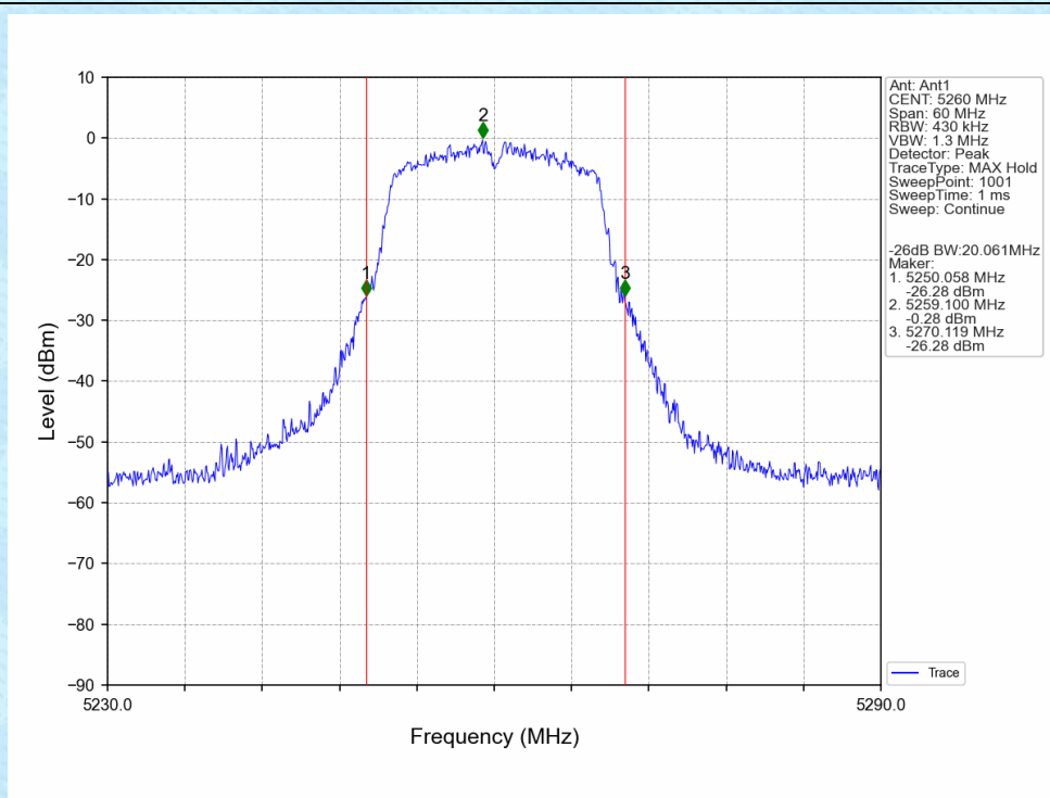
802.11a_LCH_5260MHz_Ant1_NTNV
