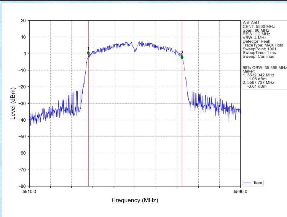
802.11n(HT40)_MCH_5550MHz_Ant1_NTNV
