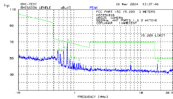
Camera Coplanar
