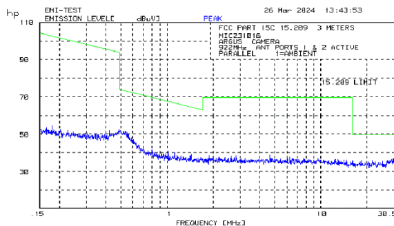
Camera Parallel
