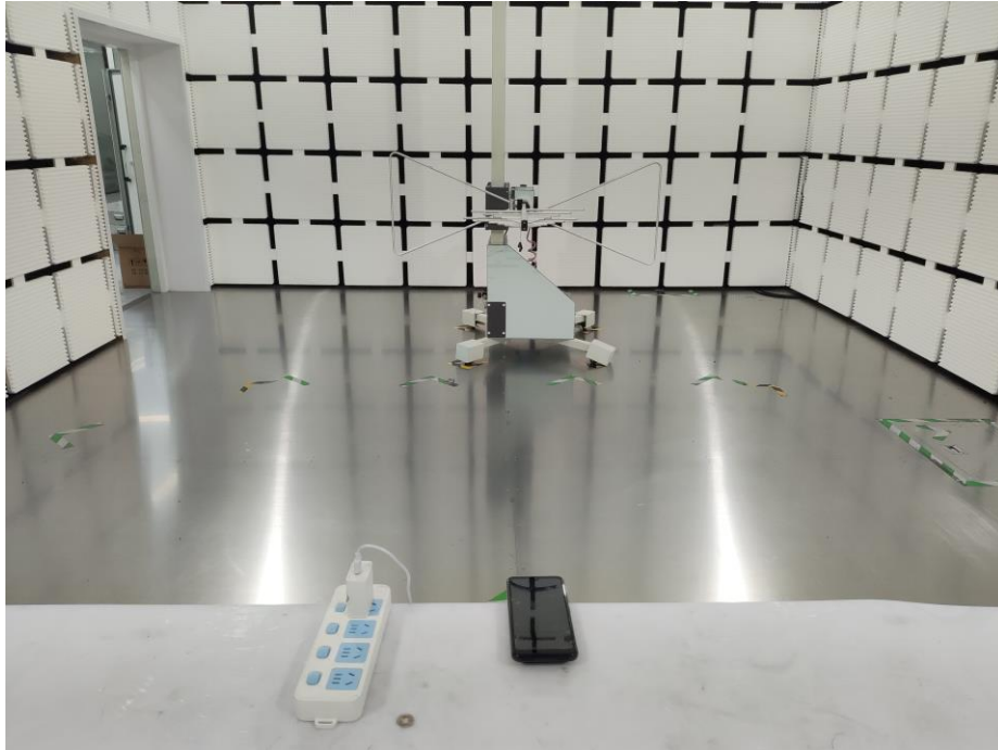
Radiation (30MHz-1000MHz)
