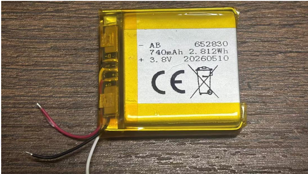
Photo 11 Battery Appearance
