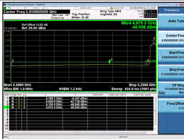
11N40SISO_Ant1_Low_5190_Peak
