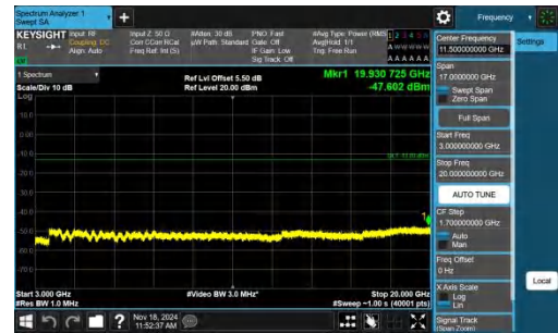
Band4-20MHz-QPSK-20175-1RB#99-3000~20000-PASS
