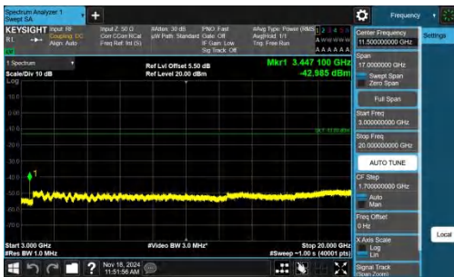
Band4-20MHz-QPSK-20175-1RB#0-3000~20000-PASS
