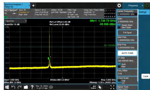
Band4-3MHz-QPSK-20385-1RB#0-1000~3000-PASS
