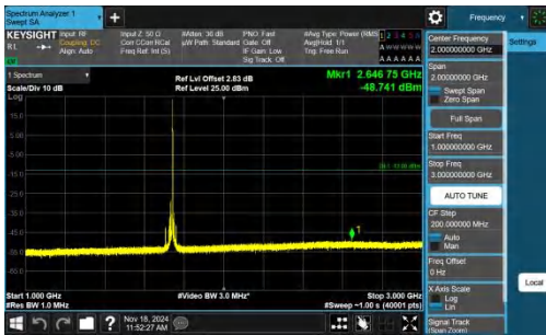
Band4-20MHz-QPSK-20175-1RB#99-1000~3000-PASS
