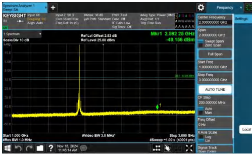
Band4-15MHz-QPSK-20175-1RB#74-1000~3000-PASS
