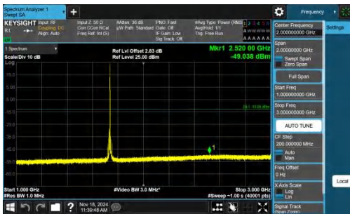
Band4-10MHz-QPSK-20175-1RB#49-1000~3000-PASS
