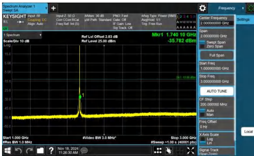
Band4-3MHz-QPSK-20175-1RB#14-1000~3000-PASS
