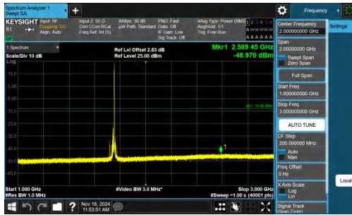
Band4-20MHz-QPSK-20300-1RB#99-1000~3000-PASS
