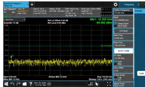
Band4-15MHz-QPSK-20325-1RB#74-0.009~0.15-PASS
