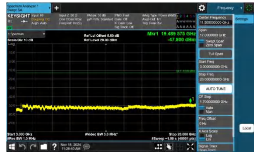
Band4-3MHz-QPSK-20175-1RB#14-3000~20000-PASS
