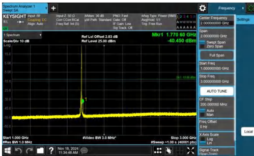
Band4-5MHz-QPSK-20375-1RB#24-1000~3000-PASS
