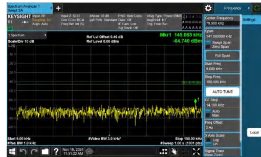
Band4-5MHz-QPSK-19975-1RB#24-0.009~0.15-PASS
