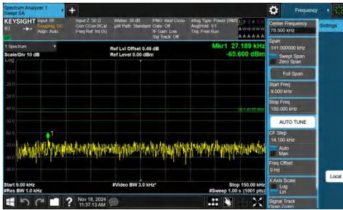
Band4-10MHz-QPSK-20000-1RB#0-0.009~0.15-PASS
