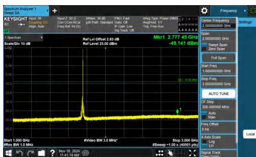
Band4-10MHz-QPSK-20350-1RB#49-1000~3000-PASS
