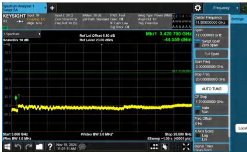
Band4-5MHz-QPSK-19975-1RB#0-3000~20000-PASS
