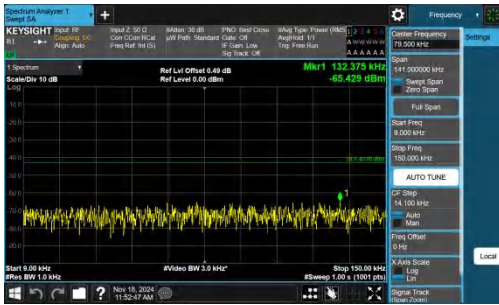
Band4-20MHz-QPSK-20300-1RB#0-0.009~0.15-PASS
