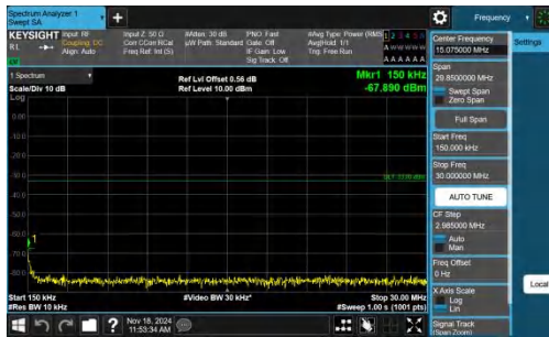
Band4-20MHz-QPSK-20300-1RB#99-0.15~30-PASS
