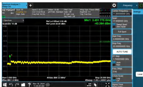
Band4-15MHz-QPSK-20175-1RB#0-3000~20000-PASS
