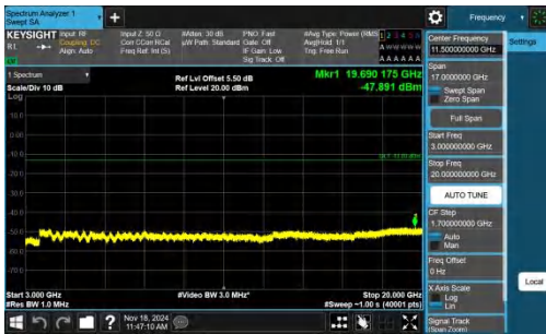
Band4-15MHz-QPSK-20325-1RB#0-3000~20000-PASS
