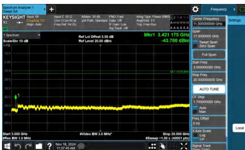
Band4-10MHz-QPSK-20000-1RB#0-3000~20000-PASS
