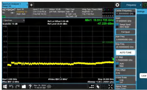
Band4-10MHz-QPSK-20350-1RB#0-3000~20000-PASS
