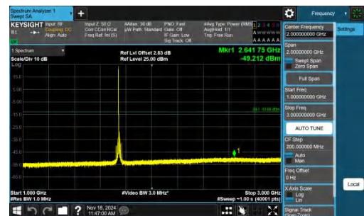
Band4-15MHz-QPSK-20325-1RB#0-1000~3000-PASS
