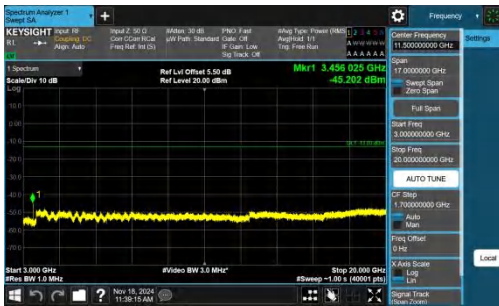
Band4-10MHz-QPSK-20175-1RB#0-3000~20000-PASS
