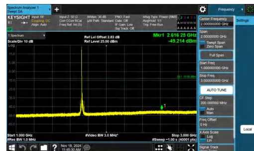
Band4-15MHz-QPSK-20175-1RB#0-1000~3000-PASS
