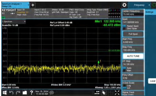
Band4-5MHz-QPSK-20375-1RB#0-0.009~0.15-PASS
