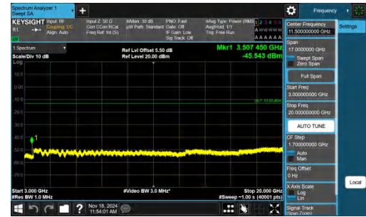
Band4-20MHz-QPSK-20300-1RB#99-3000~20000-PASS
