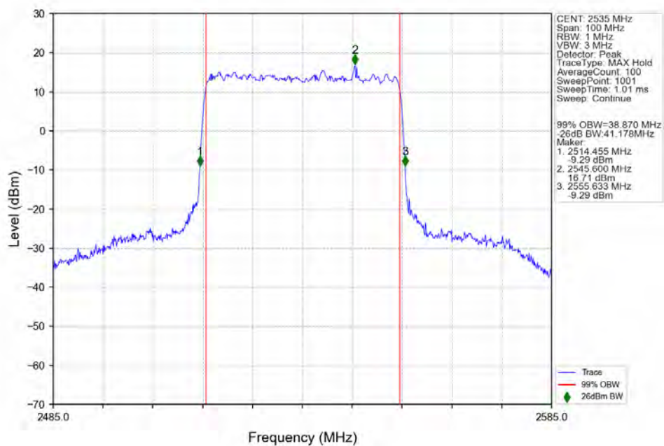
n7_15kHz_SISO_NTNV_40MHz_DFT-s-OFDM 64 QAM 2535MHz_Outer_Full_Ant1
