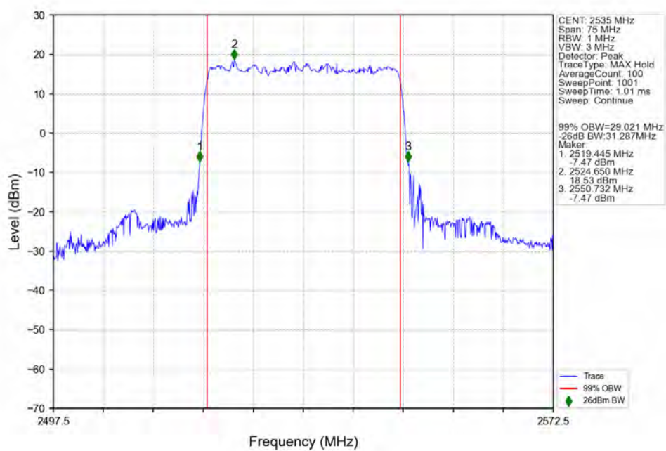
n7_15kHz_SISO_NTNV_30MHz_DFT-s-OFDM QPSK_2535MHz_Outer_Full_Ant1
