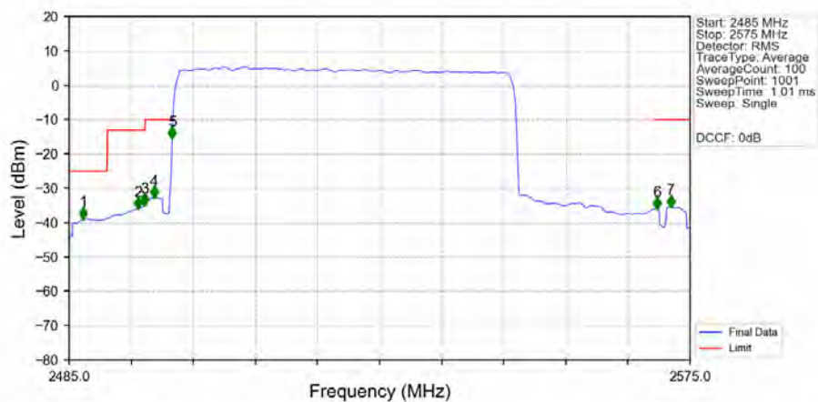
n7 15kHz SISO NTNV 50MHz DFT-s-OFDM QPSK 2525MHz Outer Full Ant1
