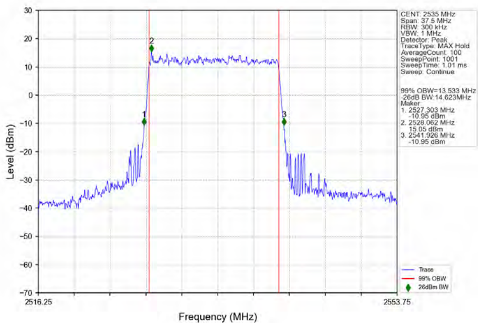
n7_15kHz_SISO_NTNV_15MHz_DFT-s-OFDM 64 QAM 2535MHz_Outer_Full_Ant1
