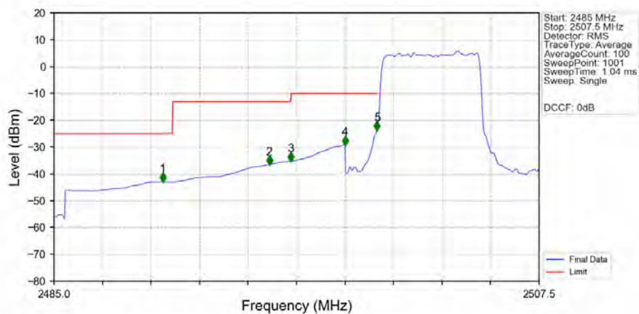
n7_15kHz_SISO_NTNV_5MHz_DFT-s-OFDM_QPSK_2502.5MHz_Outer_Full_Ant1
