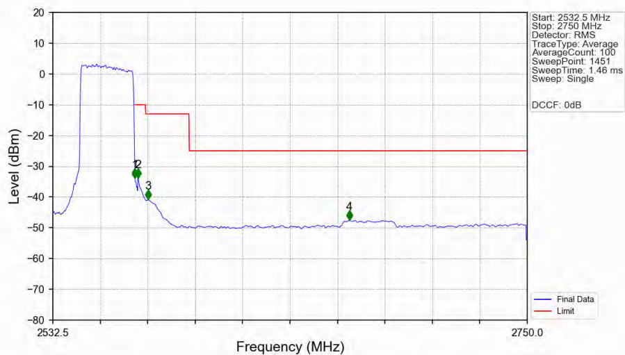
n7_15kHz_SISO_NTNV_25MHz_CP-OFDM_QPSK_2557.5MHz_Outer_Full_Ant1
