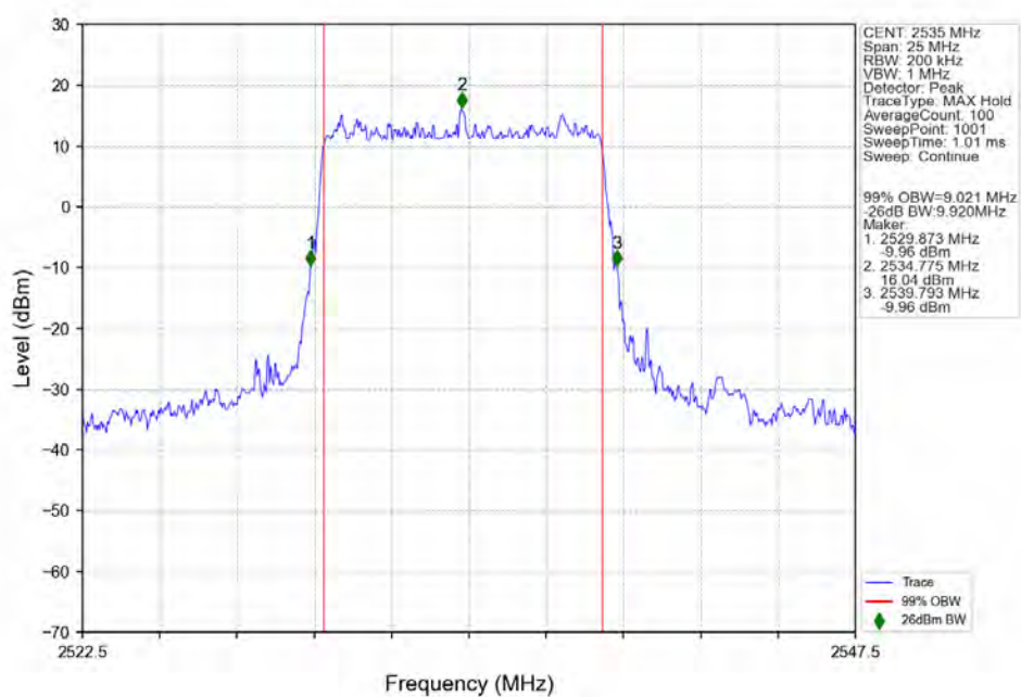
n7_15kHz_SISO_NTNV_10MHz_DFT-s-OFDM 64 QAM 2535MHz_Outer_Full_Ant1
