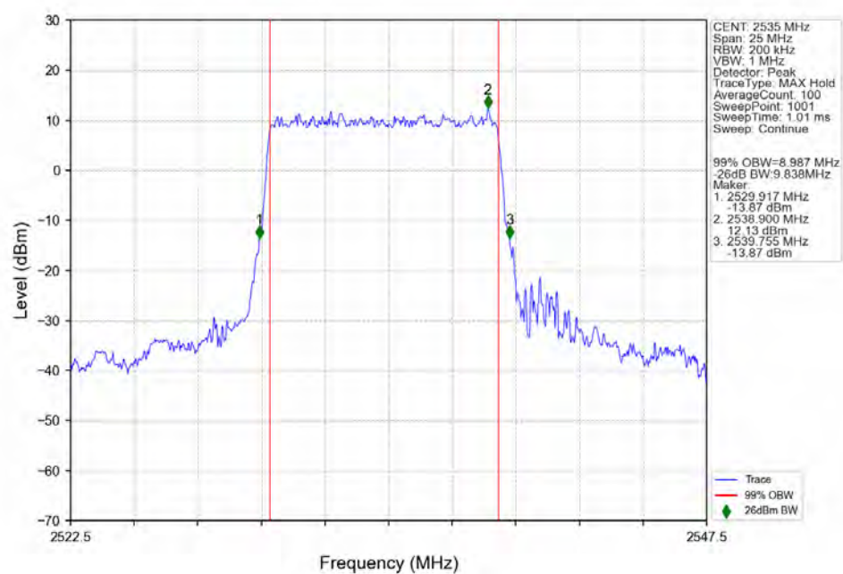
n7_15kHz_SISO_NTNV_10MHz_CP-OFDM_QPSK_2535MHz_Outer_Full_Ant1
