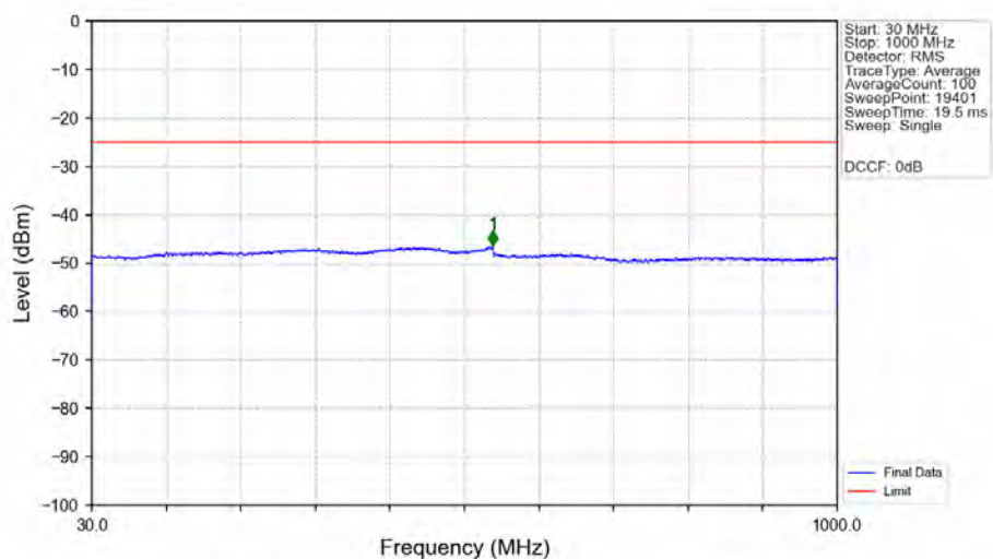
n7_15kHz_SISO_NTNV_5MHz_DFT-s-OFDM_QPSK_2535MHz_Edge_1RB_Left_Ant1
