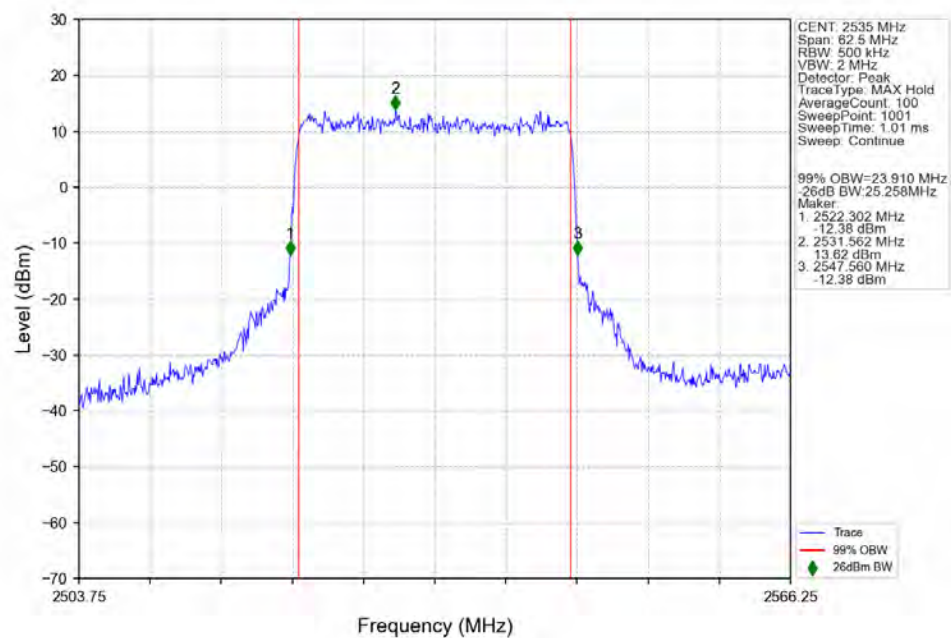
n7_15kHz_SISO_NTNV_25MHz_CP-OFDM_QPSK_2535MHz_Outer_Full_Ant1
