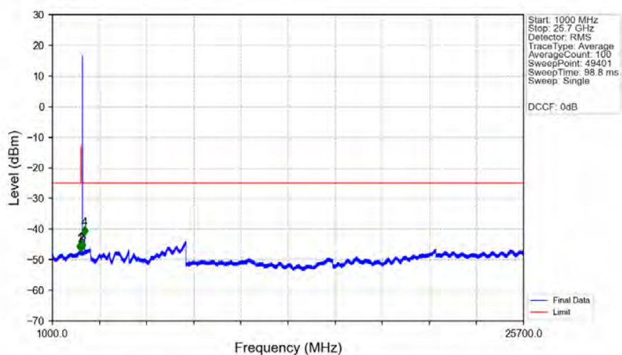
n7_15kHz_SISO_NTNV_5MHz_DFT-s-OFDM_QPSK_2567.5MHz_Edge_1RB_Right_Ant1
