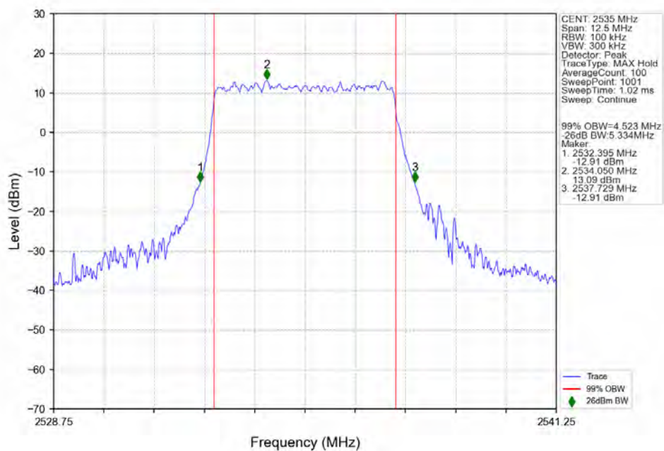
n7_15kHz_SISO_NTNV_5MHz_CP-OFDM QPSK 2535MHz_Outer_Full_Ant1
