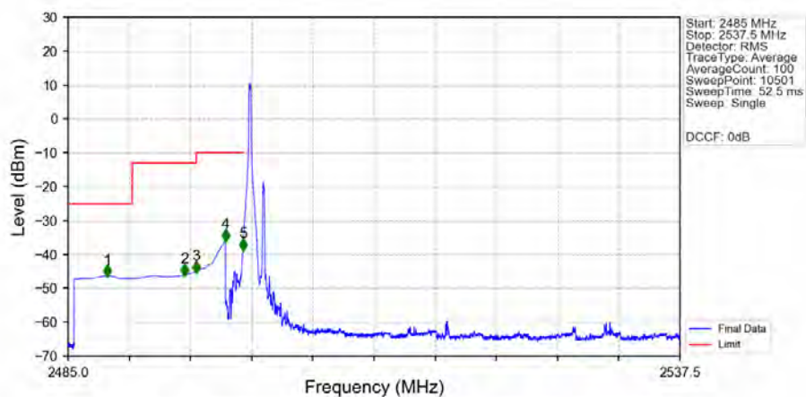
n7_15kHz_SISO_NTNV_25MHz_DFT-s-OFDM_QPSK_2512.5MHz_Edge_1RB_Left_Ant1
