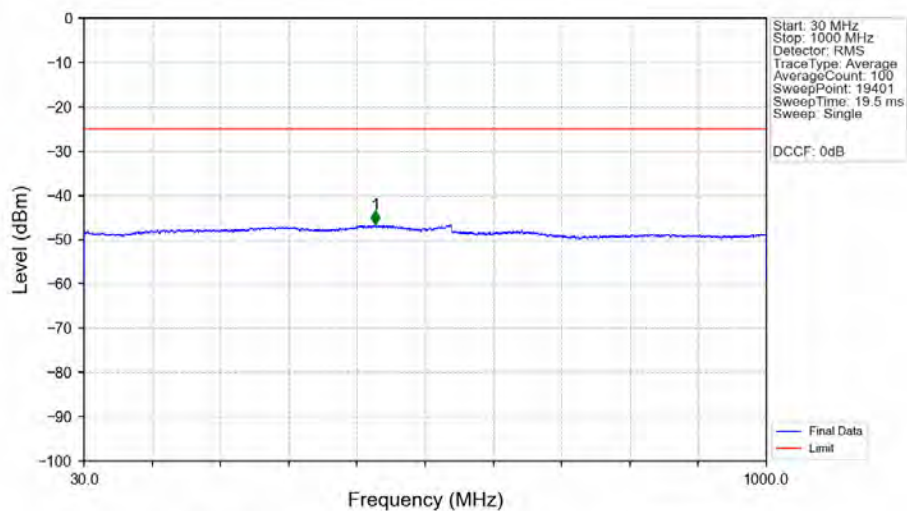
n7_15kHz_SISO_NTNV_50MHz_DFT-s-OFDM_QPSK_2525MHz_Edge_1RB_Left_Ant1
