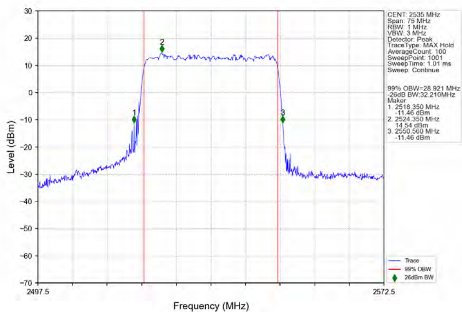
n7_15kHz_SISO_NTNV_30MHz_CP-OFDM_QPSK_2535MHz_Outer_Full_Ant1
