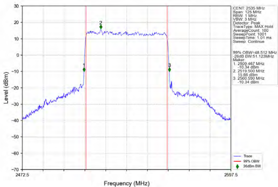
n7_15kHz_SISO_NTNV_50MHz_DFT-s-OFDM 64 QAM 2535MHz_Outer_Full_Ant1
