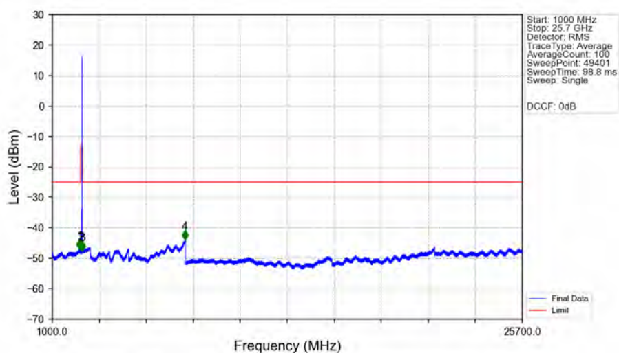
n7_15kHz_SISO_NTNV_25MHz_DFT-s-OFDM_QPSK_2557.5MHz_Edge_1RB_Right_Ant1
