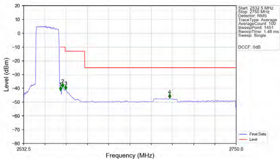
n7_15kHz_SISO_NTNV_25MHz_DFT-s-OFDM_QPSK_2557.5MHz_Outer_Full_Ant1
