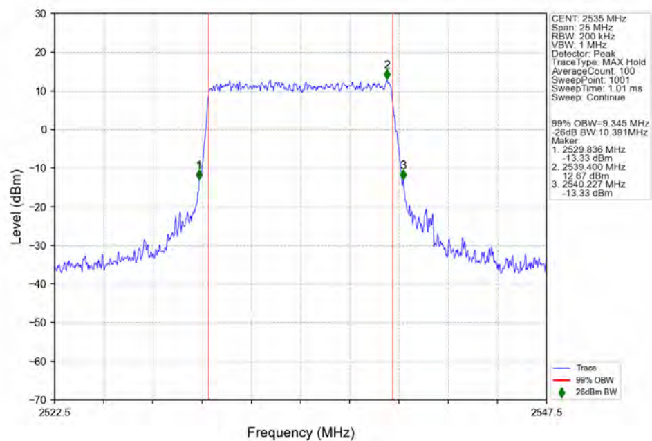
n7_15kHz_SISO_NTNV_10MHz_CP-OFDM_QPSK_2535MHz_Outer_Full_Ant1
