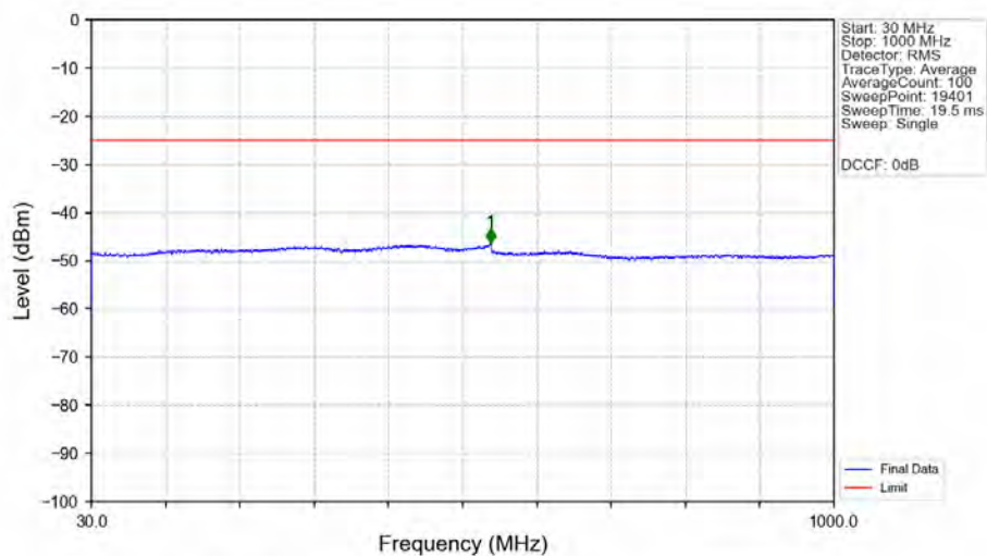
n7_15kHz_SISO_NTNV_25MHz_CP-OFDM_QPSK_2512.5MHz_Edge_1RB_Left_Ant1
