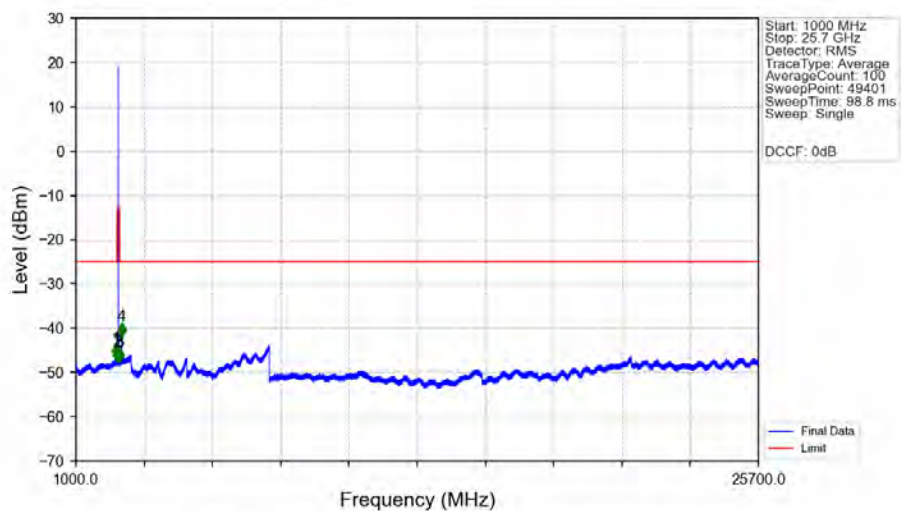
n7_15kHz_SISO_NTNV_5MHz_DFT-s-OFDM_QPSK_2535MHz_Edge_1RB_Left_Ant1
