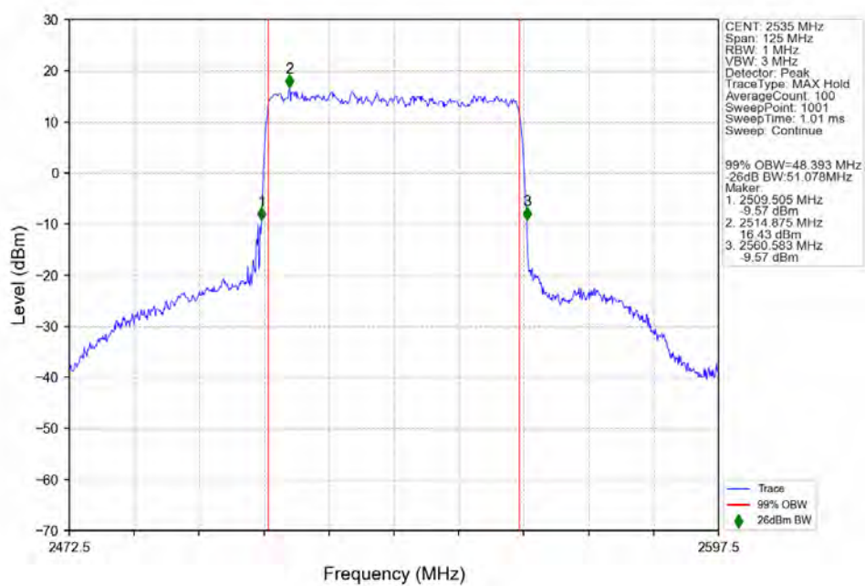
n7_15kHz_SISO_NTNV_50MHz_DFT-s-OFDM QPSK_2535MHz_Outer_Full_Ant1
