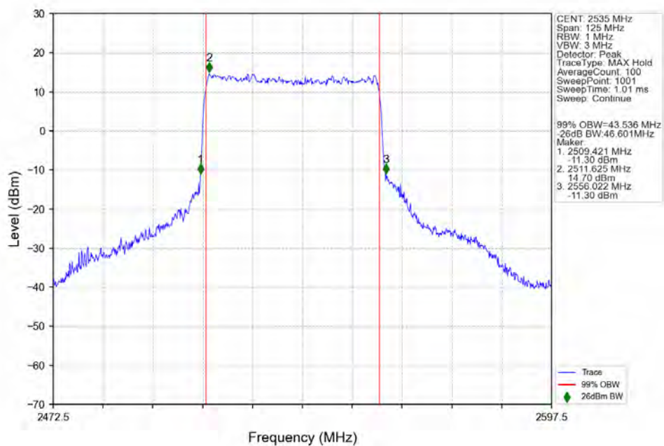
n7_15kHz_SISO_NTNV_50MHz_CP-OFDM_QPSK_2535MHz_Outer_Full_Ant1
