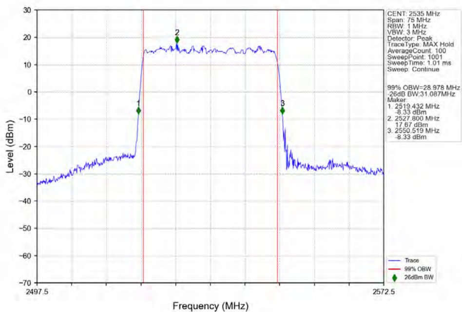
n7_15kHz_SISO_NTNV_30MHz_DFT-s-OFDM 64 QAM 2535MHz_Outer_Full_Ant1
