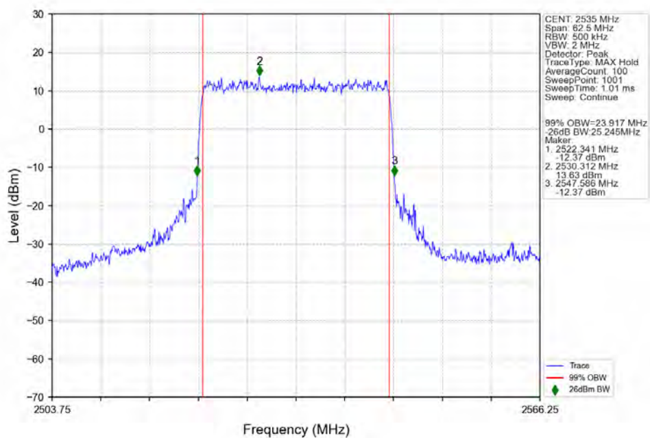
n7_15kHz_SISO_NTNV_25MHz_CP-OFDM 64 QAM 2535MHz_Outer_Full_Ant1
