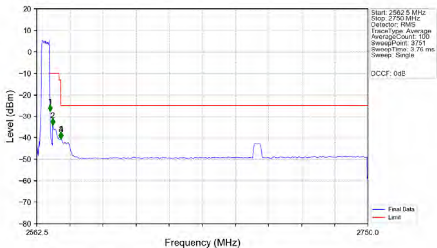
n7_15kHz_SISO_NTNV_5MHz_DFT-s-OFDM_QPSK_2567.5MHz_Outer_Full_Ant1
