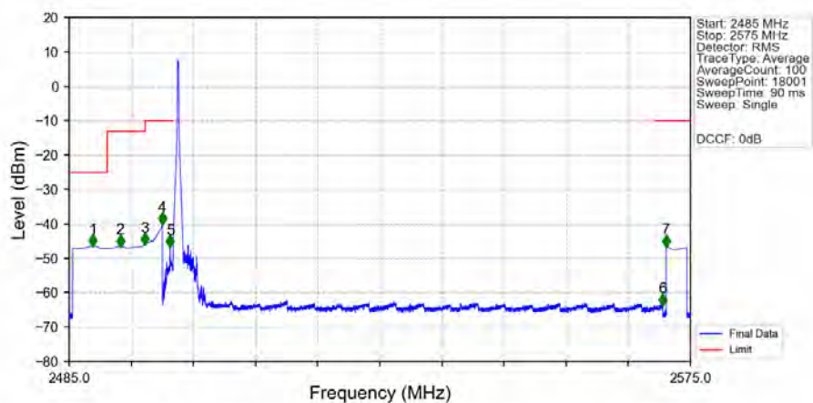
n7_15kHz_SISO_NTNV_50MHz_DFT-s-OFDM_QPSK_2525MHz_Edge_1RB_Left_Ant1
