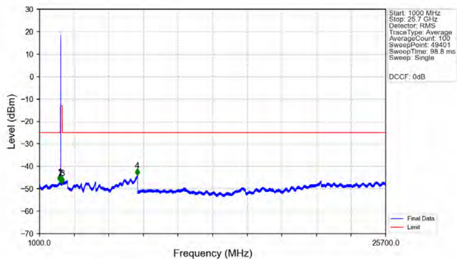
n7_15kHz_SISO_NTNV_50MHz_DFT-s-OFDM_QPSK_2535MHz_Edge_1RB_Left_Ant1
