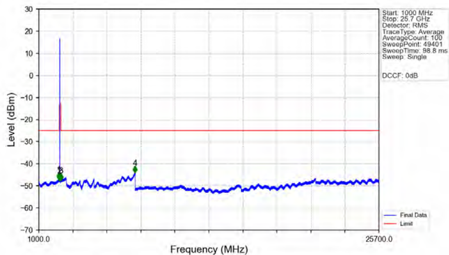
n7_15kHz_SISO_NTNV_25MHz_CP-OFDM_QPSK_2535MHz_Edge_1RB_Left_Ant1
