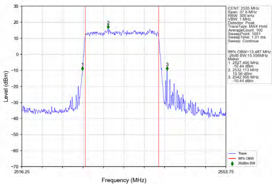
n7_15kHz_SISO_NTNV_15MHz_DFT-s-OFDM QPSK_2535MHz_Outer_Full_Ant1
