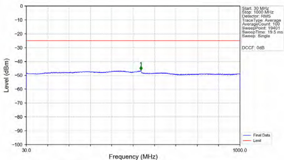
n7_15kHz_SISO_NTNV_25MHz_DFT-s-OFDM_QPSK_2535MHz_Edge_1RB_Left_Ant1
