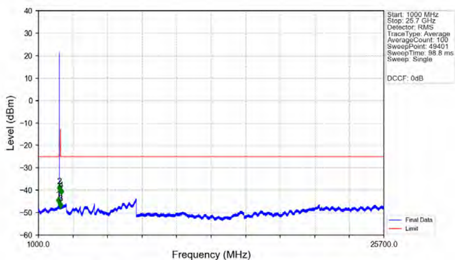
n7_15kHz_SISO_NTNV_5MHz_DFT-s-OFDM_QPSK_2502.5MHz_Edge_1RB_Left_Ant1
