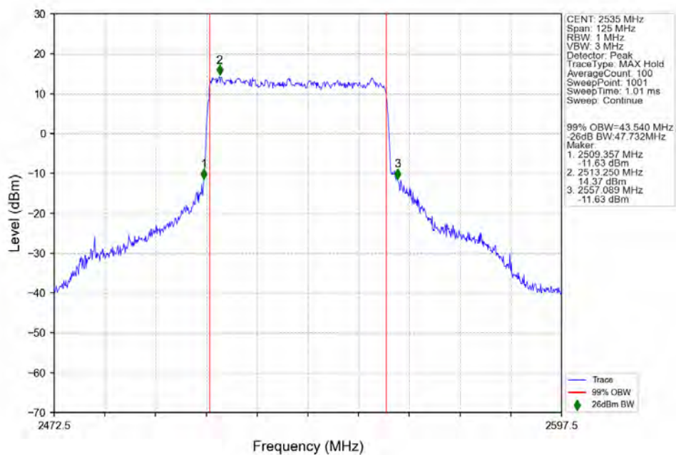
n7_15kHz_SISO_NTNV_50MHz_CP-OFDM 64 QAM 2535MHz_Outer_Full_Ant1
