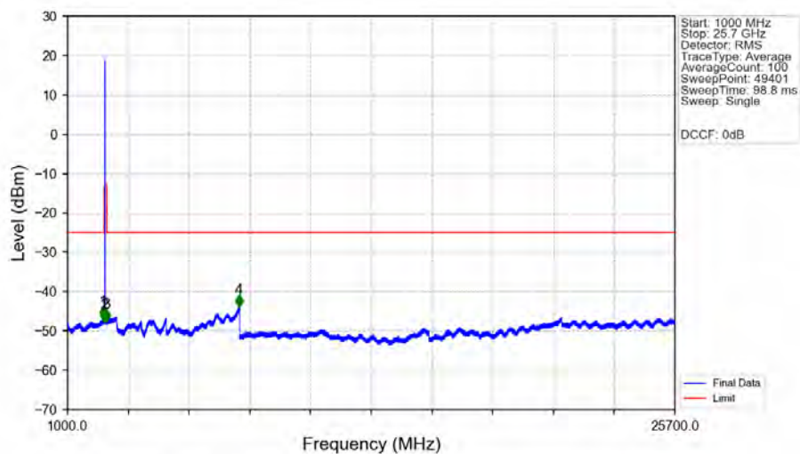
n7_15kHz_SISO_NTNV_25MHz_DFT-s-OFDM_QPSK_2535MHz_Edge_1RB_Left_Ant1
