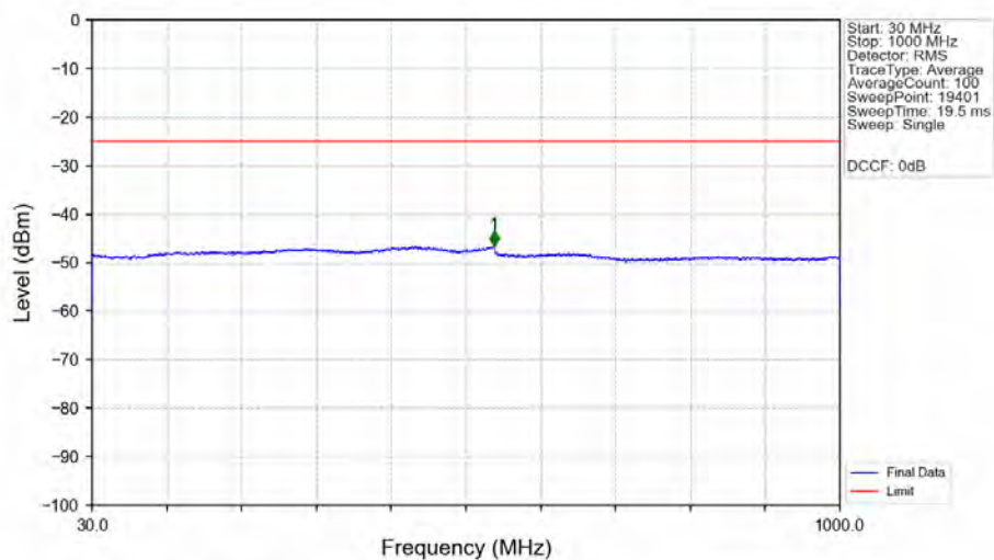
n7_15kHz_SISO_NTNV_25MHz_DFT-s-OFDM_QPSK_2512.5MHz_Edge_1RB_Left_Ant1
