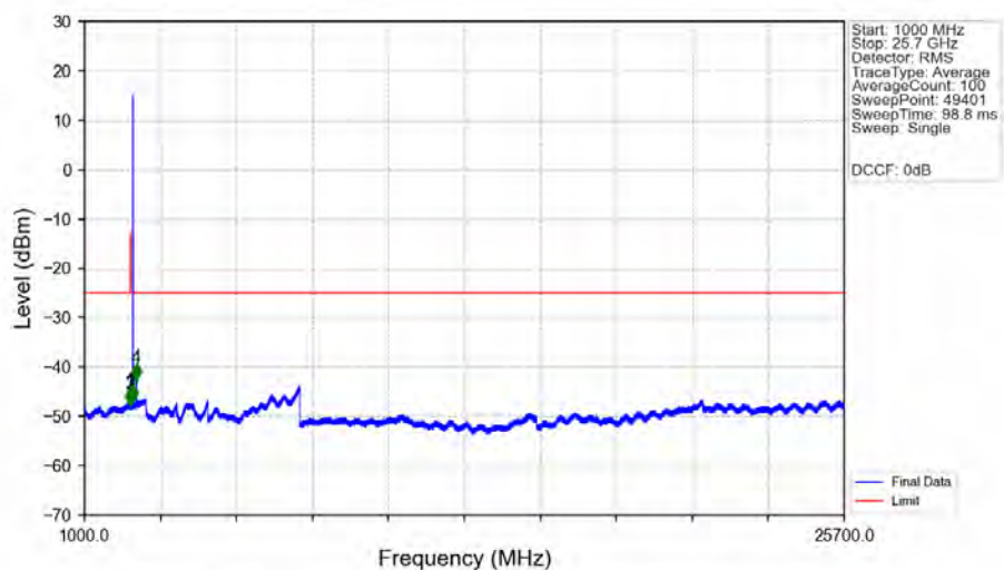
n7_15kHz_SISO_NTNV_5MHz_CP-OFDM_QPSK_2567.5MHz_Edge_1RB_Right_Ant1
