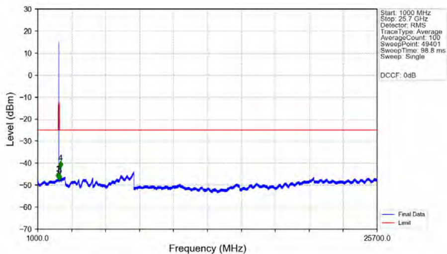
n7_15kHz_SISO_NTNV_5MHz_CP-OFDM_QPSK_2535MHz_Edge_1RB_Left_Ant1
