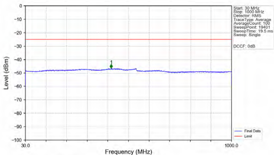
n7_15kHz_SISO_NTNV_5MHz_CP-OFDM_QPSK_2535MHz_Edge_1RB_Left_Ant1
