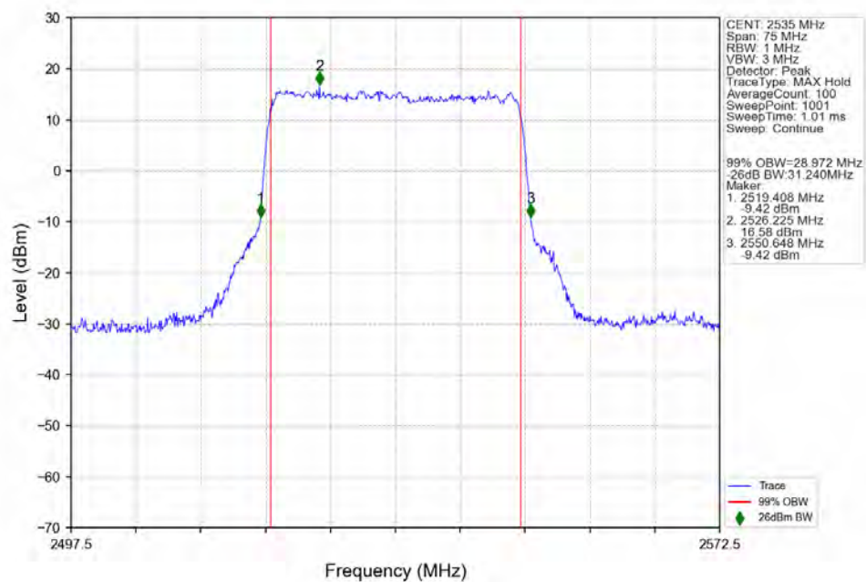
n7_15kHz_SISO_NTNV_30MHz_CP-OFDM_QPSK_2535MHz_Outer_Full_Ant1
