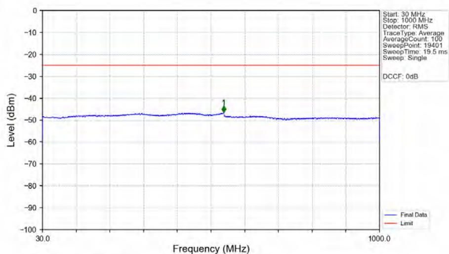
n7_15kHz_SISO_NTNV_50MHz_DFT-s-OFDM_QPSK_2535MHz_Edge_1RB_Left_Ant1
