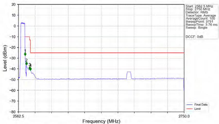
n7_15kHz_SISO_NTNV_5MHz_CP-OFDM_QPSK_2567.5MHz_Outer_Full_Ant1
