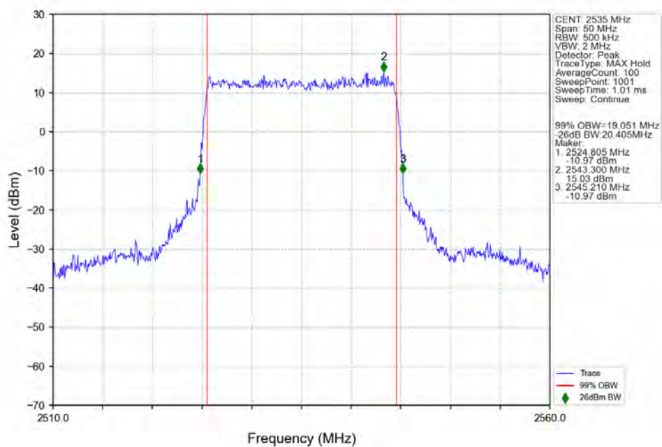
n7_15kHz_SISO_NTNV_20MHz_CP-OFDM 64 QAM 2535MHz_Outer_Full_Ant1
