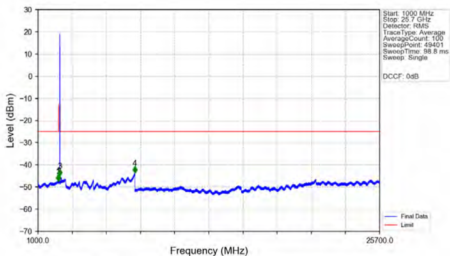
n7_15kHz_SISO_NTNV_25MHz_CP-OFDM_QPSK_2557.5MHz_Edge_1RB_Right_Ant1
