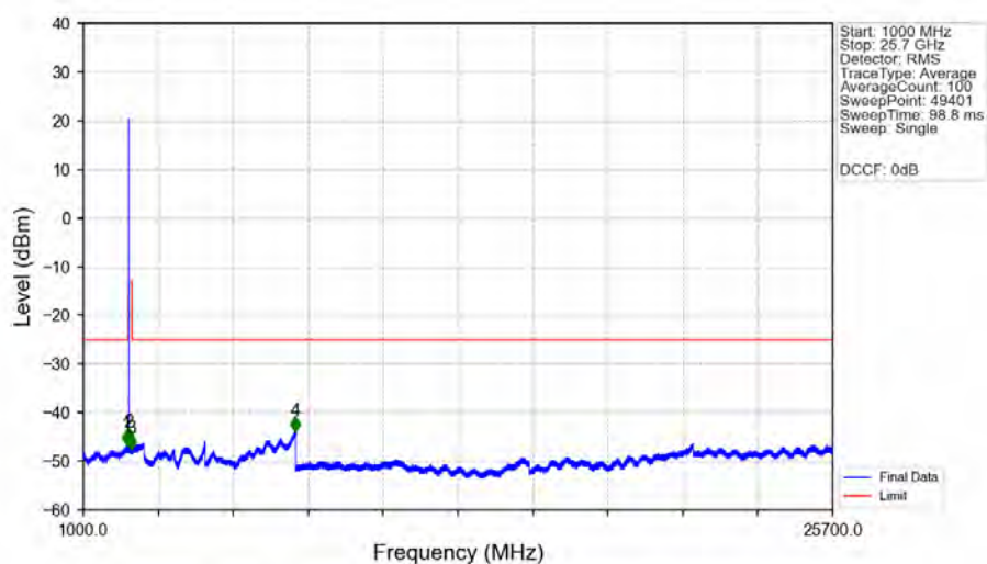
n7_15kHz_SISO_NTNV_25MHz_DFT-s-OFDM_PI/2_BPSK_2512.5MHz_Edge_1RB_Left_Ant1
