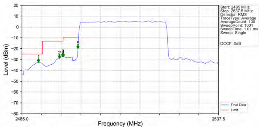
n7_15kHz_SISO_NTNV_25MHz_DFT-s-OFDM_PI/2_BPSK_2512.5MHz_Outer_Full_Ant1
