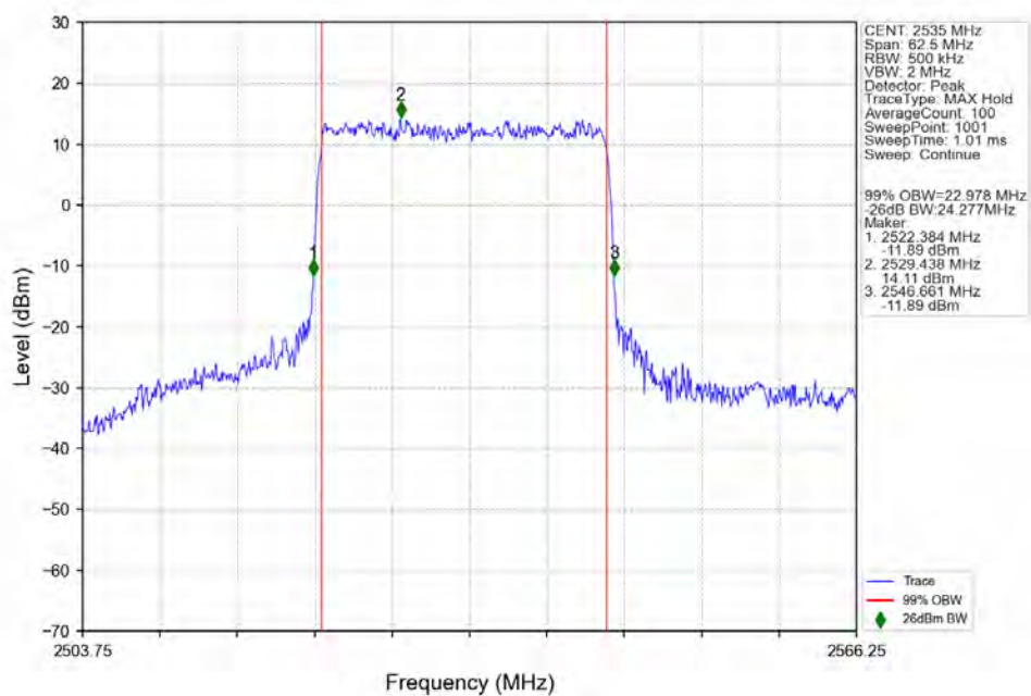
n7_15kHz_SISO_NTNV_25MHz_DFT-s-OFDM 64 QAM 2535MHz_Outer_Full_Ant1
