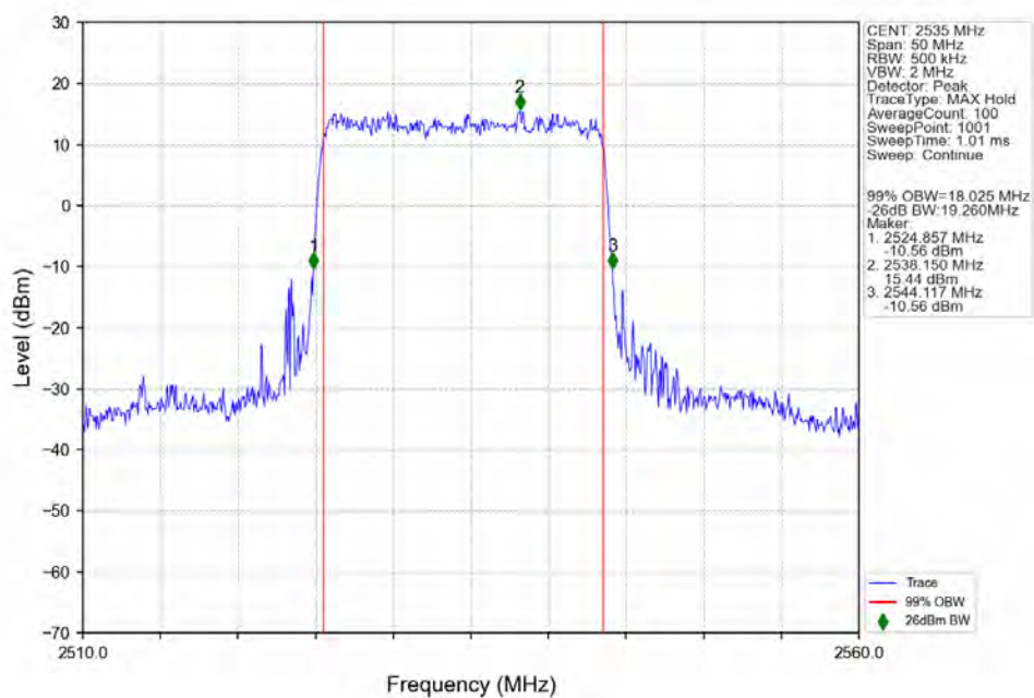
n7_15kHz_SISO_NTNV_20MHz_DFT-s-OFDM 64 QAM 2535MHz_Outer_Full_Ant1
