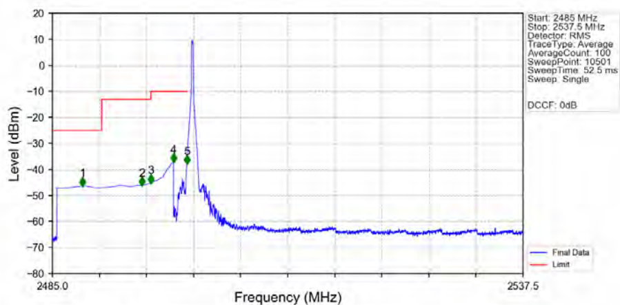
n7_15kHz_SISO_NTNV_25MHz_CP-OFDM_QPSK_2512.5MHz_Edge_1RB_Left_Ant1
