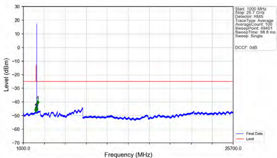
n7_15kHz_SISO_NTNV_5MHz_DFT-s-OFDM_PI/2_BPSK_2567.5MHz_Edge_1RB_Right_Ant1
