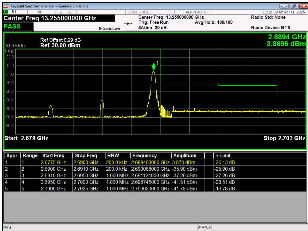
Band41 QPSK BW=10MHz Channel=41540 RB Size=50 Position=#0
