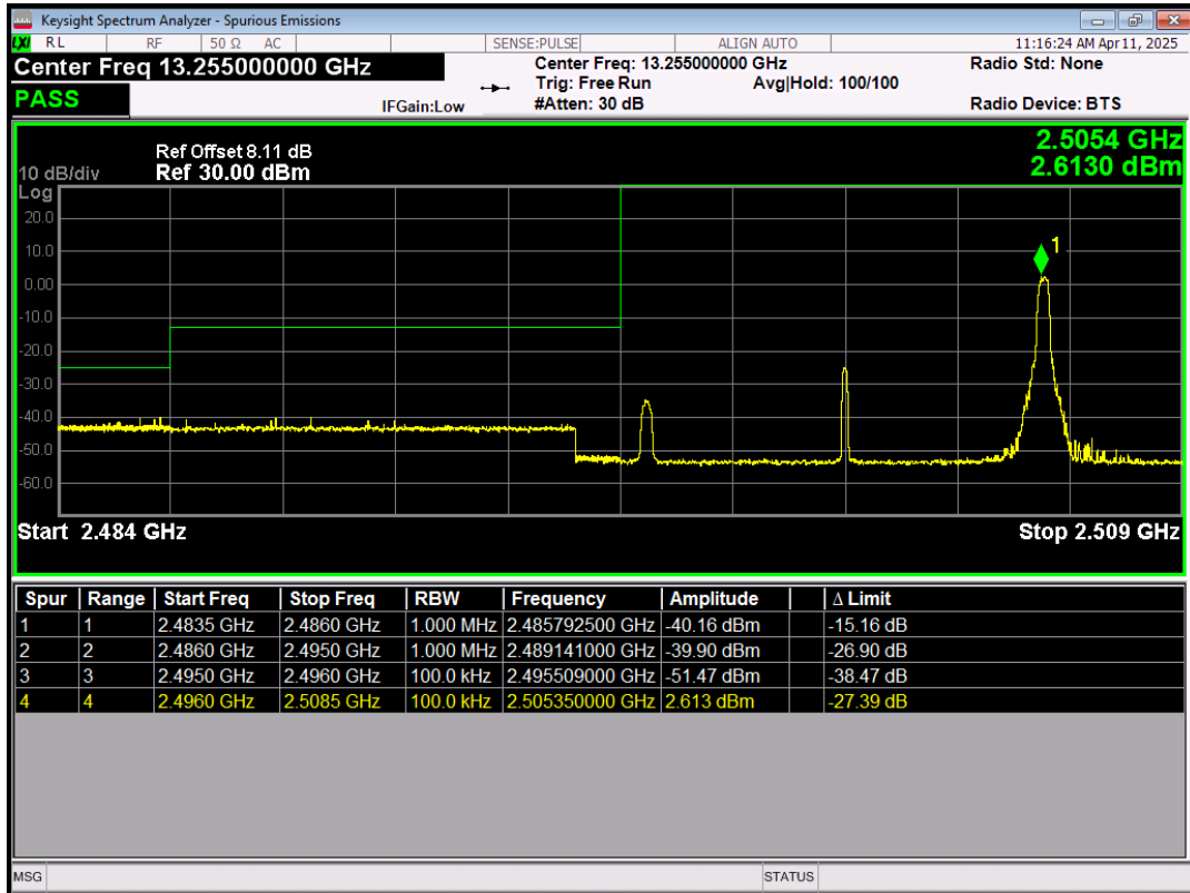
Band41 16QAM BW=10MHz Channel=39700 RB Size=50 Position=#0
