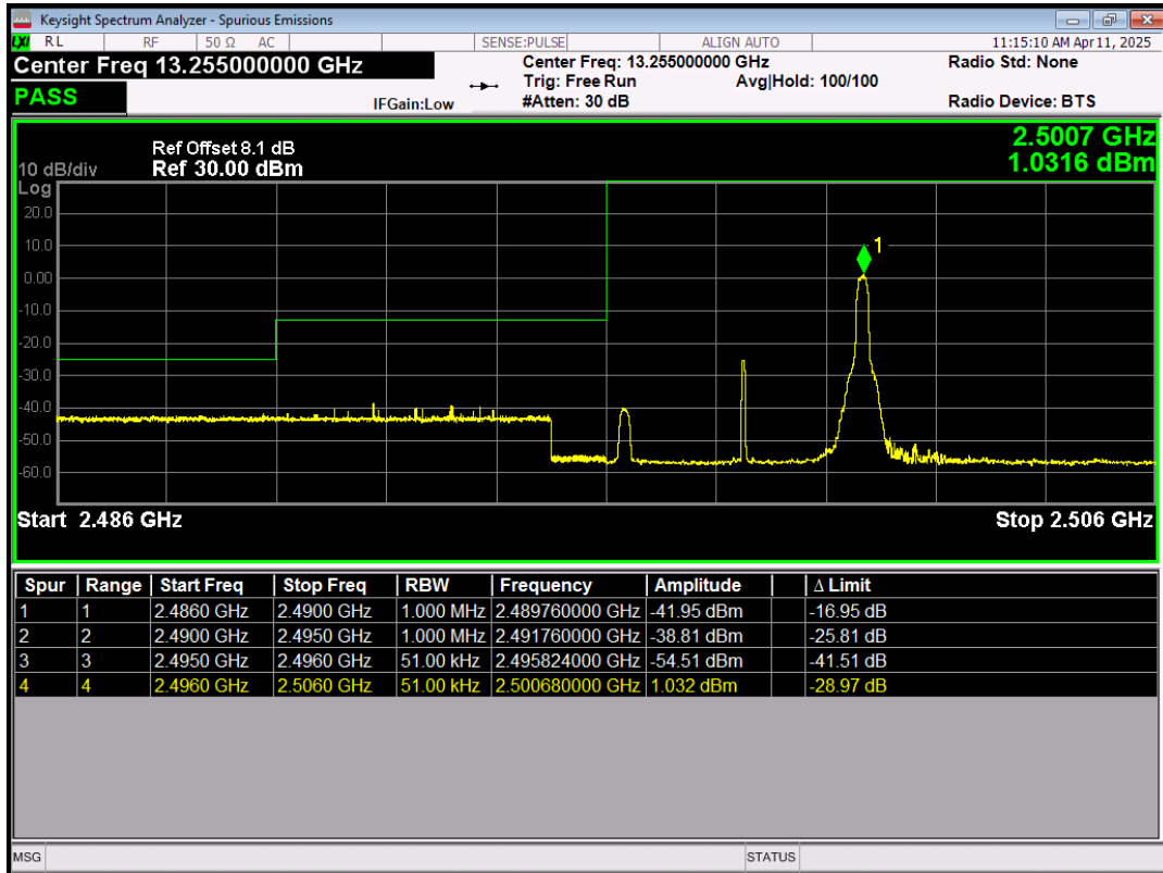
Band41 16QAM BW=5MHz Channel=39675 RB Size=25 Position=#0
