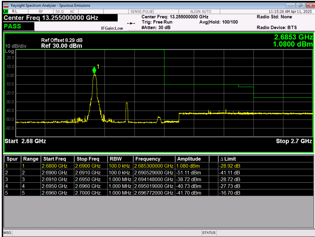
Band41 QPSK BW=5MHz Channel=41565 RB Size=1 Position=#Max
