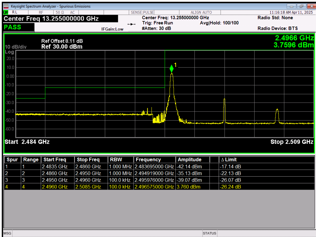
Band41 16QAM BW=10MHz Channel=39700 RB Size=1 Position=#Max
