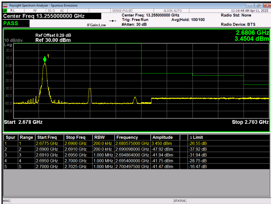
Band41 16QAM BW=10MHz Channel=41540 RB Size=1 Position=#Max
