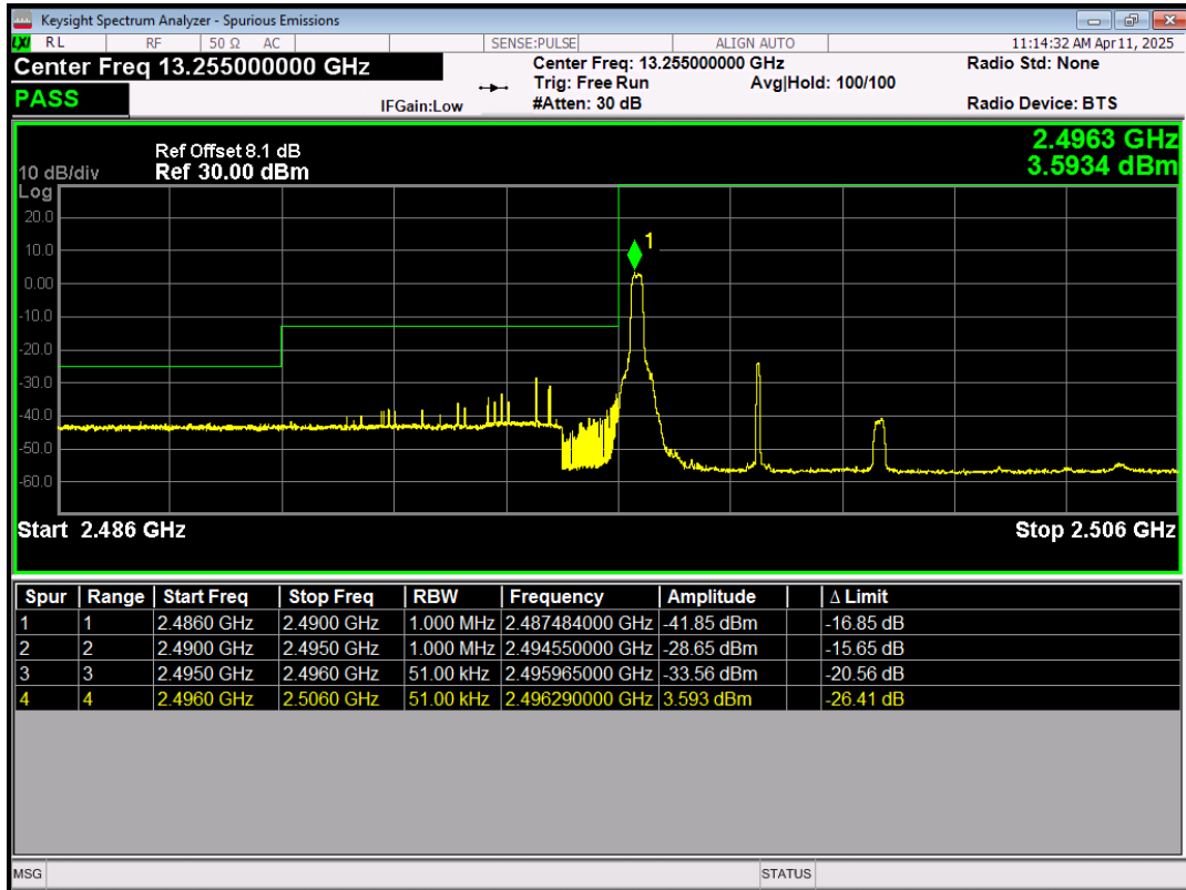
Band41 QPSK BW=5MHz Channel=39675 RB Size=1 Position=#Max
