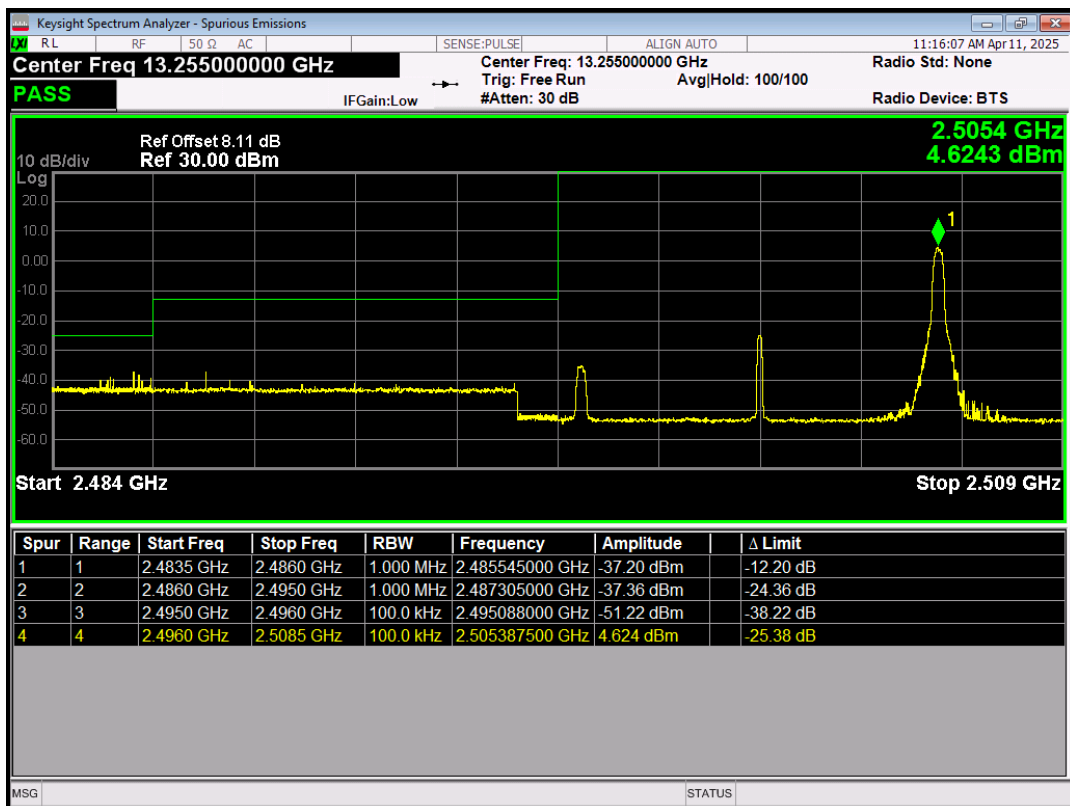
Band41 QPSK BW=10MHz Channel=39700 RB Size=50 Position=#0
