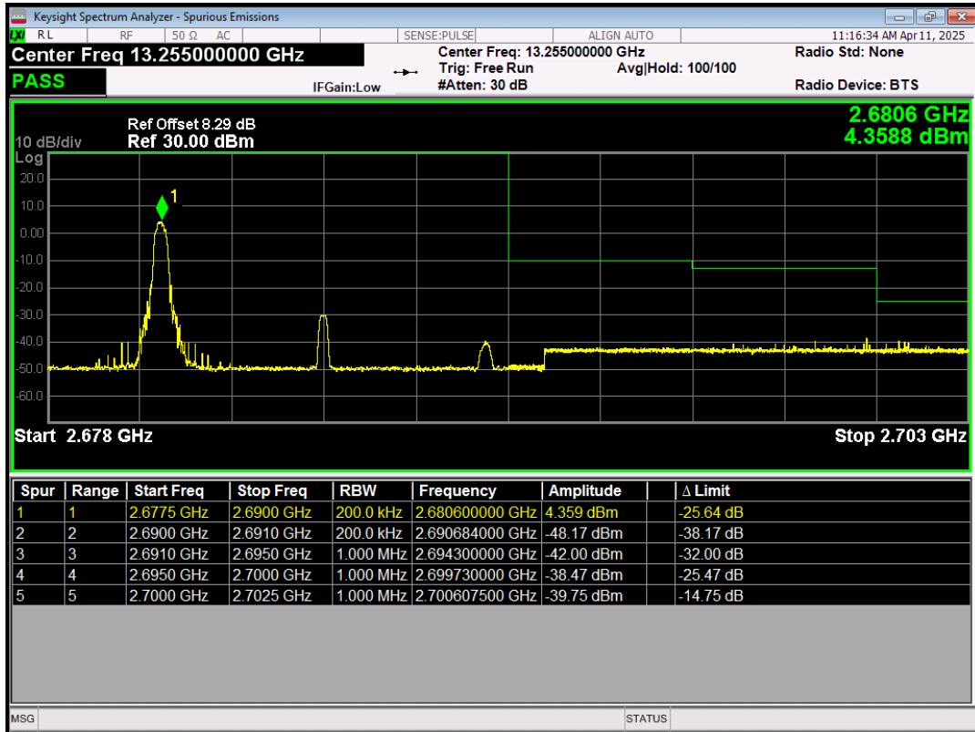
Band41 QPSK BW=10MHz Channel=41540 RB Size=1 Position=#Max
