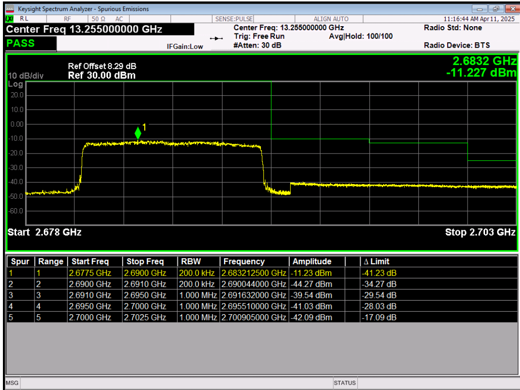
Band41 16QAM BW=10MHz Channel=41540 RB Size=1 Position=#0
