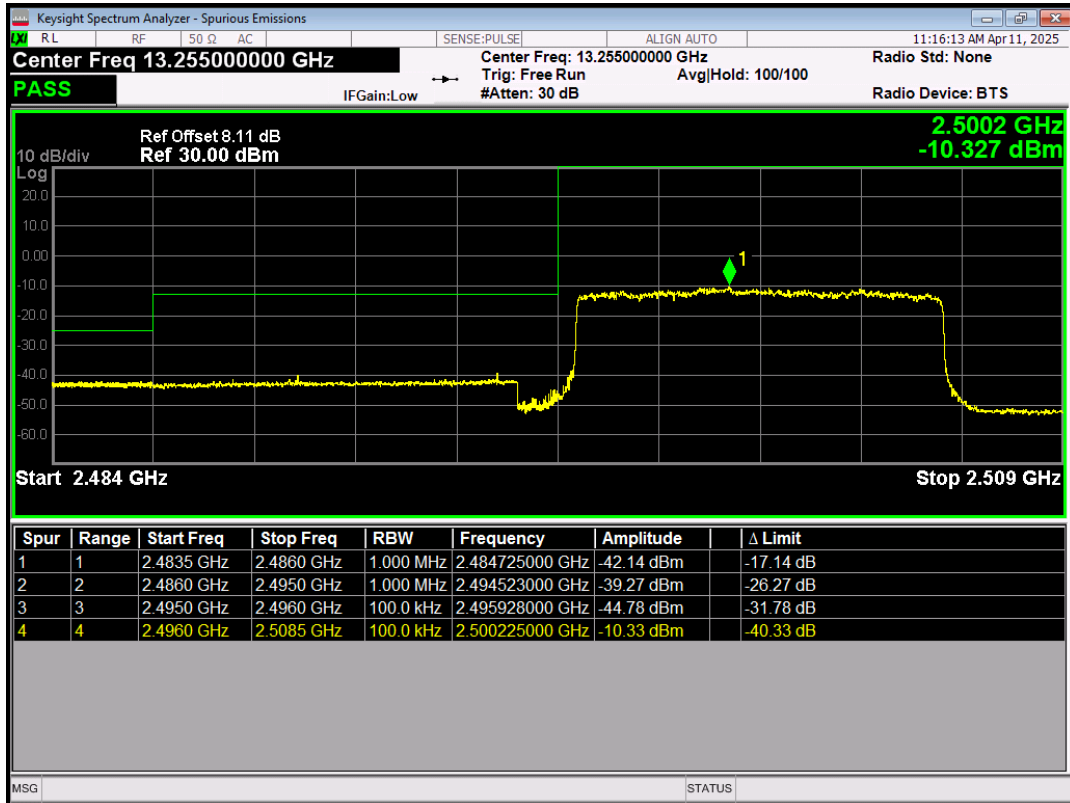
Band41 16QAM BW=10MHz Channel=39700 RB Size=1 Position=#0
