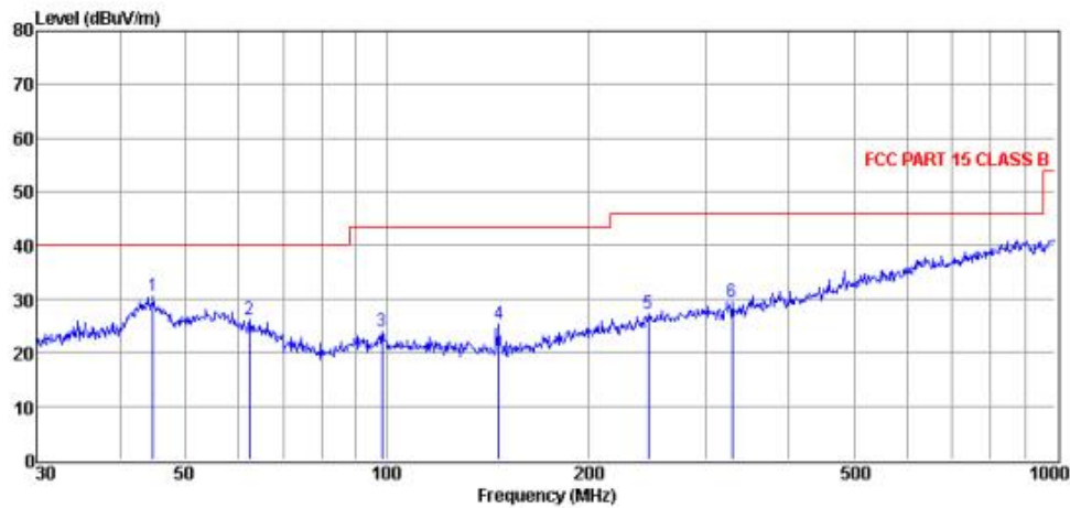
Quasi-peak measurement:
