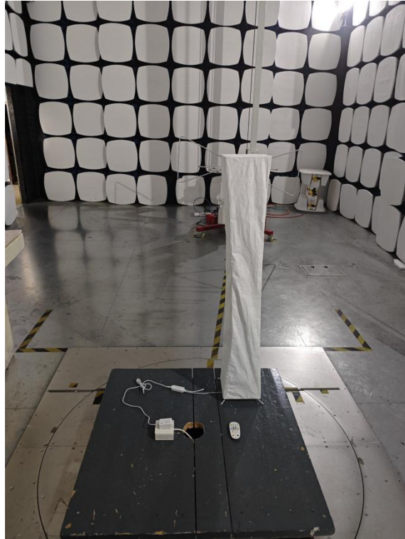
Radiated Emission (30MHz-1GHz)
