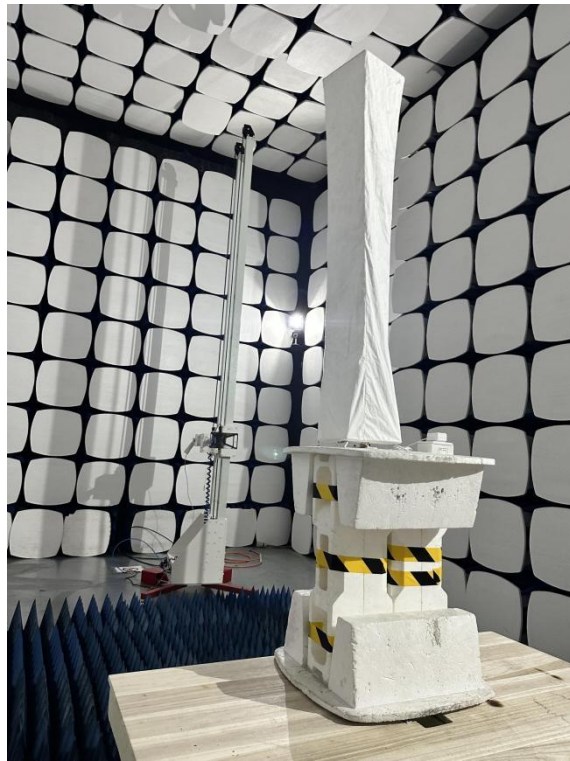
Radiated Emission (Above 1GHz)
