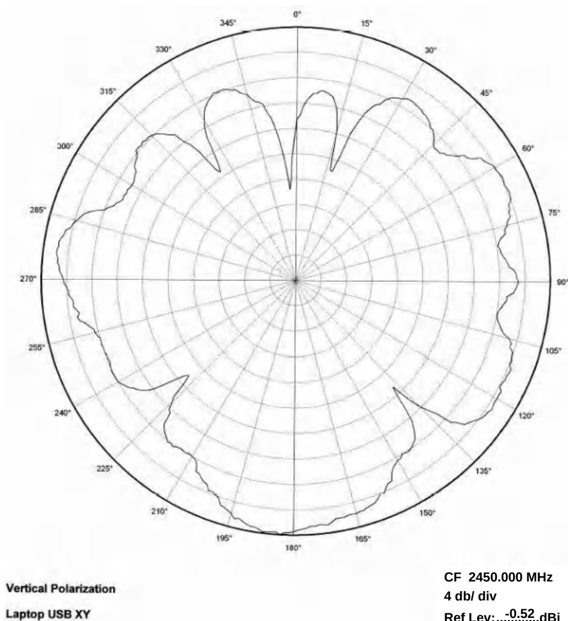
Figure10 : USB Dongle in Laptop XY Plane
