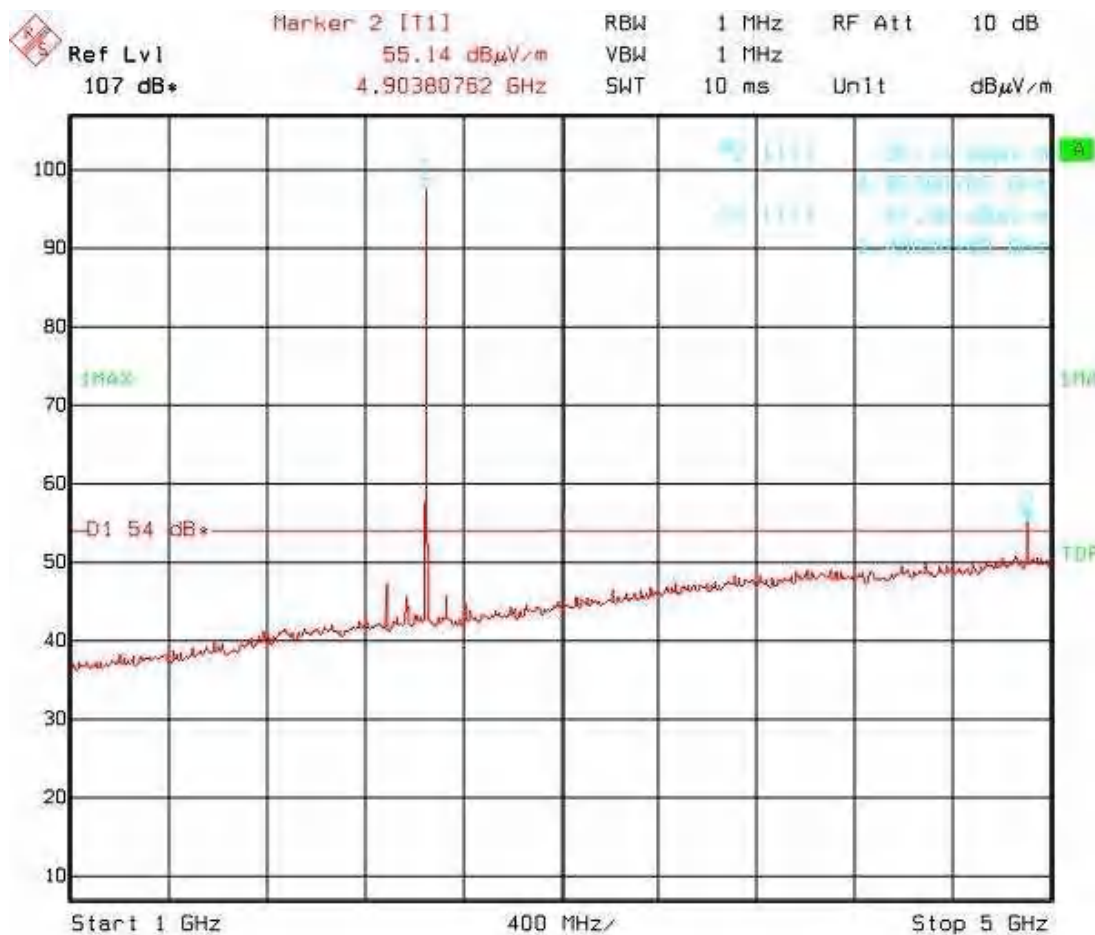
Figure 17: TX Spurious Emission 1 – 5 GHz
