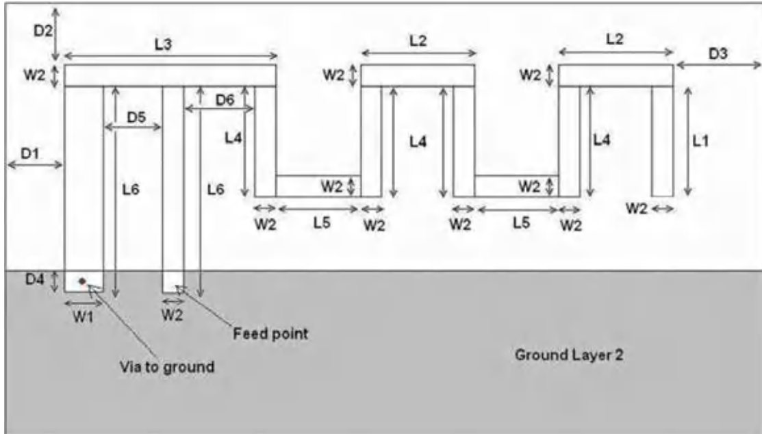
Figure 3: Antenna Dimensions
