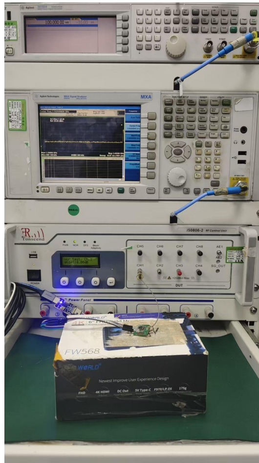
RF Conducted test setup photos
