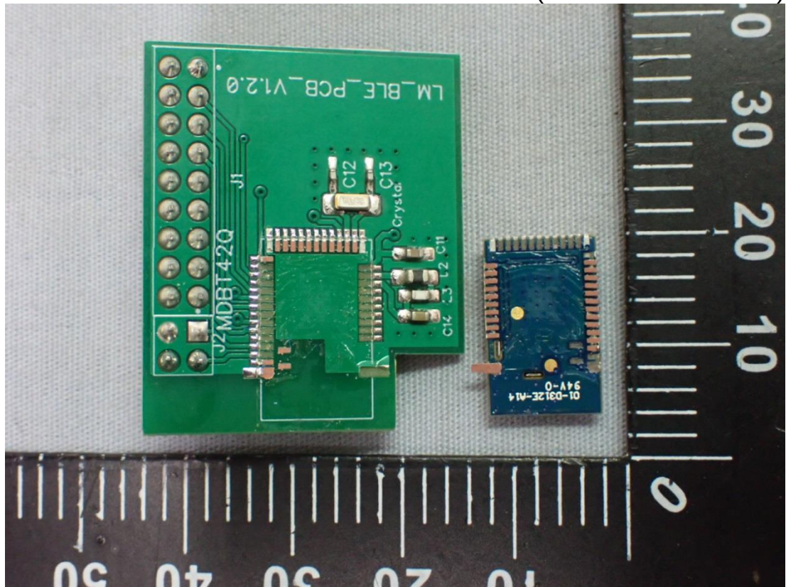
Figure 17 Internal (Removed RF Module)
