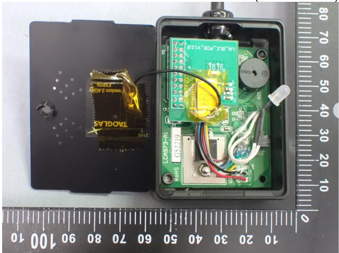
Figure 13 Internal (Removed Cover)
