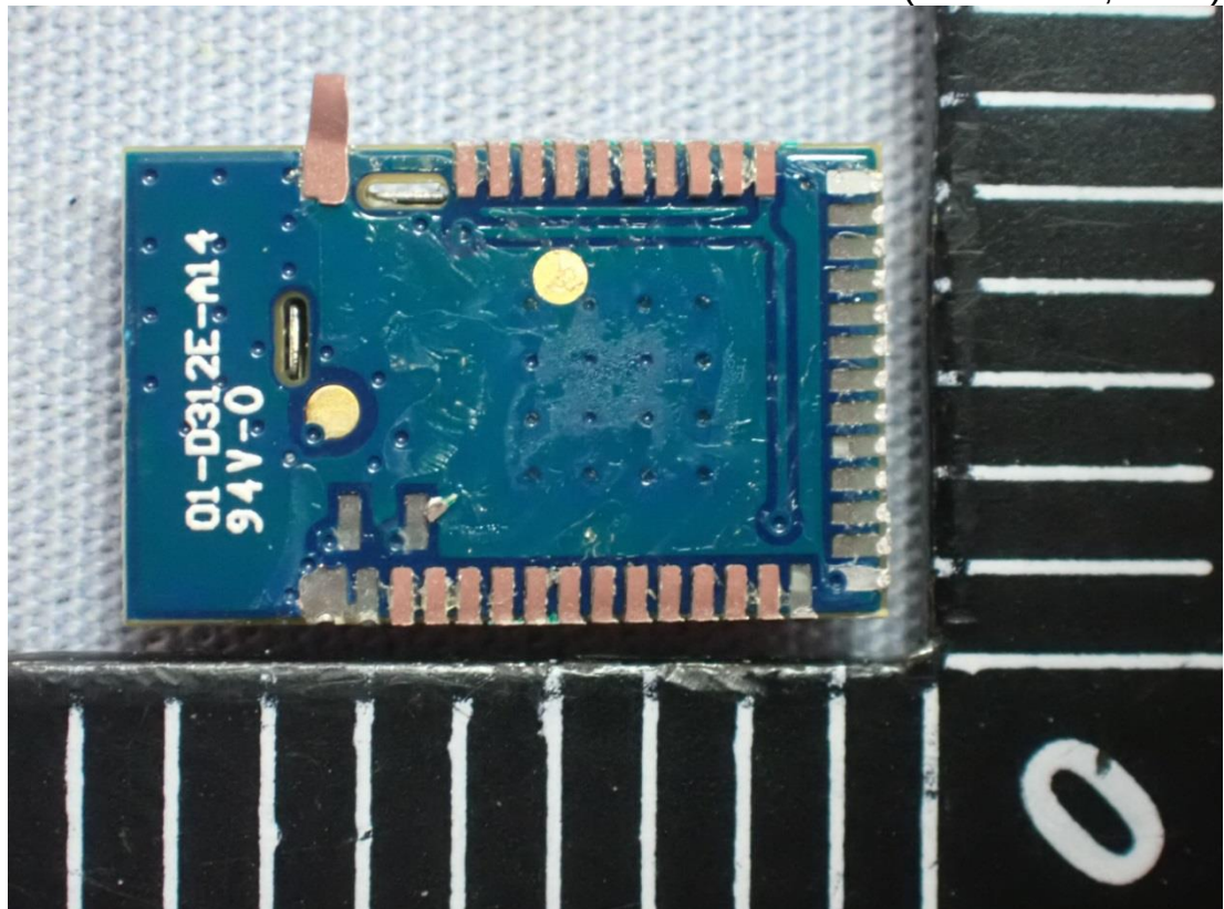
Figure 18 Internal (RF Module, Back)
