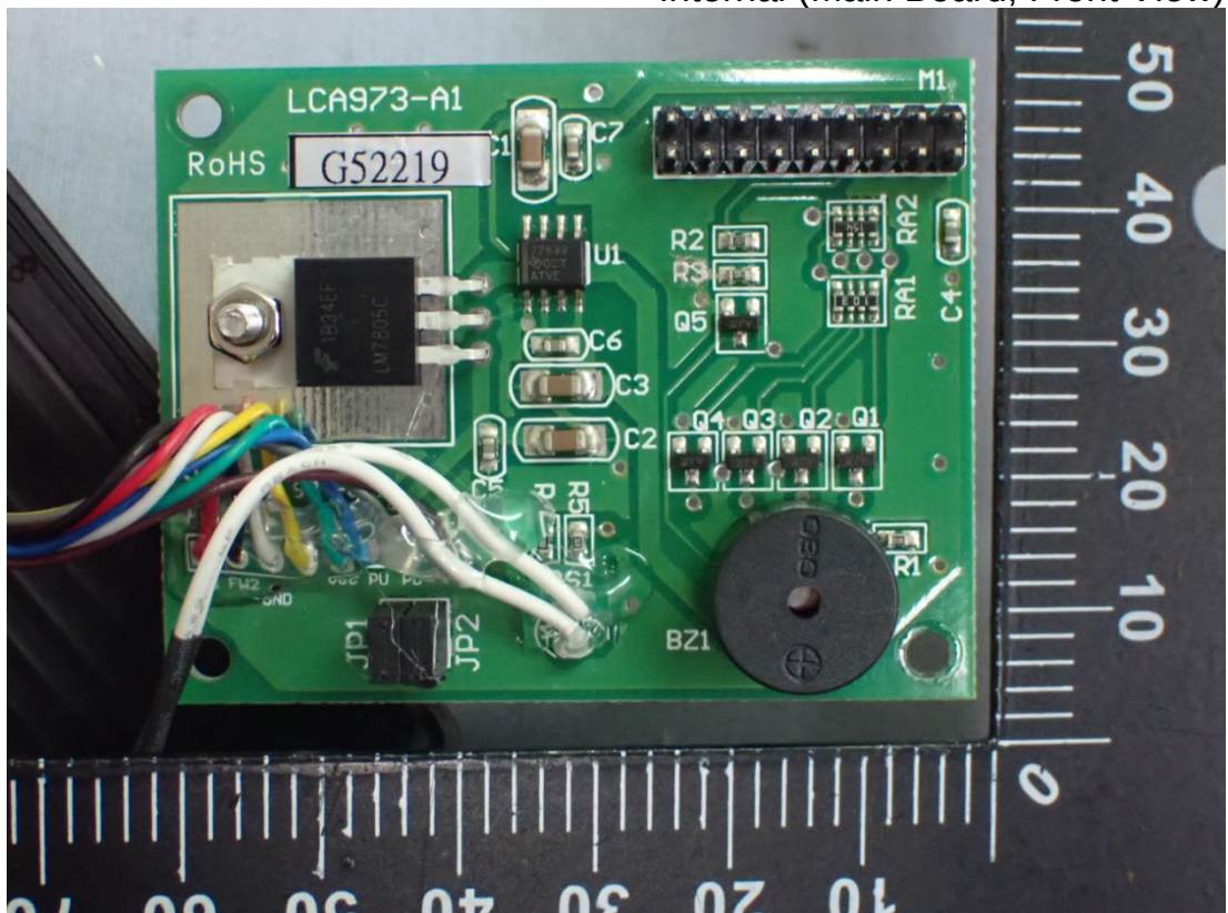
Figure 22 Internal (Main Board, Front View)
