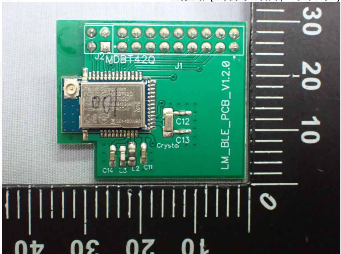
Figure 16 Internal (Module Board, Front View)
