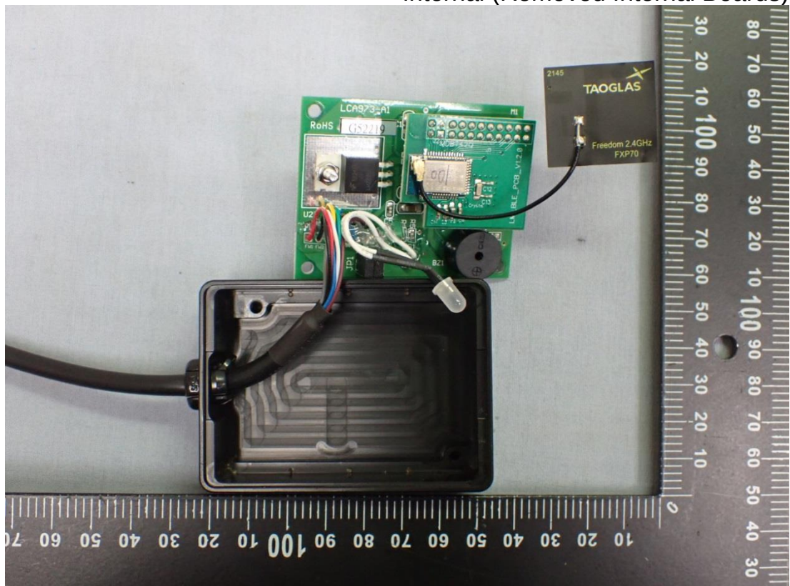
Figure 14 Internal (Removed Internal Boards)
