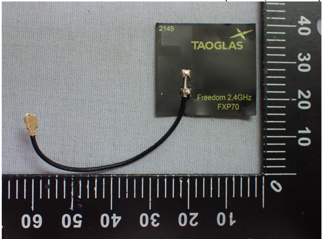
Figure 20 Internal (RF ANT, Front View)
