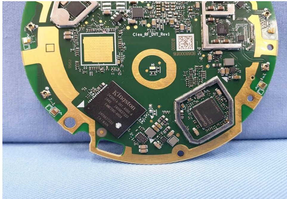
EUT Photo (10) _5G Filter_ Skyworks SKY85905-88
