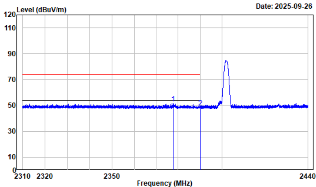
Left Band edge_Horizontal_BT_DH5
