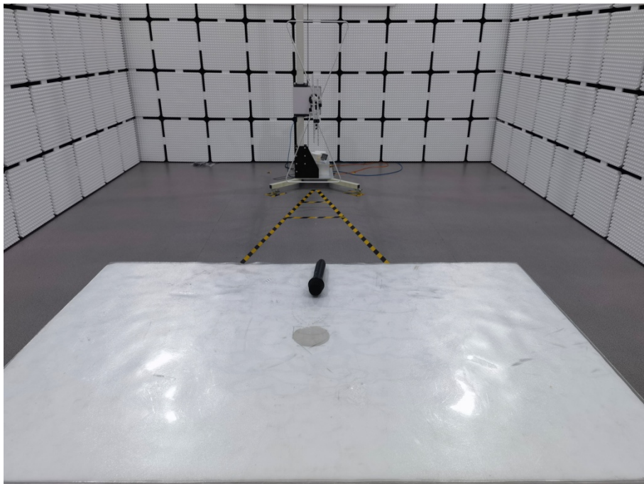
Test Model: C-9200 Radiated Emissions
