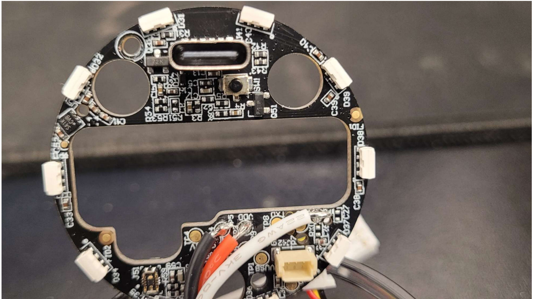
Top View #3 of PCB
