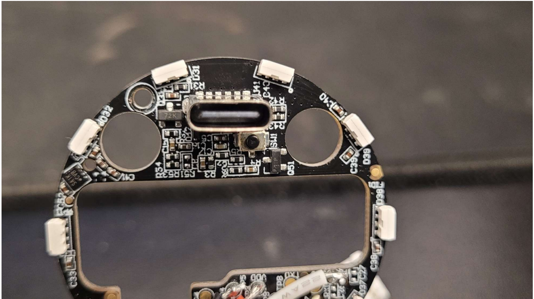
Top View #1 of PCB
