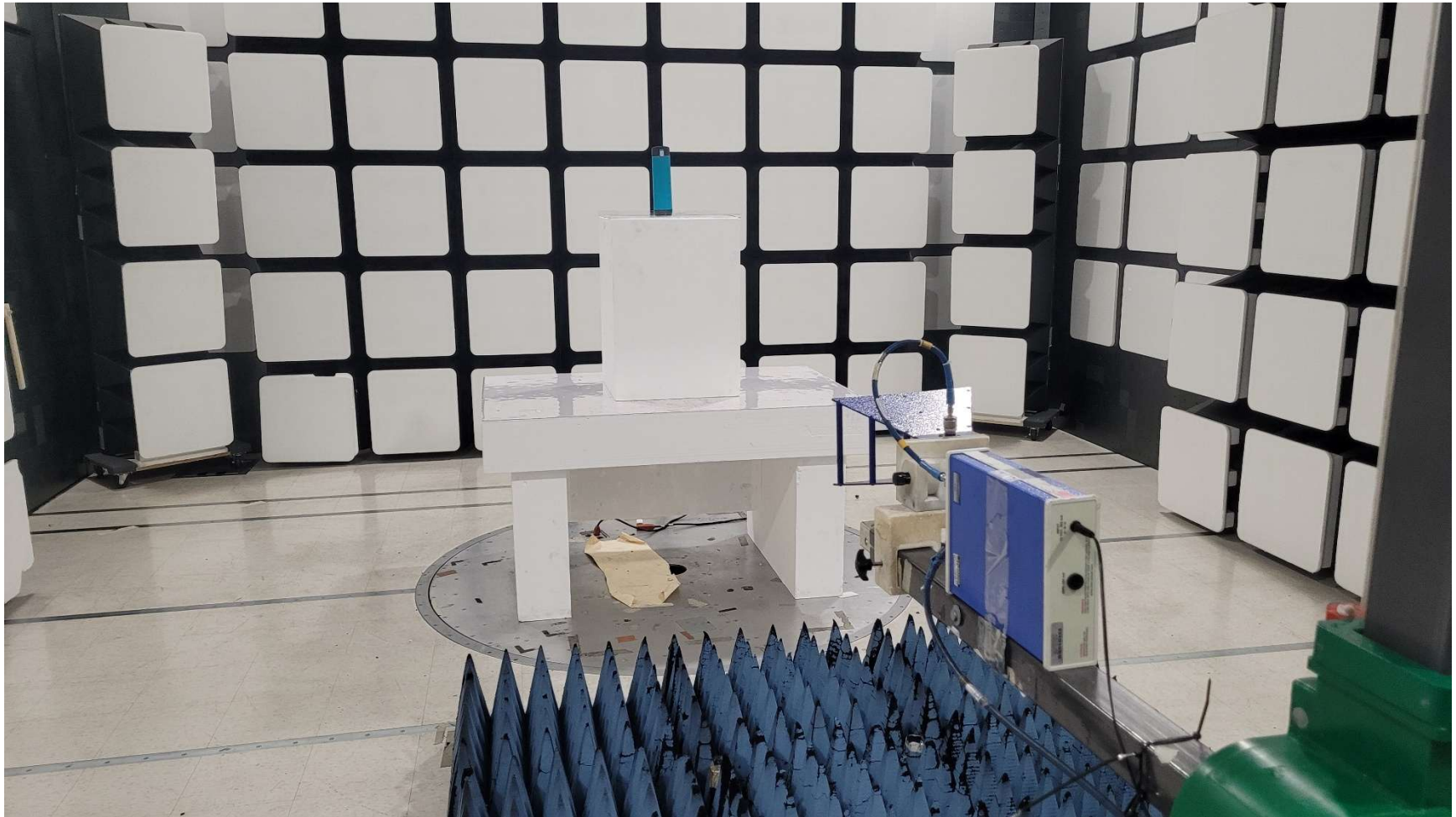
Normal Mode Radiated Emissions
