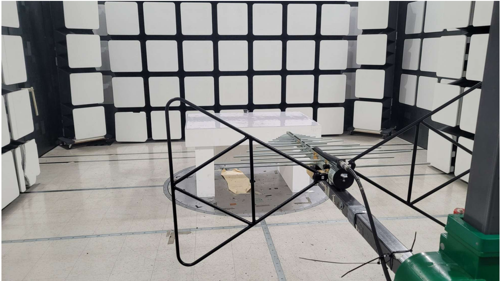
Charging Mode Radiated Emissions
