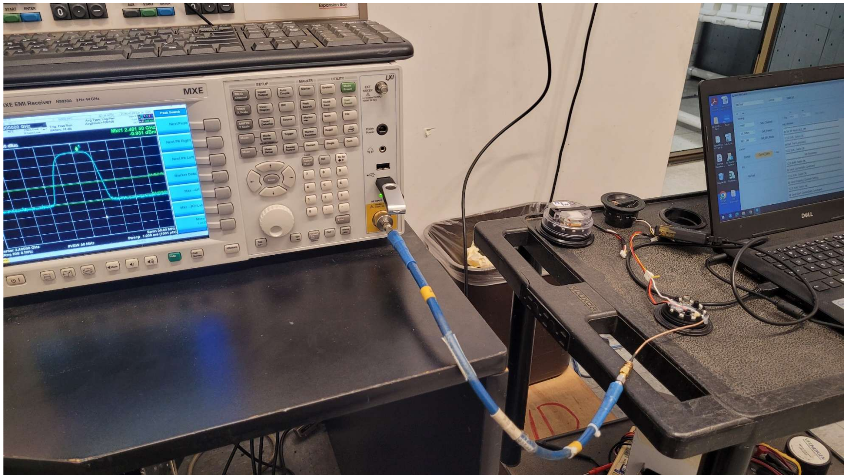
Direct RF Conducted Measurements
