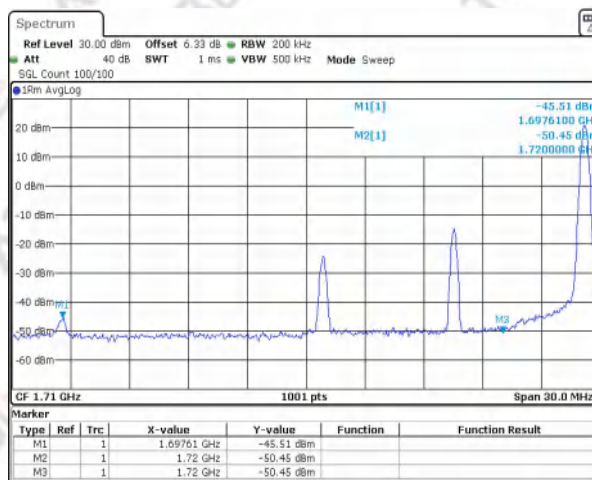
Band4 QPSK BW=15MHz Channel=20025 RB Size=1 Position=#Max NVNT
