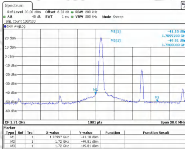
Band4 QPSK BW=15MHz Channel=20025 RB Size=1 Position=#0 NVNT
