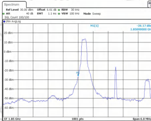
Band2 QPSK BW=3MHz Channel=18615 RB Size=1 Position=#0 NVNT
