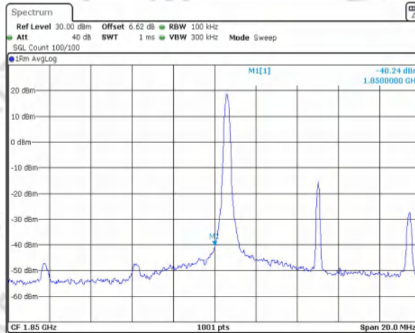
Band2 QPSK BW=10MHz Channel=18650 RB Size=1 Position=#0 NVNT
