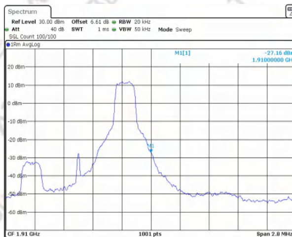
Band2 QPSK BW=1.4MHz Channel=19193 RB Size=1 Position=#Max NVNT
