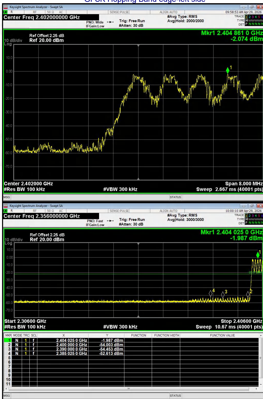
GFSK Hopping Band edge-left side
