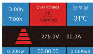
Over Voltage
