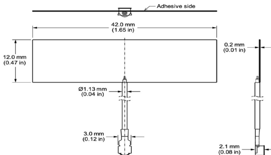
Figure 1. ANT-W63-FPC2-UFL-100 Dimensions
