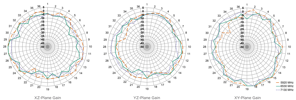
Figure 7. Radiation Patterns for ANT-W63-FPC2-UFL-100 Antenna
