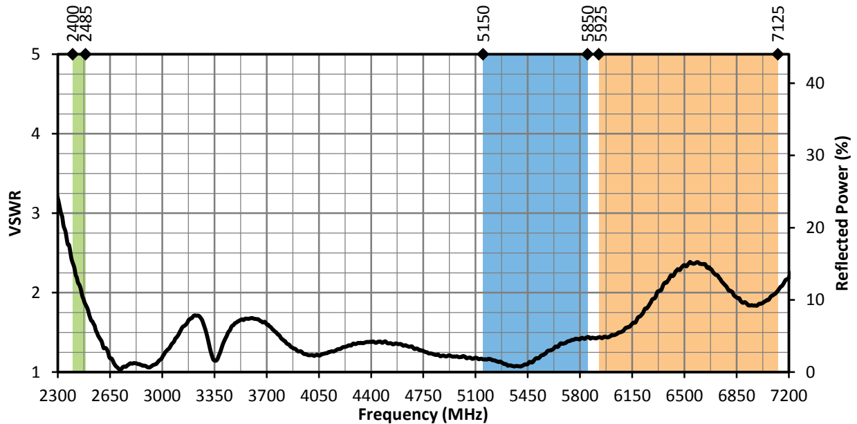
Figure 2. W63-FPC2 Antenna VSWR with Frequency Band Highlights
