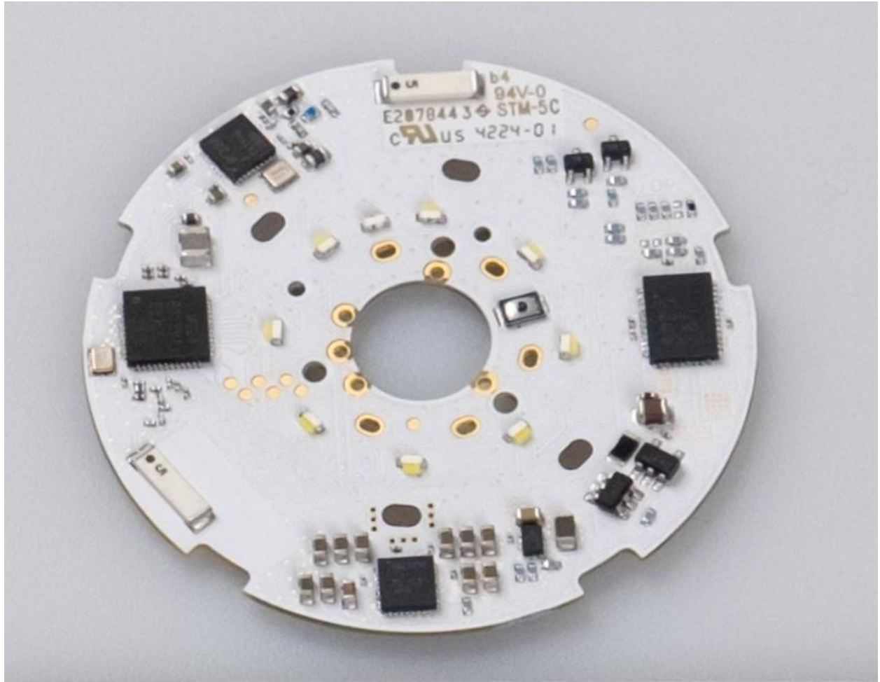
Figure 1: Top View
