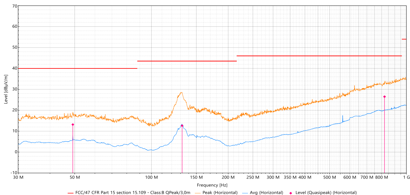
#51(30 MHz-1 GHz), Horizontal
