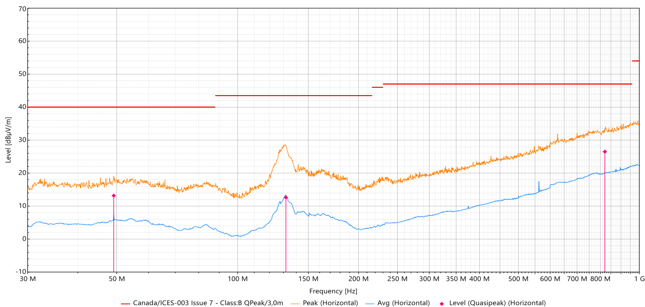
#58(30 MHz-1 GHz), Horizontal
