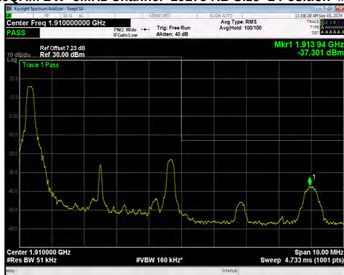
Band2 16QAM BW=5MHz Channel=19175 RB Size=1 Position=#Max Extended
