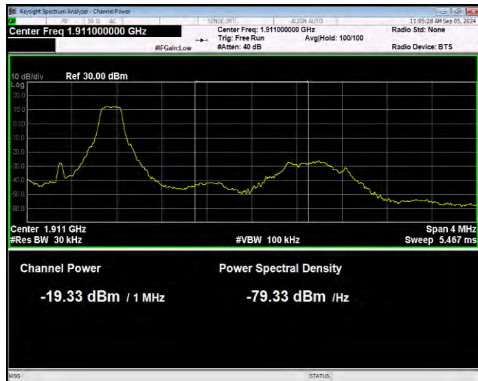
Band2 QPSK BW=1.4MHz Channel=19193 RB Size=1 Position=#Max Normal
