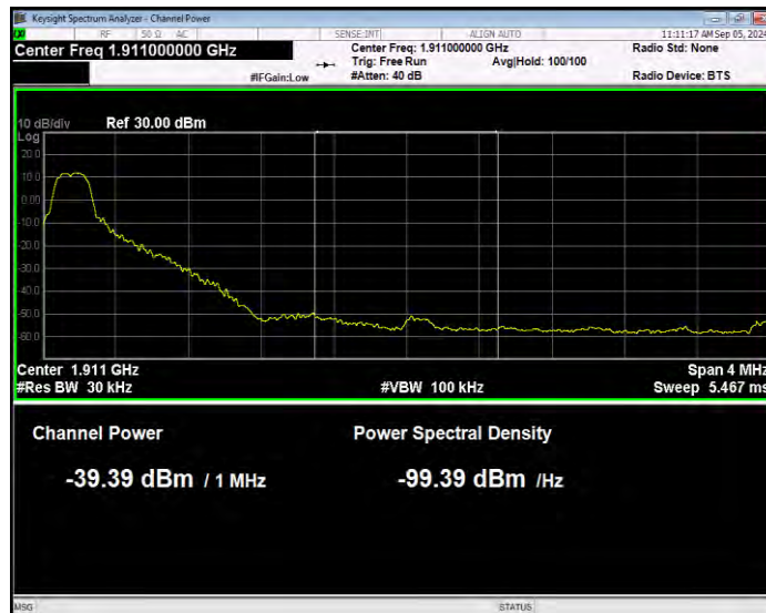
Band2 16QAM BW=15MHz Channel=19125 RB Size=1 Position=#Max Normal
