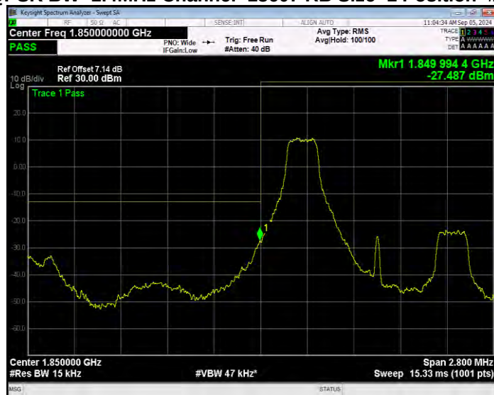
Band2 QPSK BW=1.4MHz Channel=18607 RB Size=1 Position=#Max Extended
