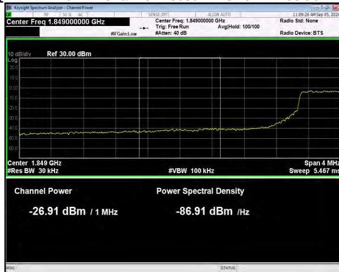
Band2 16QAM BW=10MHz Channel=18650 RB Size=27 Position=#0 Normal
