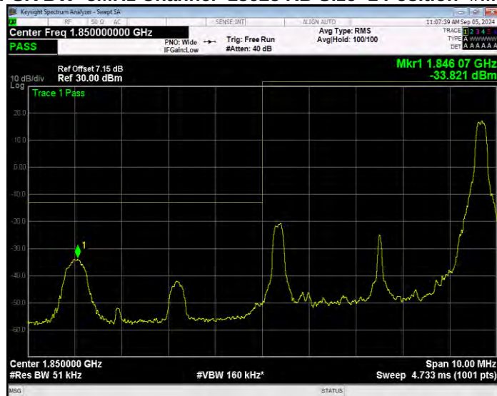
Band2 QPSK BW=5MHz Channel=18625 RB Size=25 Position=#0 Extended
