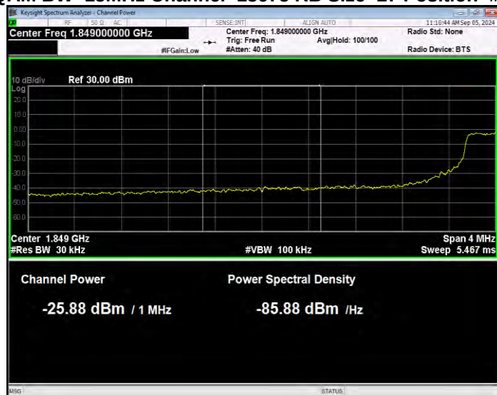
Band2 16QAM BW=15MHz Channel=18675 RB Size=27 Position=#0 Normal
