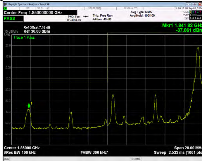
Band2 16QAM BW=10MHz Channel=18650 RB Size=27 Position=#0 Extended
