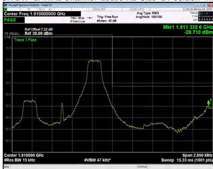
Band2 QPSK BW=1.4MHz Channel=19193 RB Size=6 Position=#0 Extended
