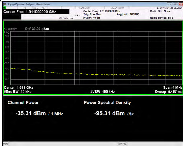
Band2 16QAM BW=10MHz Channel=19150 RB Size=27 Position=#0 Normal
