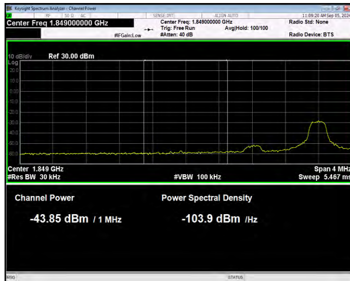
Band2 16QAM BW=10MHz Channel=18650 RB Size=1 Position=#Max Normal
