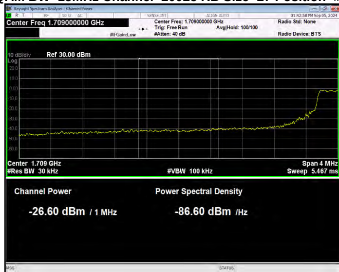
Band4 16QAM BW=15MHz Channel=20025 RB Size=27 Position=#0 Normal
