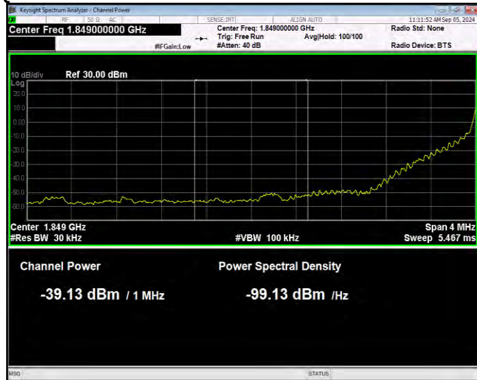
Band2 16QAM BW=20MHz Channel=18700 RB Size=1 Position=#0 Normal
