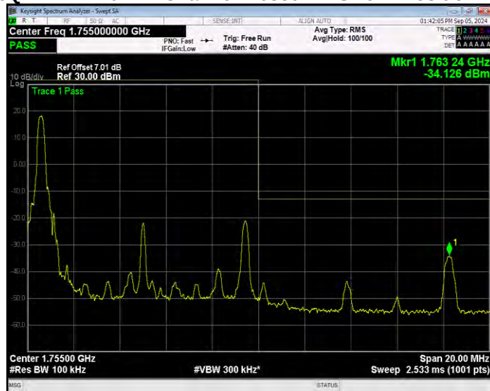
Band4 16QAM BW=10MHz Channel=20350 RB Size=1 Position=#Max Extended
