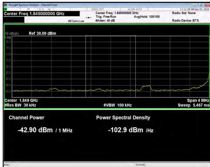
Band2 QPSK BW=20MHz Channel=18700 RB Size=1 Position=#Max Normal
