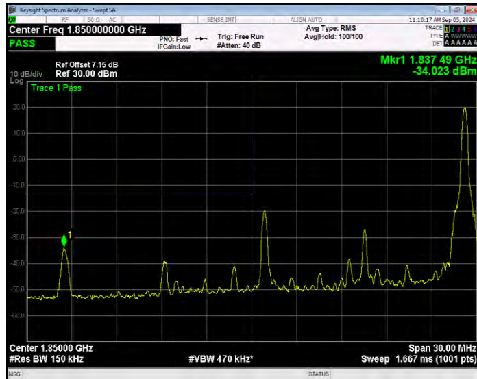
Band2 QPSK BW=15MHz Channel=18675 RB Size=75 Position=#0 Extended
