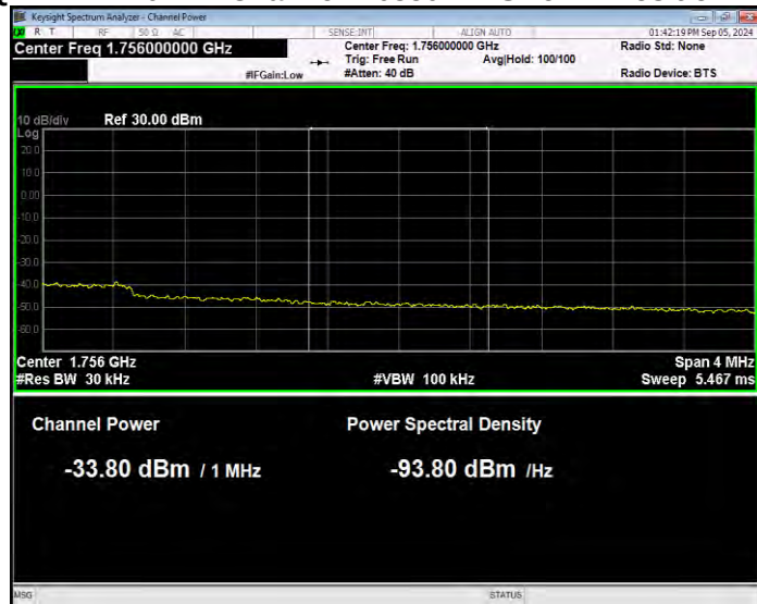
Band4 16QAM BW=10MHz Channel=20350 RB Size=27 Position=#0 Normal
