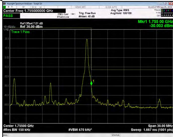
Band4 16QAM BW=15MHz Channel=20325 RB Size=27 Position=#0 Extended
