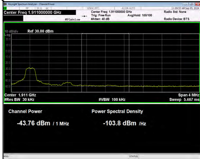
Band2 16QAM BW=10MHz Channel=19150 RB Size=1 Position=#0 Normal
