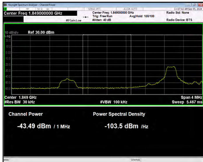
Band2 QPSK BW=5MHz Channel=18625 RB Size=1 Position=#Max Normal
