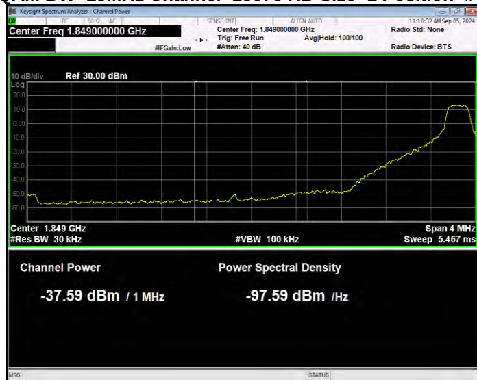
Band2 16QAM BW=15MHz Channel=18675 RB Size=1 Position=#0 Normal
