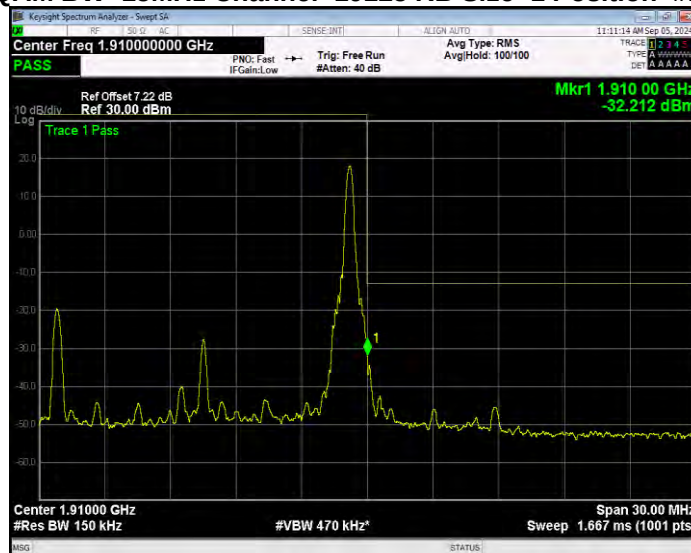
Band2 16QAM BW=15MHz Channel=19125 RB Size=27 Position=#0 Extended
