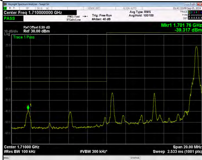
Band4 16QAM BW=10MHz Channel=20000 RB Size=27 Position=#0 Extended
