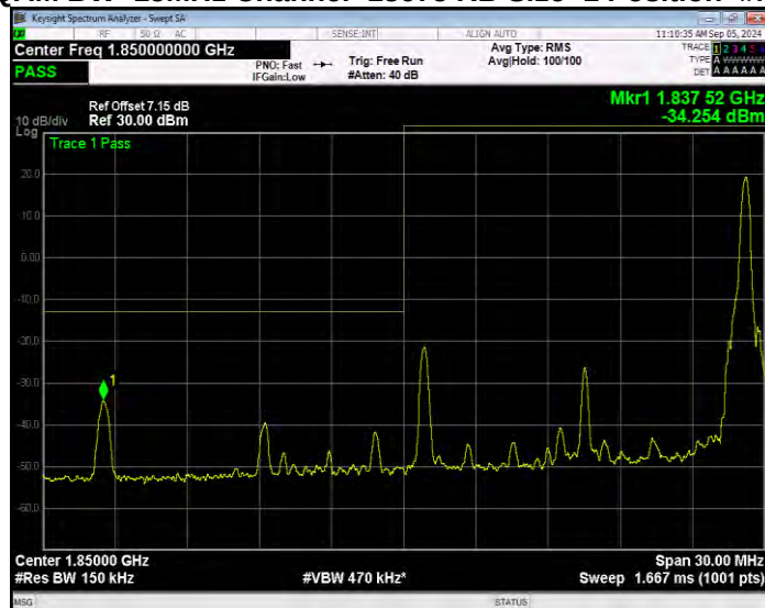
Band2 16QAM BW=15MHz Channel=18675 RB Size=27 Position=#0 Extended
