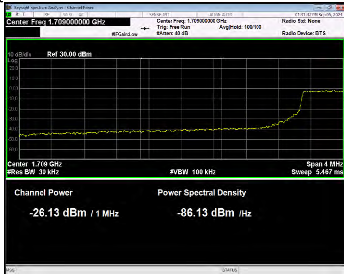
Band4 16QAM BW=10MHz Channel=20000 RB Size=27 Position=#0 Normal
