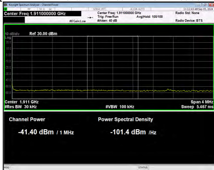
Band2 16QAM BW=20MHz Channel=19100 RB Size=27 Position=#0 Normal
