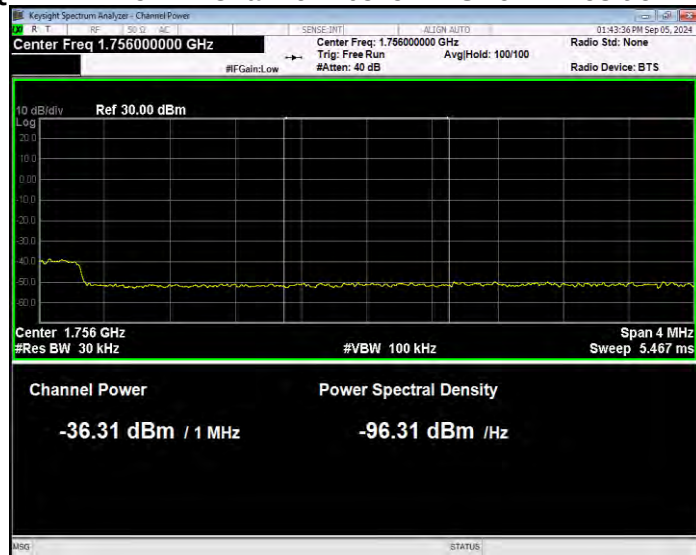
Band4 16QAM BW=15MHz Channel=20325 RB Size=27 Position=#0 Normal
