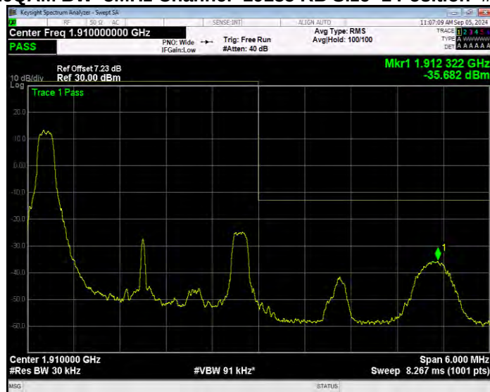
Band2 16QAM BW=3MHz Channel=19185 RB Size=1 Position=#Max Extended
