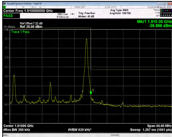
Band2 QPSK BW=20MHz Channel=19100 RB Size=100 Position=#0 Extended
