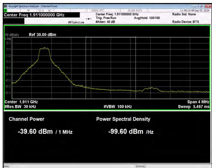
Band2 QPSK BW=5MHz Channel=19175 RB Size=1 Position=#Max Normal
