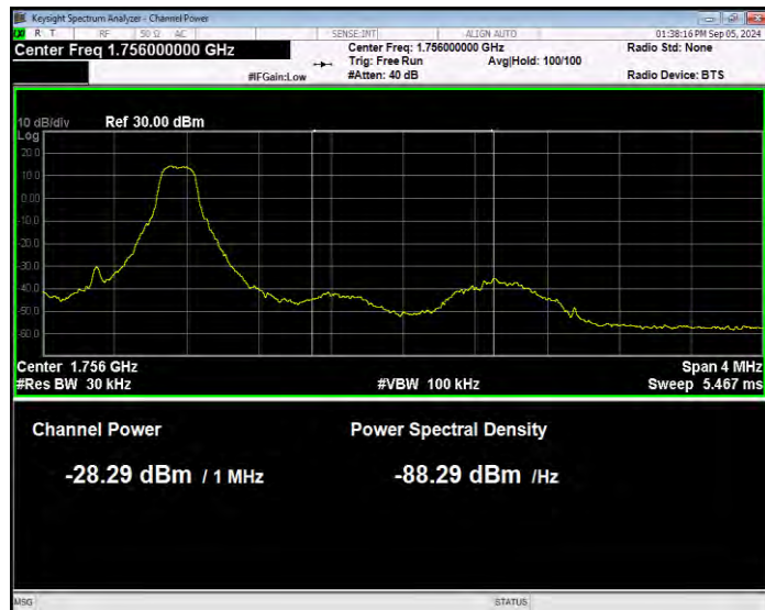
Band4 16QAM BW=1.4MHz Channel=20393 RB Size=1 Position=#Max Normal
