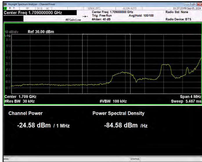
Band4 16QAM BW=1.4MHz Channel=19957 RB Size=1 Position=#Max Normal
