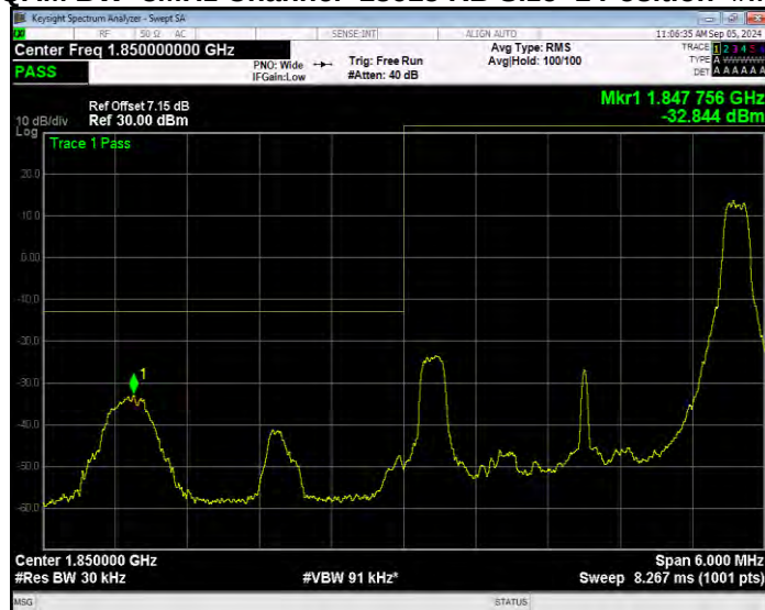
Band2 16QAM BW=3MHz Channel=18615 RB Size=15 Position=#0 Extended
