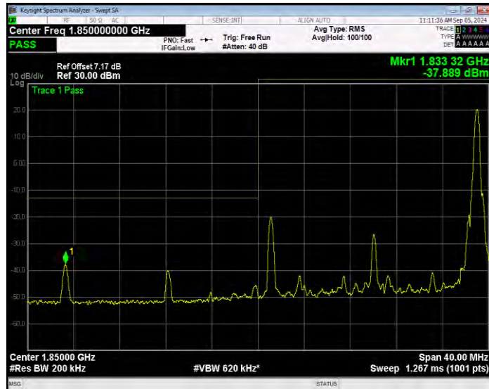
Band2 QPSK BW=20MHz Channel=18700 RB Size=100 Position=#0 Extended
