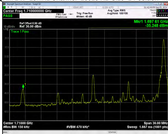
Band4 16QAM BW=15MHz Channel=20025 RB Size=27 Position=#0 Extended
