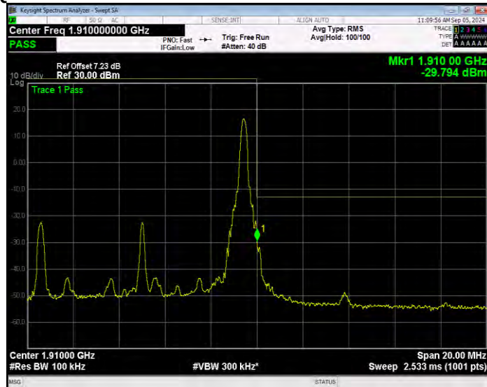
Band2 16QAM BW=10MHz Channel=19150 RB Size=27 Position=#0 Extended
