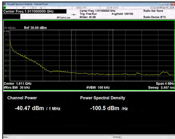
Band2 QPSK BW=20MHz Channel=19100 RB Size=1 Position=#Max Normal
