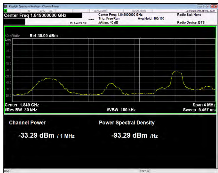
Band2 QPSK BW=3MHz Channel=18615 RB Size=1 Position=#Max Normal
