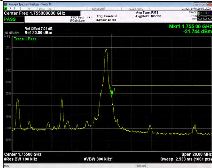
Band4 16QAM BW=10MHz Channel=20350 RB Size=27 Position=#0 Extended
