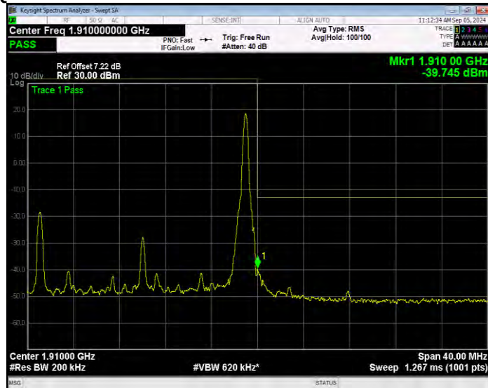
Band2 16QAM BW=20MHz Channel=19100 RB Size=27 Position=#0 Extended
