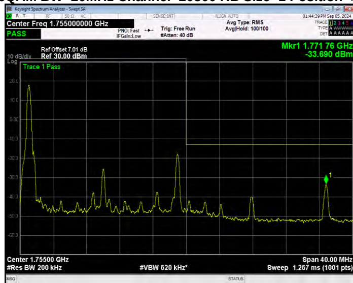
Band4 16QAM BW=20MHz Channel=20300 RB Size=1 Position=#Max Extended
