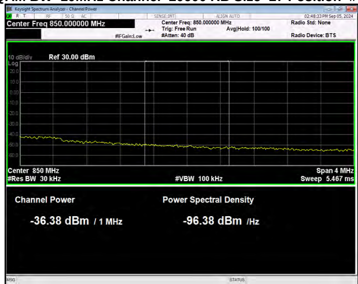
Band5 16QAM BW=10MHz Channel=20600 RB Size=27 Position=#0 Normal
