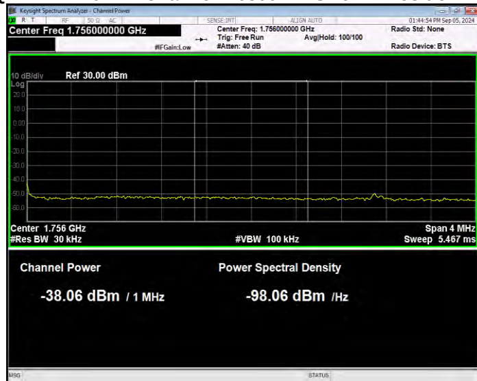
Band4 16QAM BW=20MHz Channel=20300 RB Size=27 Position=#0 Normal
