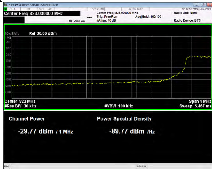
Band5 16QAM BW=10MHz Channel=20450 RB Size=27 Position=#0 Normal
