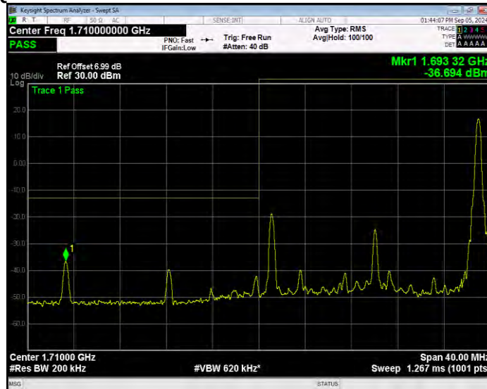
Band4 16QAM BW=20MHz Channel=20050 RB Size=27 Position=#0 Extended
