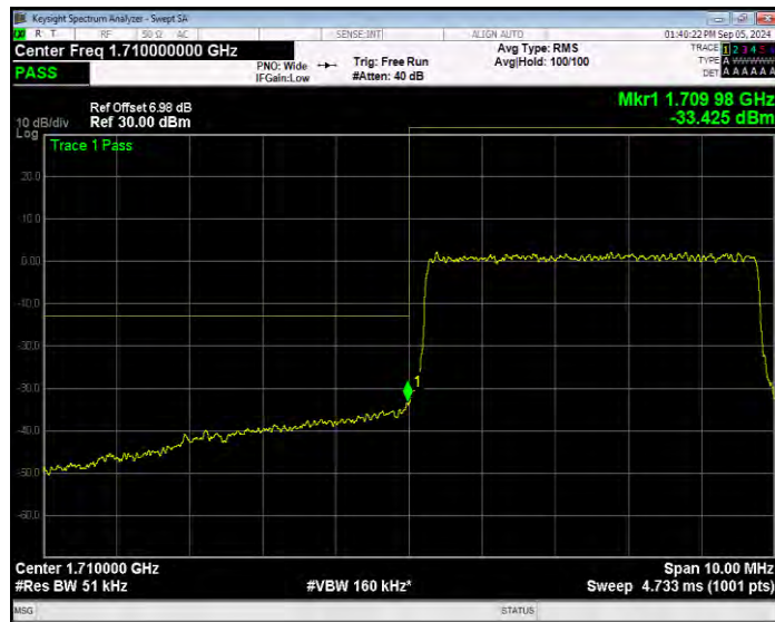
Band4 16QAM BW=5MHz Channel=20375 RB Size=1 Position=#0 Extended
