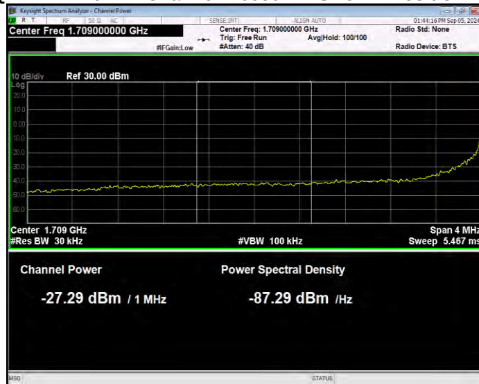
Band4 16QAM BW=20MHz Channel=20050 RB Size=27 Position=#0 Normal
