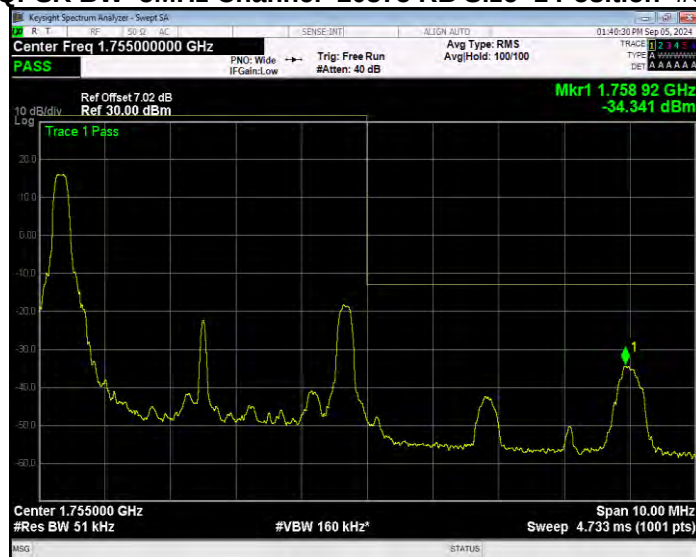
Band4 QPSK BW=5MHz Channel=20375 RB Size=1 Position=#Max Extended
