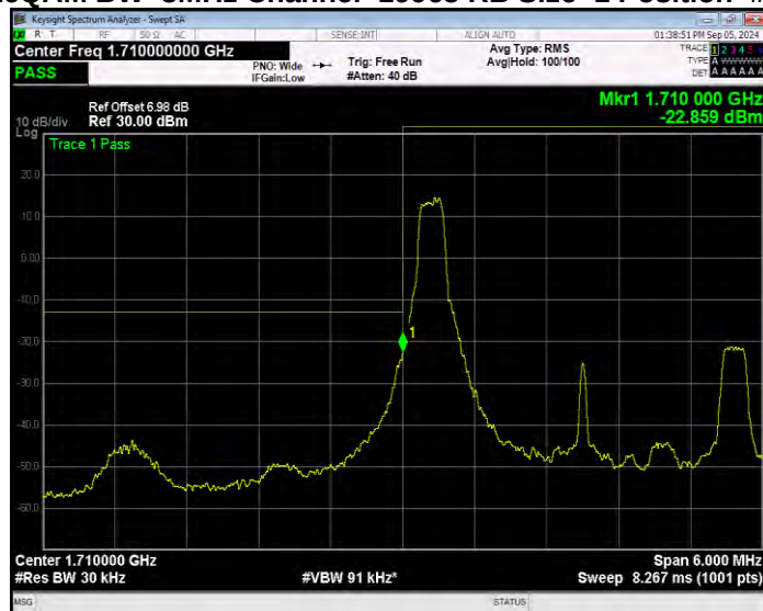
Band4 16QAM BW=3MHz Channel=19965 RB Size=1 Position=#Max Extended
