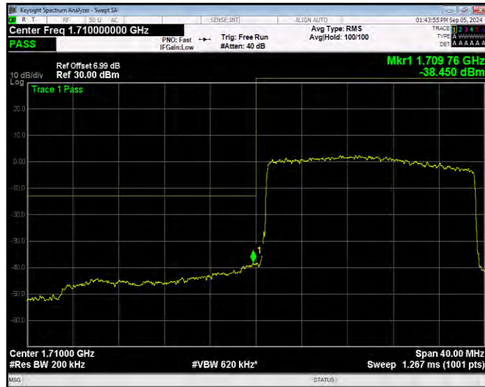
Band4 QPSK BW=20MHz Channel=20300 RB Size=1 Position=#0 Extended
