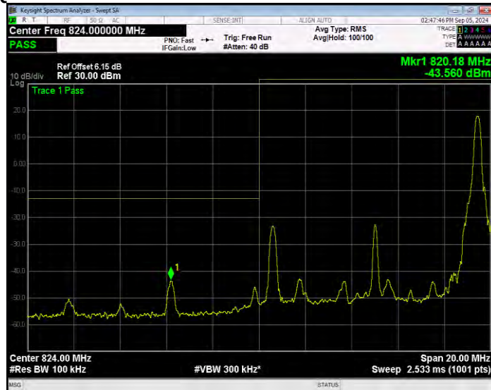
Band5 16QAM BW=10MHz Channel=20450 RB Size=27 Position=#0 Extended
