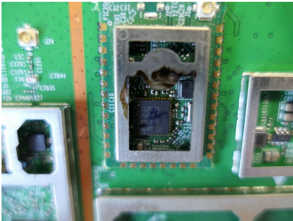
(25) EUT Photo
