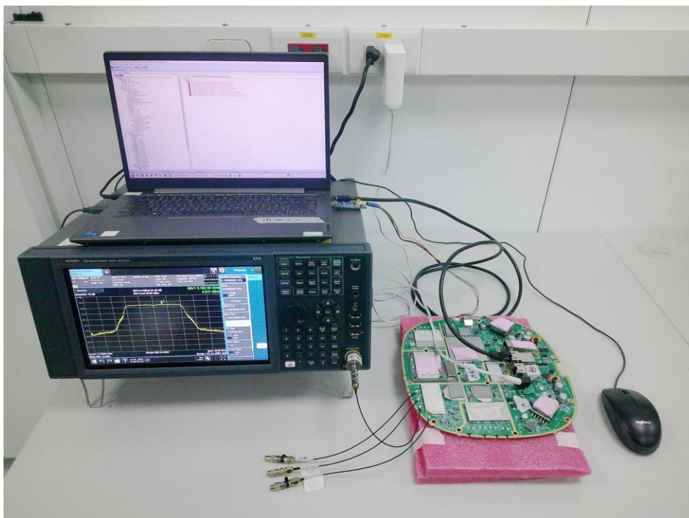
Description: Conducted Measurement Test Setup - WiFi
