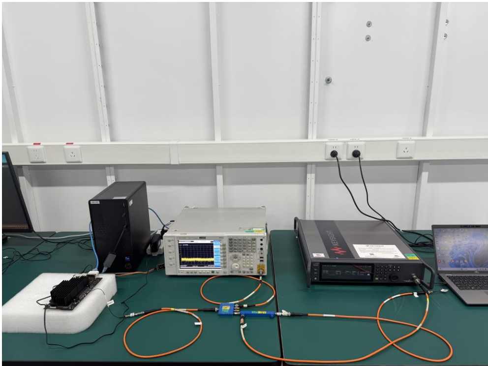
Description: Contention Based Protocol Measurement Test Setup for AP Mode
